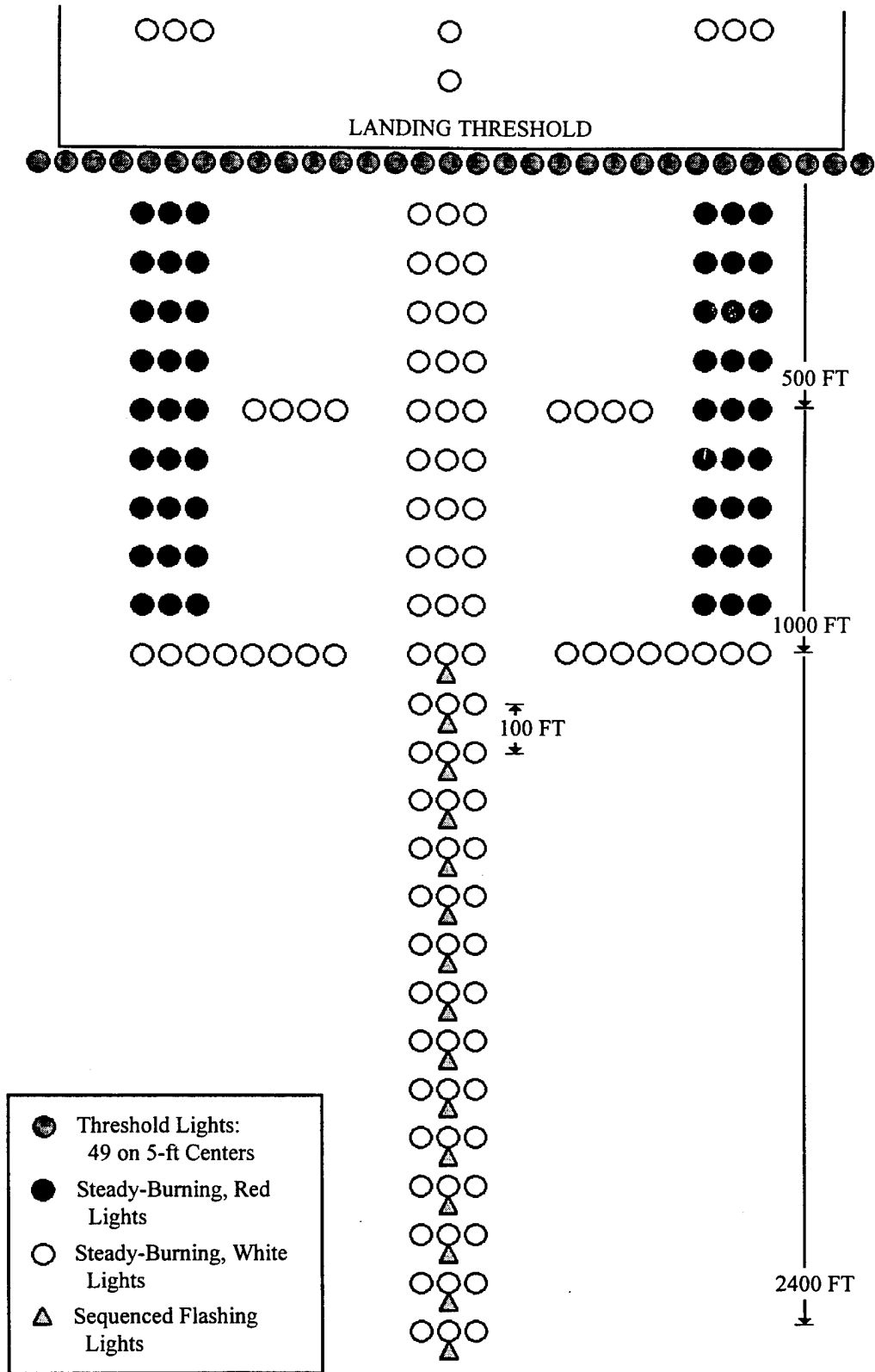
FIGURE 6. REDUCED-DENSITY ALSF-2 SYSTEM (CONFIGURATION H)
