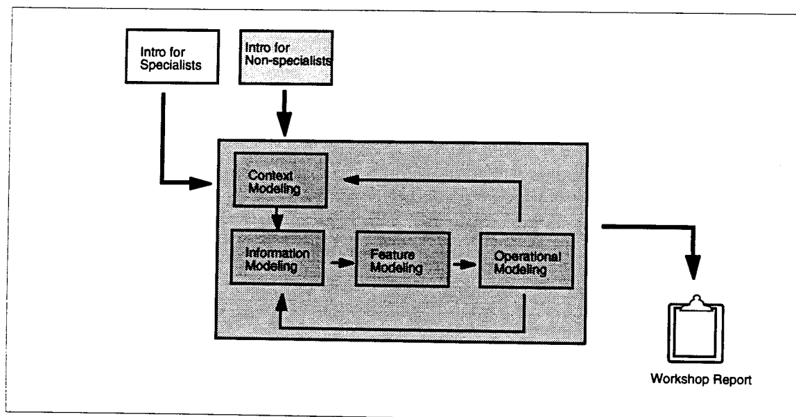
Figure 7: Model Iteration
