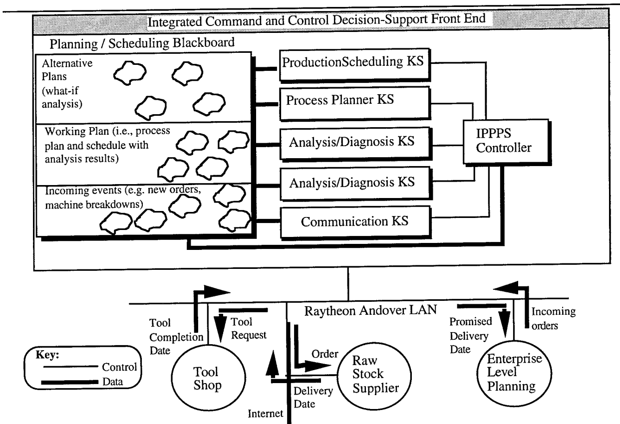
Figure 1: The IP3S Blackboard Architecture
