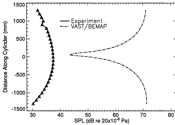
Figure 34: Test L2 Vertical Directivity Pattern at 273.59 Hz
