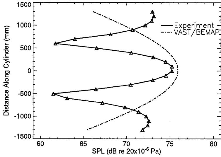
Figure 39: Test L3 Vertical Directivity Pattern at 473.66 Hz
