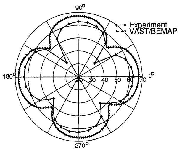
Figure 17: Test 04 Directivity Pattern at 200 Hz
