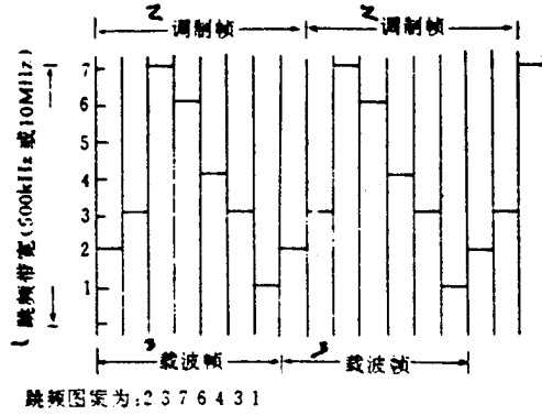
Fig. 7. TATS frequency hopping schematic
