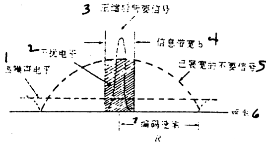
Fig. 4. Correlated spectrum
