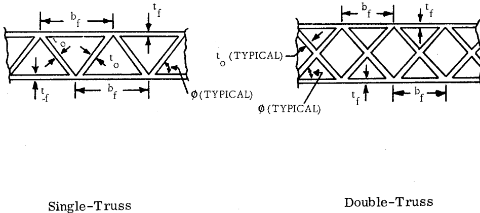
Figure 2.1-4. Corrugation Configurations
