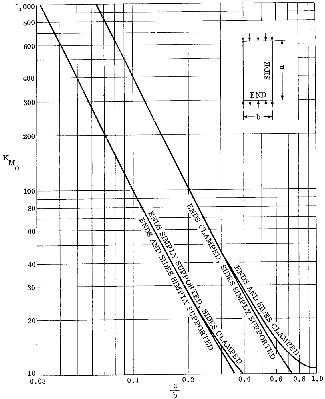
Figure 3.1-16. K_{M_0} for Sandwich Panel with Isotropic Facings in Edgewise Compression
