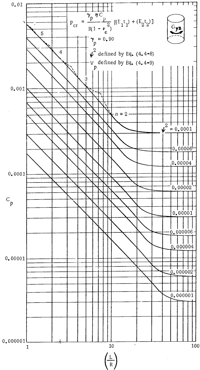
Figure 4.4-3. Buckling Coefficients C_p for Circular Sandwich Cylinders Subjected to External Lateral Pressure; Isotropic Facings; Transverse Shear Properties of Core Isotropic or Orthotropic; V_p = 0
