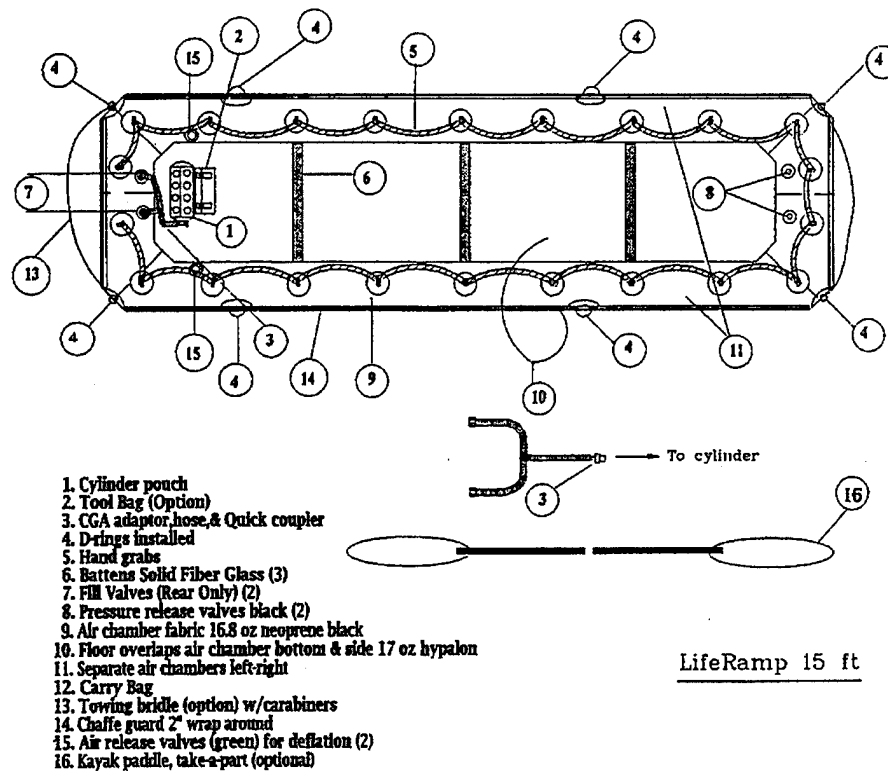
FIGURE 9. SCHEMATIC OF 15-FOOT LIFE-RAMP®
