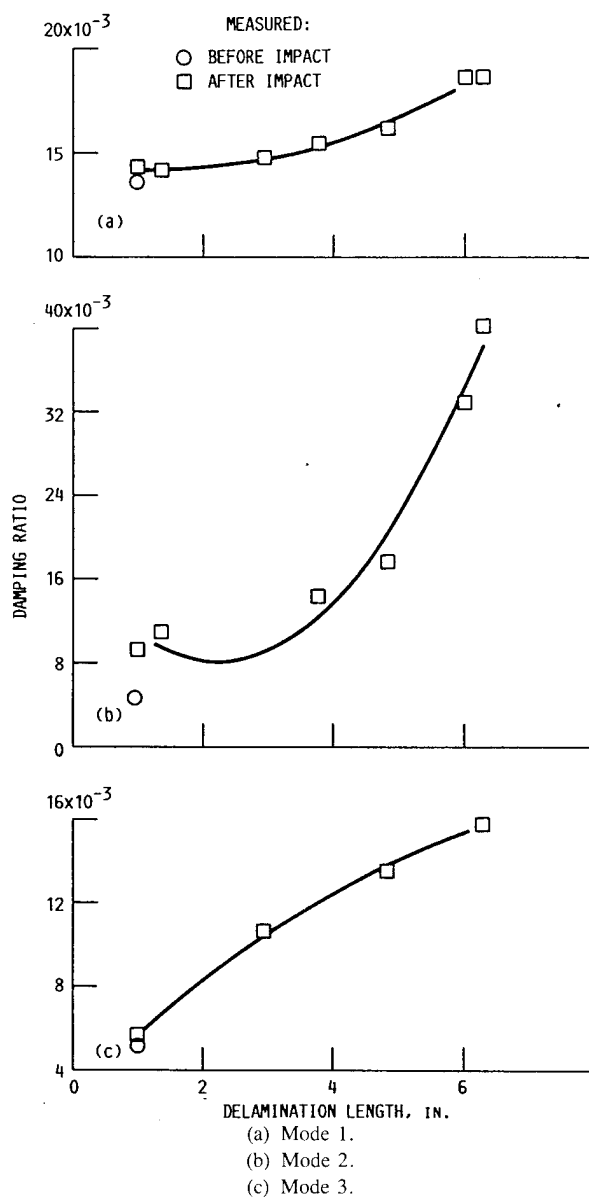
Figure 9.—Effect of delamination on damping ratios.
