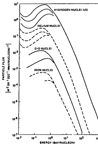
Fig. 7. Cosmic Ray Energy Spectra.
