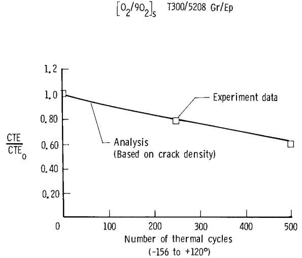
EFFECT OF THERMAL CYCLING ON THE COEFFICIENT OF THERMAL EXPANSION
