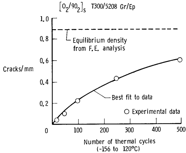
EFFECT OF THERMAL CYCLING ON MICROCRACK DENSITY
