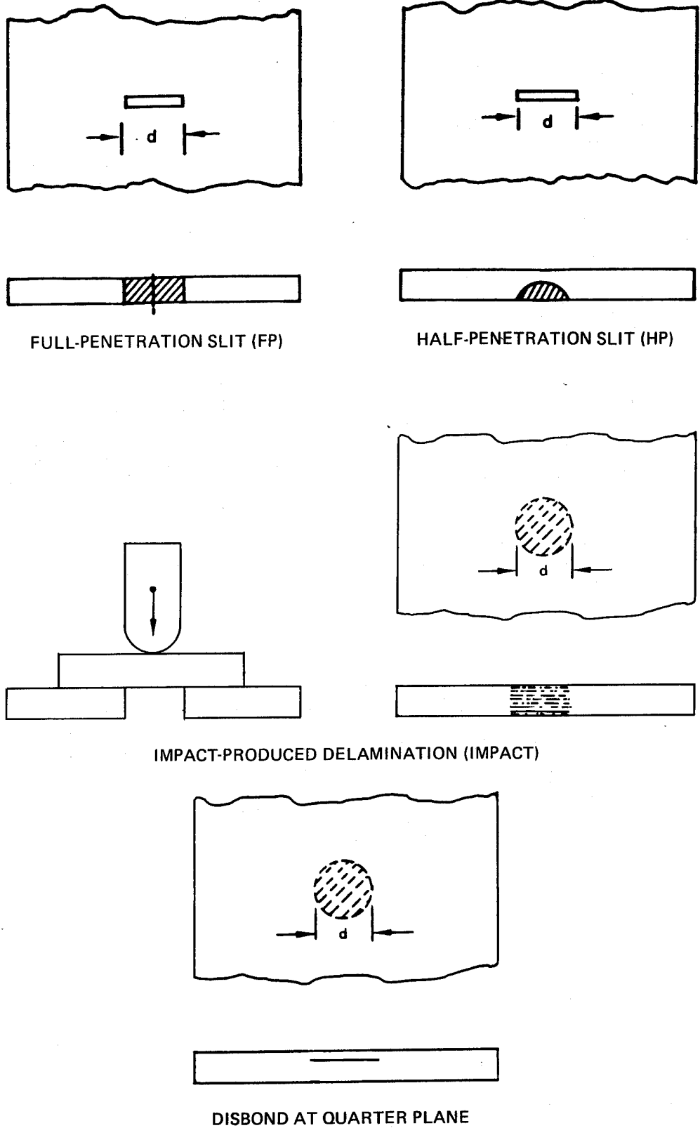
Figure 5. Stress Concentration Configurations Tested
