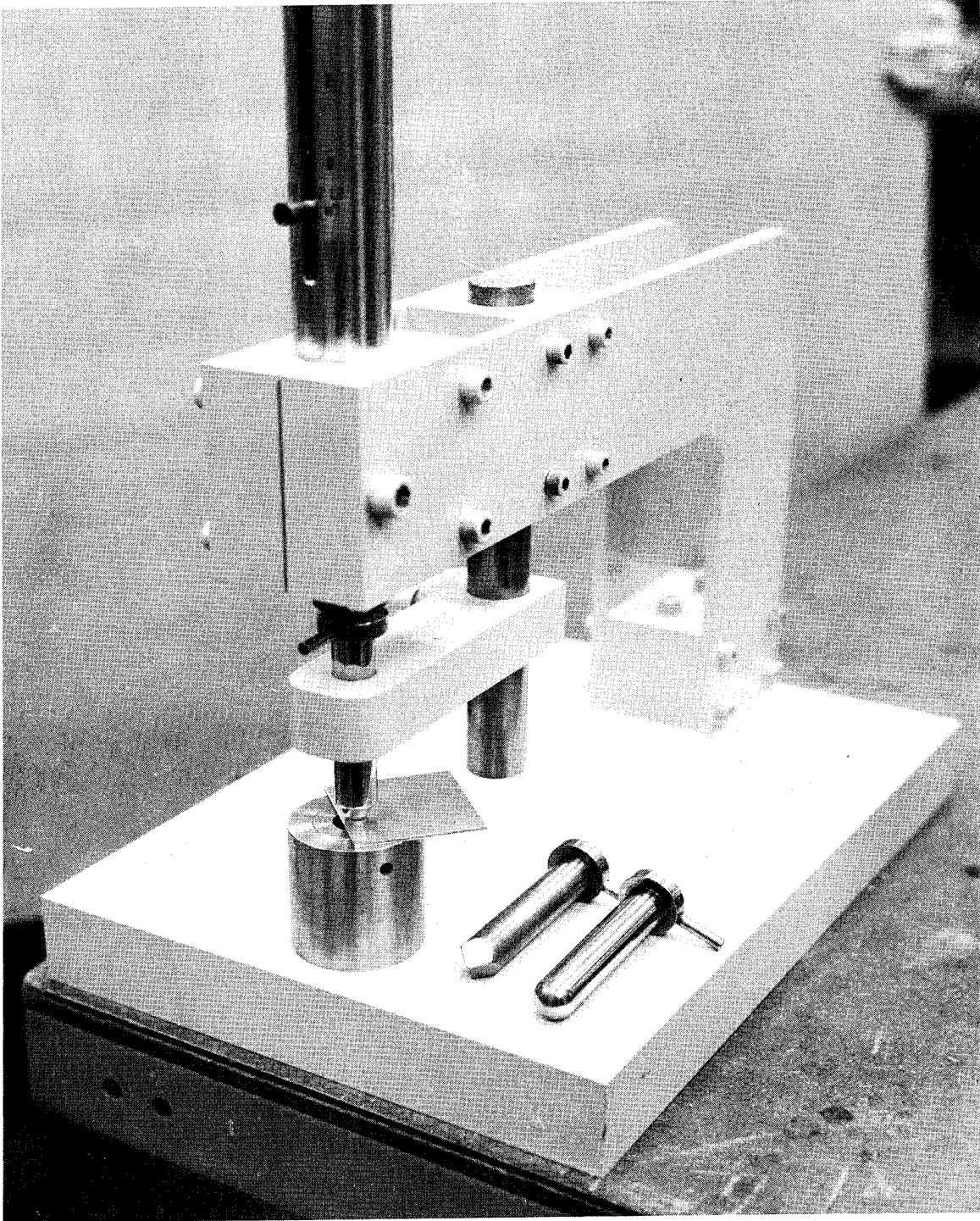
Figure 7. Impact Test Machine
