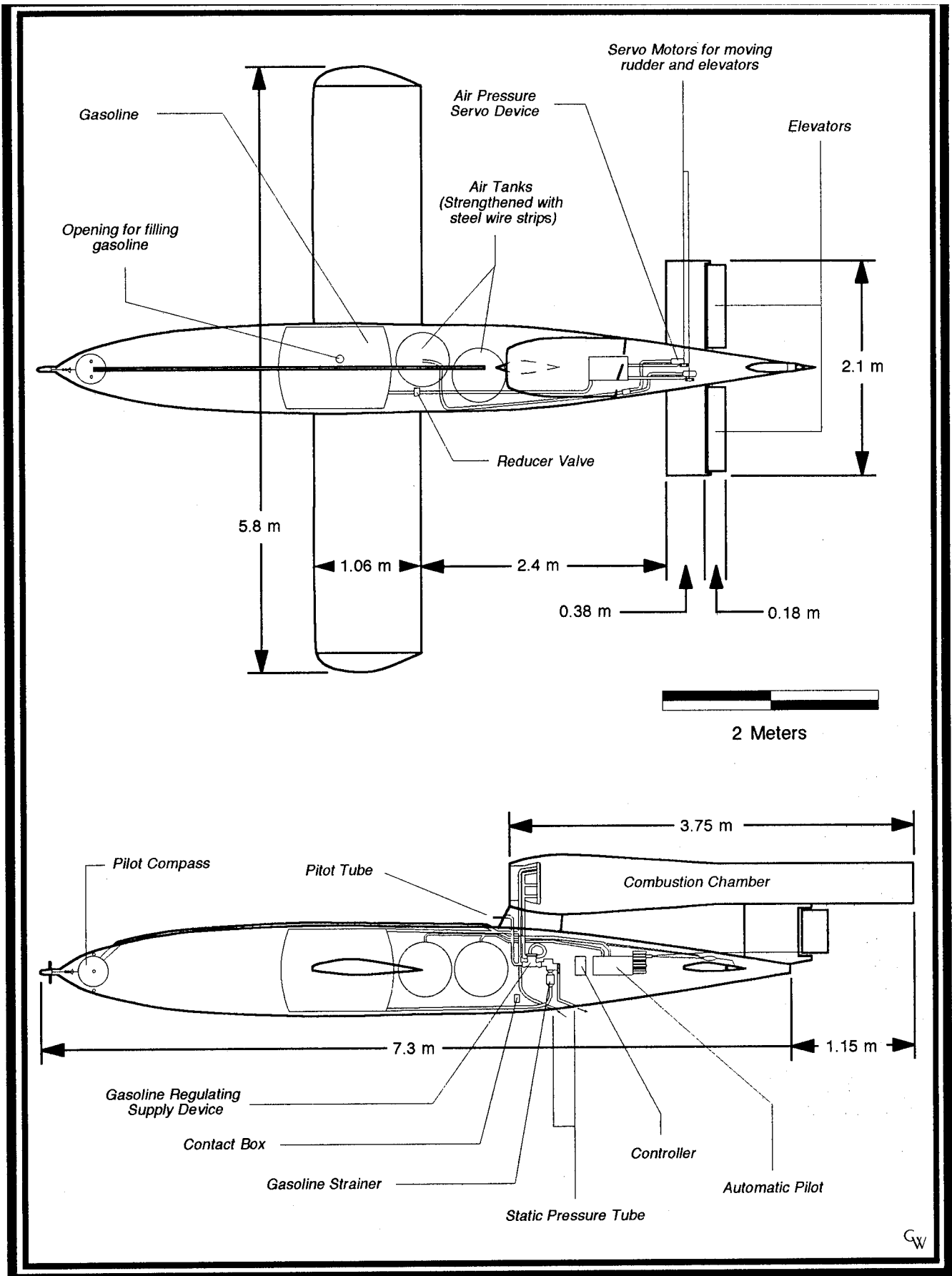
Figure 20. V-1 schematic drawing.
