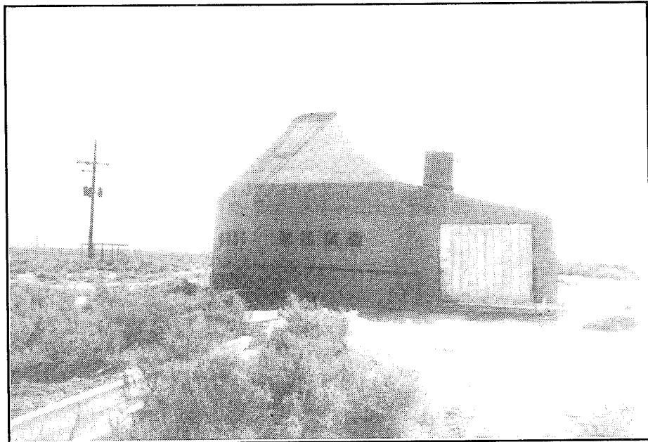
Figure 33. Aerobee observation shelter, west elevation (Allred/Space Center 1994).
