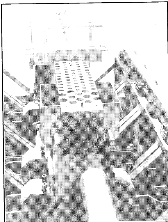
Figure 80. Water brake No. 1, the primary hydraulic brake at the 120 foot point of the track, ca. 1959 (Space Center archives).
