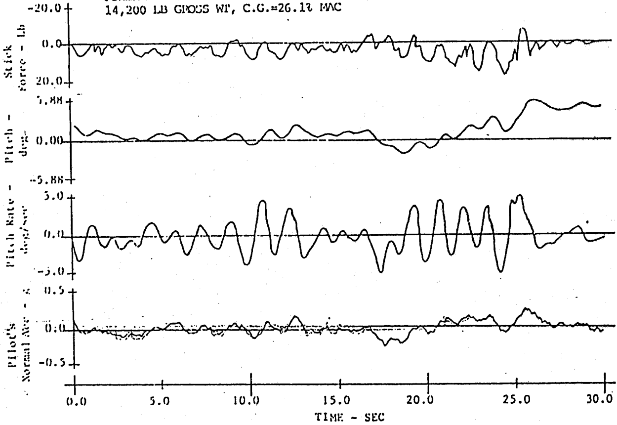
Figure 35. Selected Parameter Time Histories, Configuration 2-8
