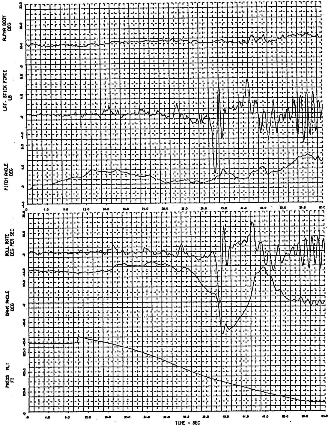
Figure E-43a. Flight Characteristics - Time History
