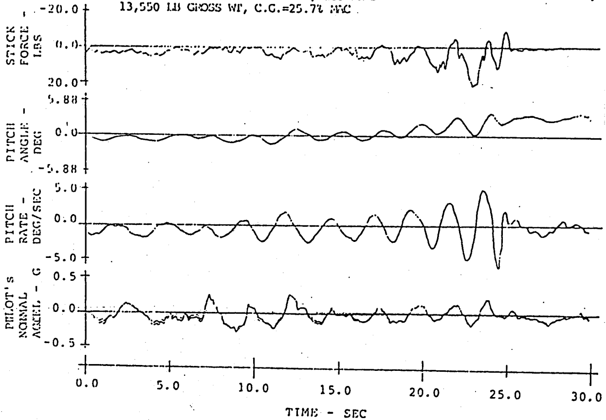
Figure 47. Selected Parameter Time Histories, Configuration 5-10
