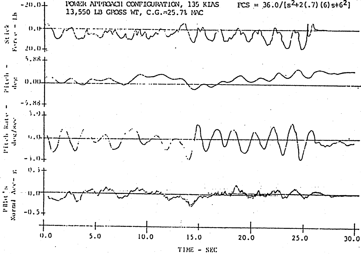
Figure 56. Selected Parameter Time Histories, Configuration 5-9
