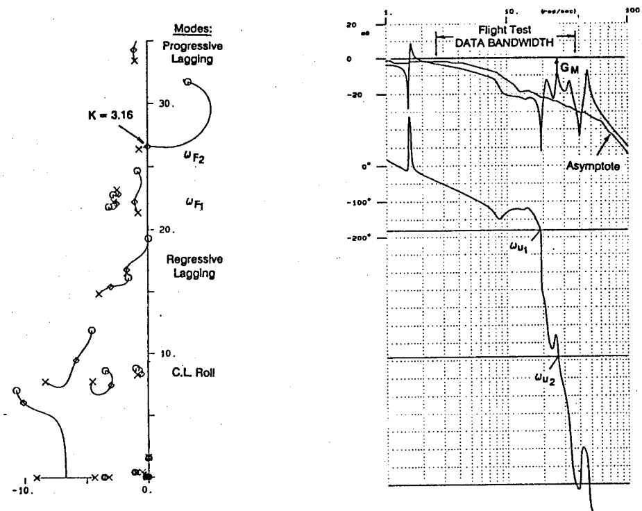
Figure 40. Large Helicopter q/\delta_B Response with All SAS Loops Closed
