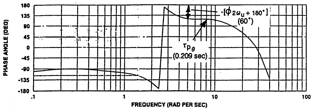
PITCH ANGLE TO CONTROLLER PHASE ANGLE VS FREQUENCY
