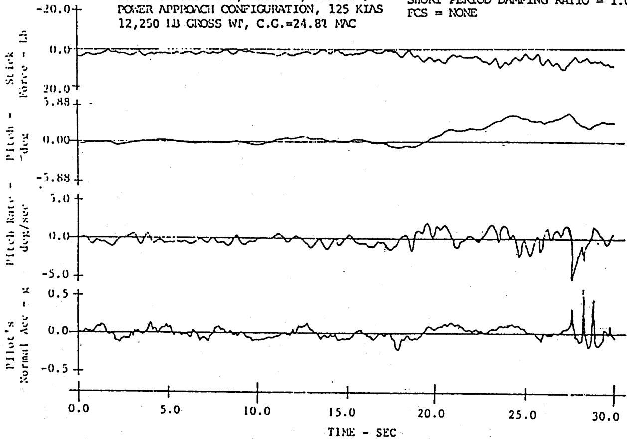
Figure 37. Selected Parameter Time Histories, Configuration 3-1
