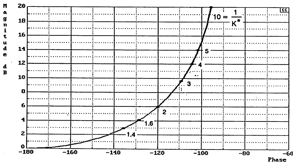
Figure 24. Sinusoidal Input/Triangle Output Inverse Describing Function
