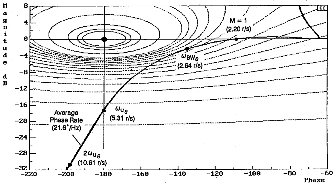
Figure B-10. X-15 Flight 1-1-5
