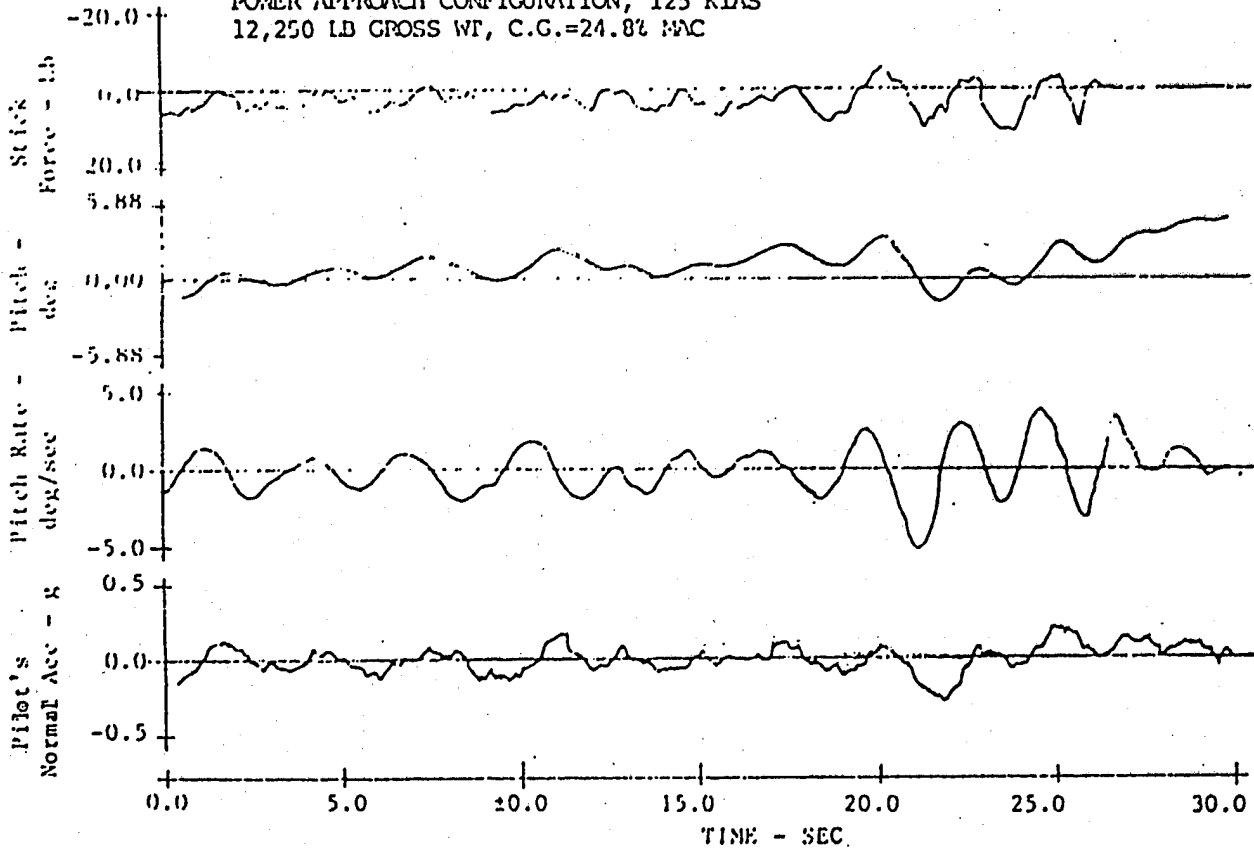
Figure 33. Selected Parameter Time Histories, Configuration 2-5
