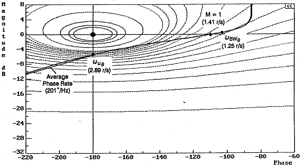
Figure B-6. Have PIO Configuration 3-13
