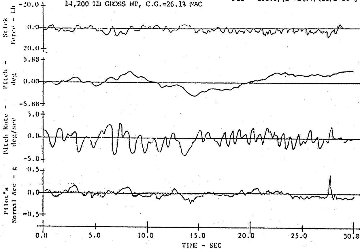
Figure 19. Selected Parameter Time Histories, Configuration 3-6
