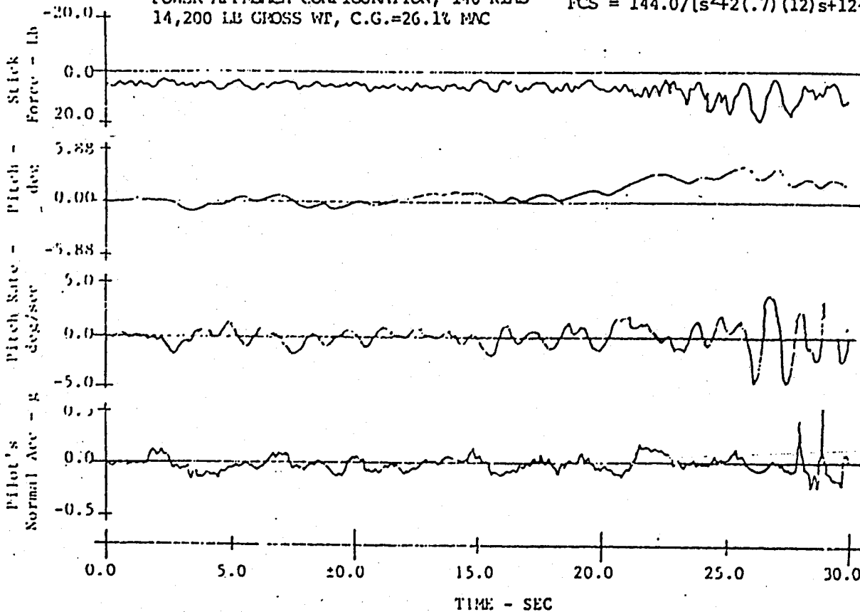
Figure 34. Selected Parameter Time Histories, Configuration 2-7
