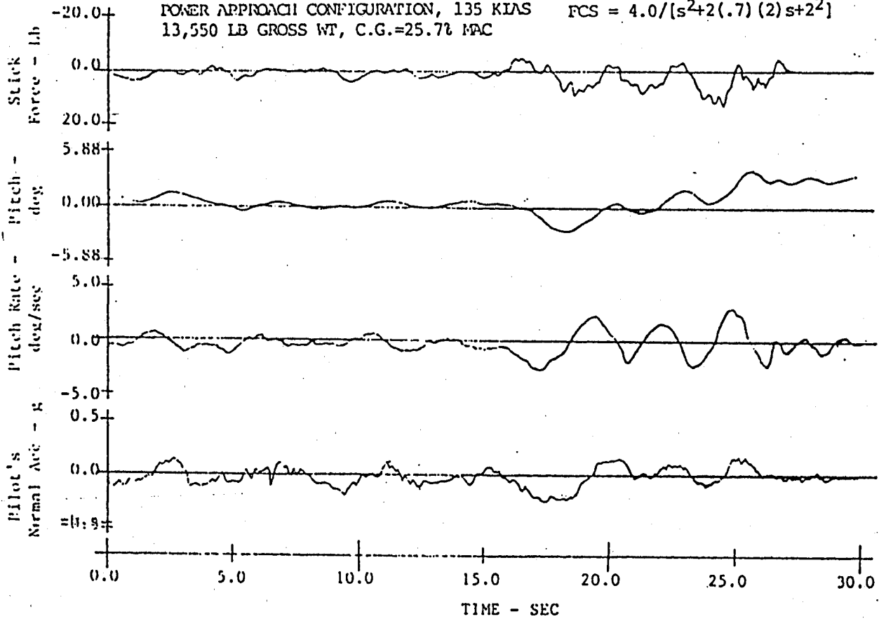
Figure 41. Selected Parameter Time Histories, Configuration 3-12
