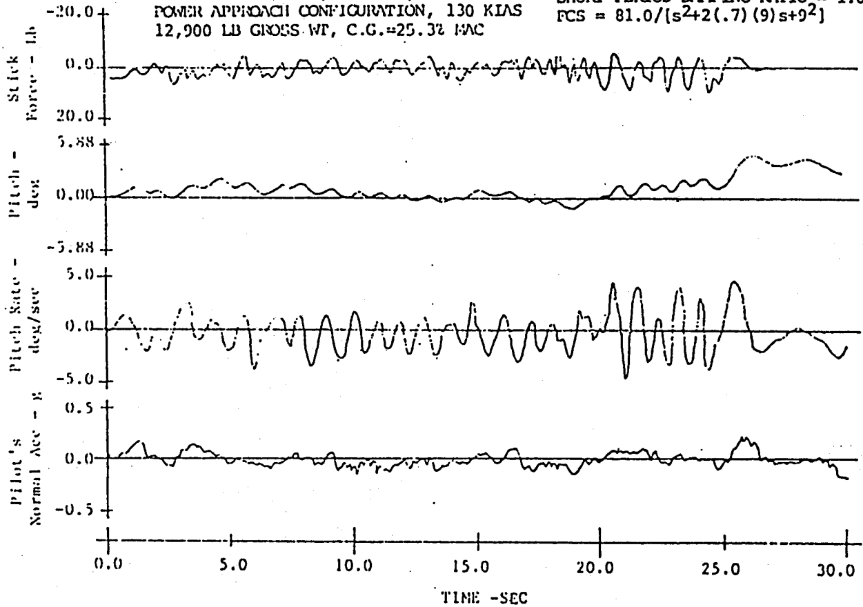
Figure 40. Selected Parameter Time Histories, Configuration 3-8
