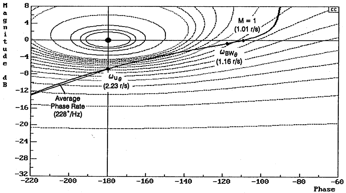
Figure B-5. Have PIO Configuration 3-12
