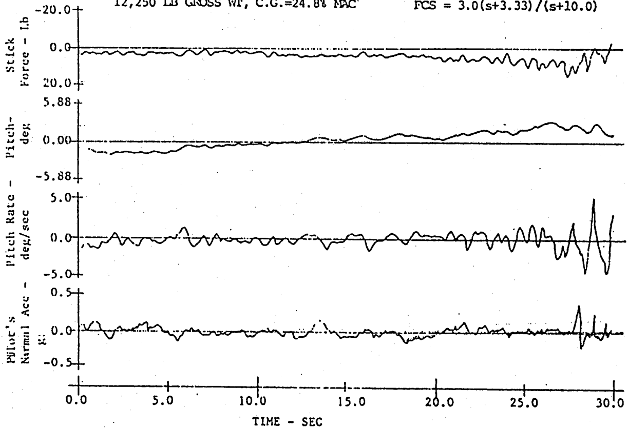
Figure 31. Selected Parameter Time Histories, Configuration 2-B
