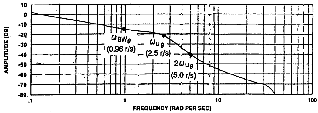
PITCH ANGLE TO CONTROLLER AMPLITUDE VS FREQUENCY
