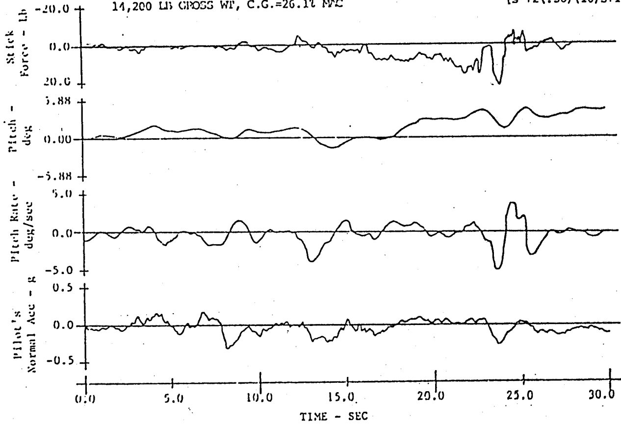
Figure 48. Selected Parameter Time Histories, Configuration 5-11
