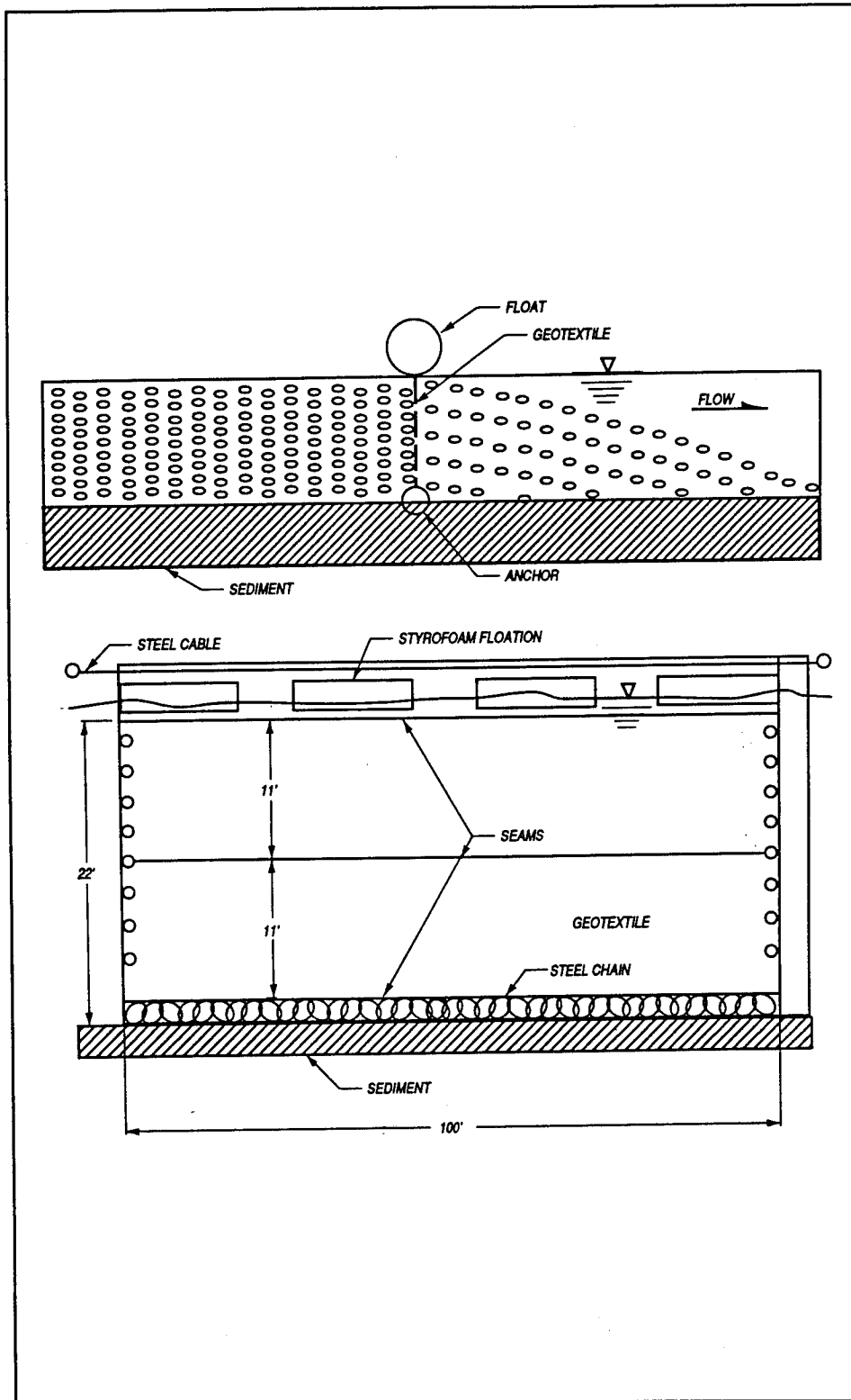
Figure 7. Sediment dispersion barrier
