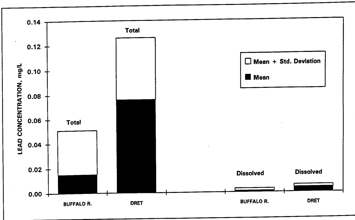
Figure 28. Lead concentrations in Buffalo River water column during dredging compared to dredging elutriate test
