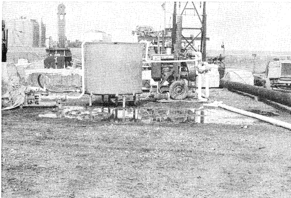
Figure M2. Small polymer pump on left beside concentrate tank, large diesel-powered pump on right
