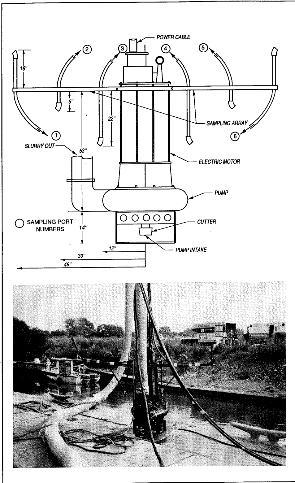
Figure 6. Submersible pump
