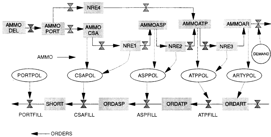
Figure D-1. DYNAMO Flow Diagram: Ammunition and Order Flows Within Theater
