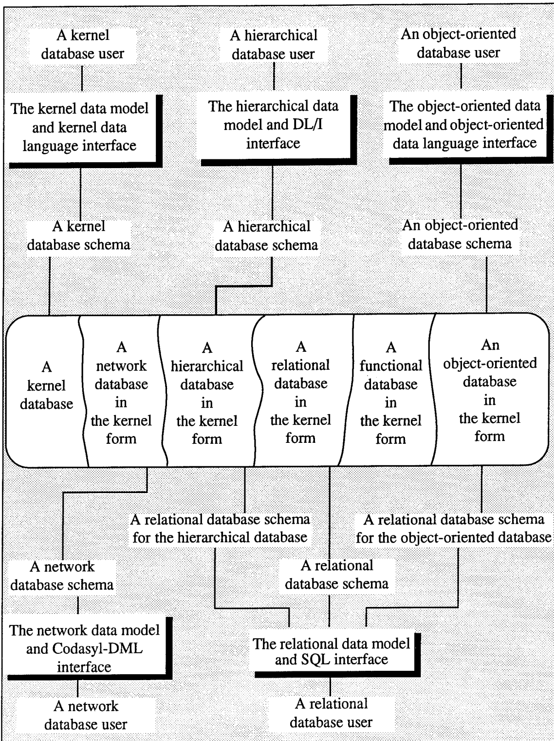
Figure 1: Interfaces, Databases and Schemas in M 3 DBMS with CMAC
