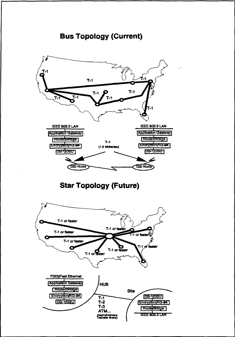
Figure 11. DSI network topology
