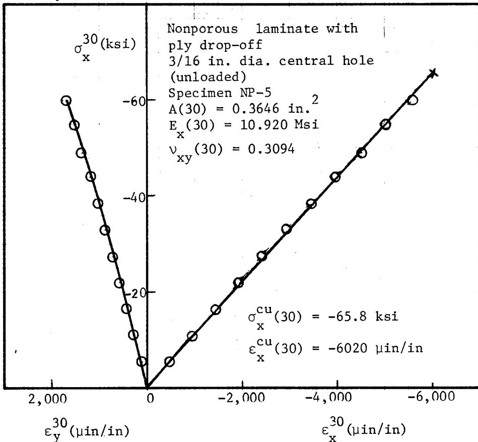
Figure C6. Stress-Strain Curves for the 28- and 30-ply Sections of Specimen NP-5.
