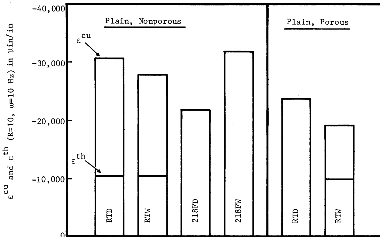
Figure 3. Compression Data on [\pm 45]_{6S} Specimens.
