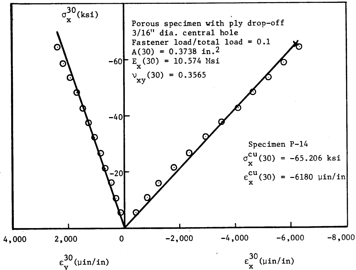
Figure C10. Stress-Strain Curves for the 28- and 30-ply Sections of Specimen P-14.
