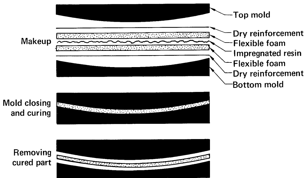
Figure 8. Schematic of elastic reservoir molding.
