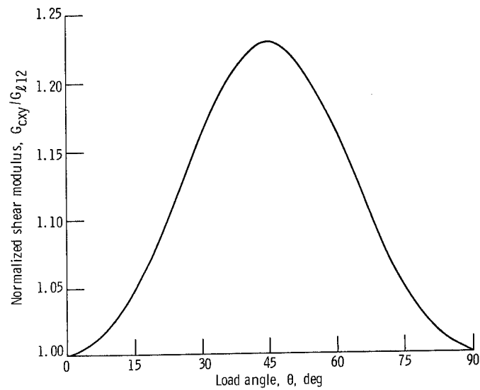
Figure 4. - Variation of shear modulus with load direction.
