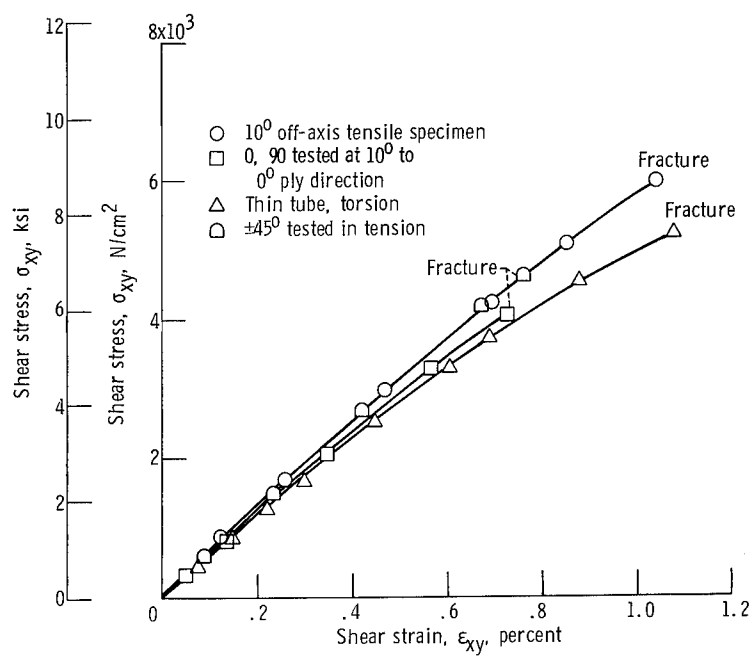
Figure 17. - Comparison of shear stress-strain curves.
