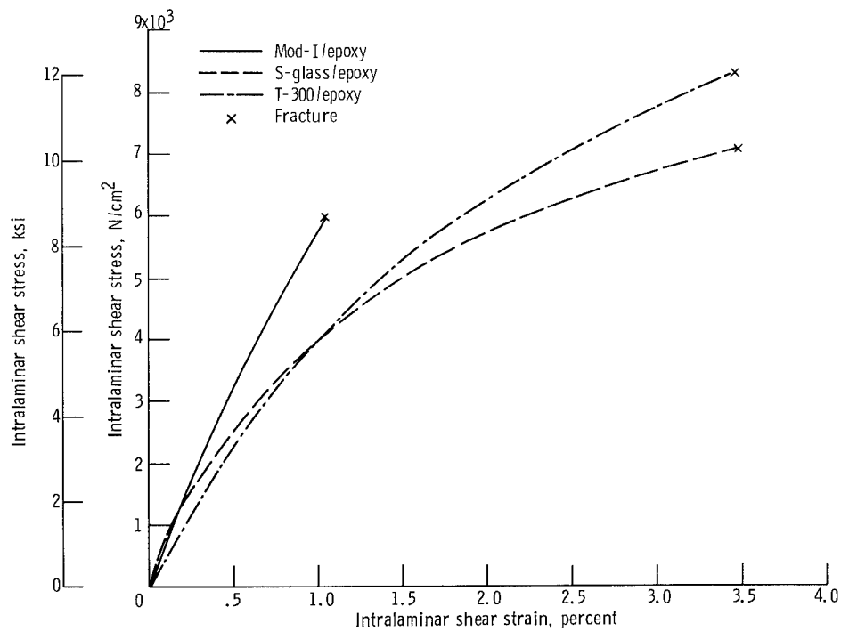
Figure 15. - Intralaminar shear stress-strain diagrams for three materials.
