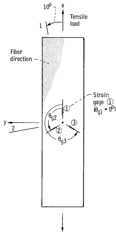
Figure 5. - Schematic depicting 10^\circ off-axis tensile test specimen with strain gage positions ( x, y - structural axes; 1, 2 - material axes).
