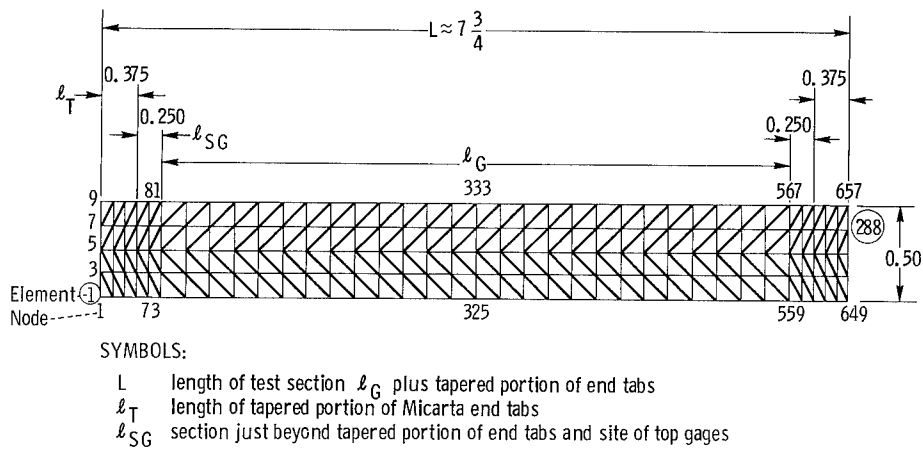
Figure 6. - Grid for finite element analysis of Mod-I/epoxy specimens. (Top gages located at nodes 74 and 77; midpoint gages located at nodes 326, 329, and 332. All dimensions shown are relative.)
