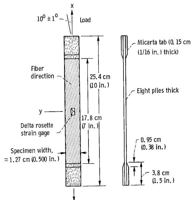
Figure 19. - Schematic showing geometry and instrumentation of proposed 10^0 off-axis tensile specimen for fiber composite intralaminar shear characterization.
