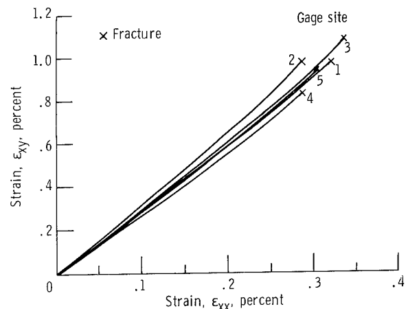
Figure 12. - Shear strain curves at various gage sites (fig. 8) for 10^\circ off-axis tensile specimen (Mod-I/epoxy fiber composite).
