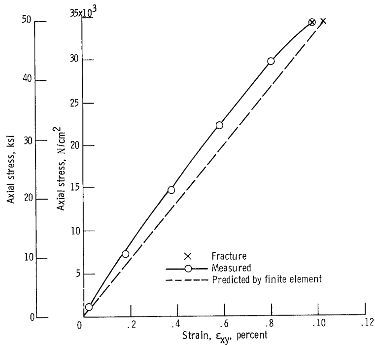
Figure 18. - Comparison of measured and predicted structural axes shear strains at center point of 10^0 off-axis tensile specimen (Mod-I/epoxy fiber composite).
