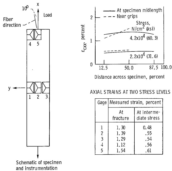
Figure 14. - Axial strain variation measured across specimen of S-glass/epoxy unidirectional composite [0]_8 loaded to fracture at 10^\circ from fiber direction.
