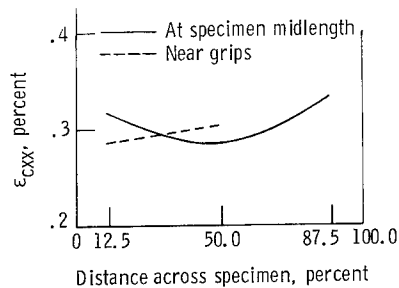
AXIAL STRAINS AT FRACTURE
