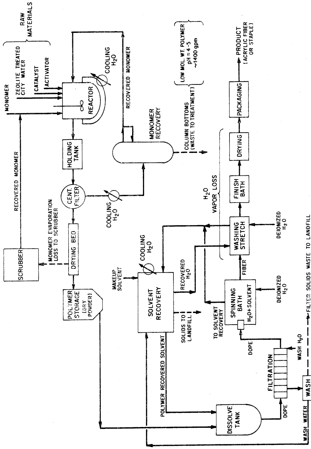
ACRYLIC FIBER PRODUCTION - WET SPINNING PROCESS FIGURE 27
