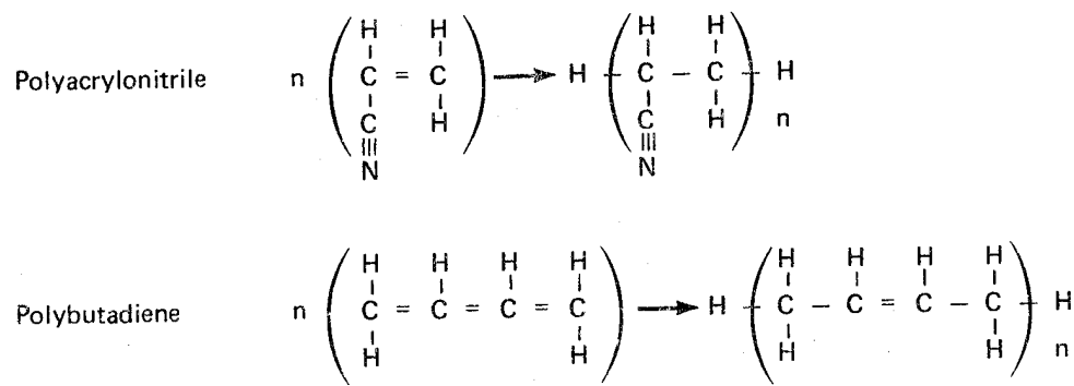
FIGURE 2 TYPICAL POLYMERIZATION REACTIONS FOR POLYACRYLONITRILE AND POLYBUTADIENE
