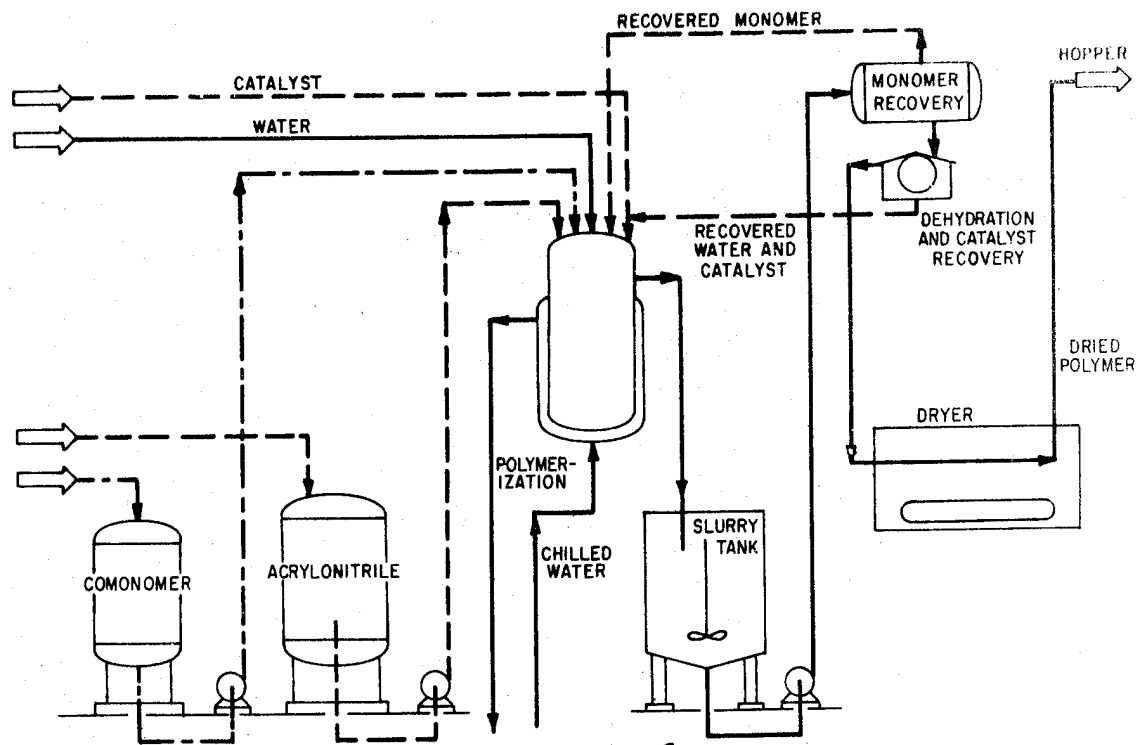
AQUEOUS - SUSPENSION ACRYLONITRILE POLYMERIZATION
