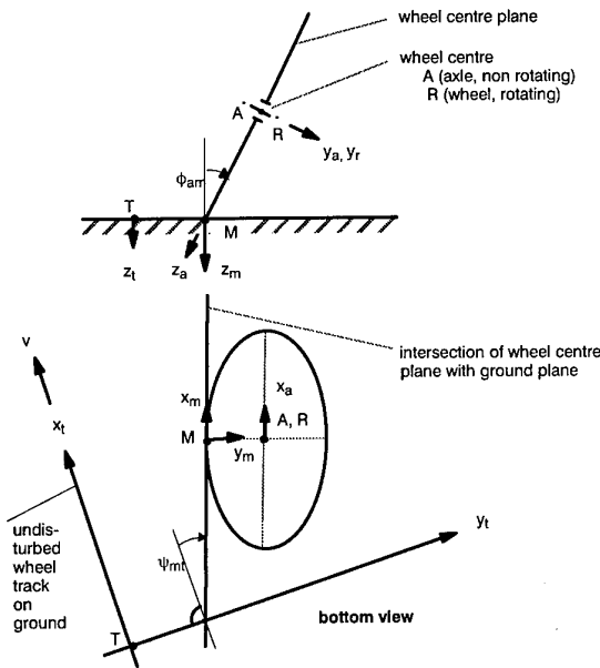
Fig. 3-1 WHEEL COORDINATES
