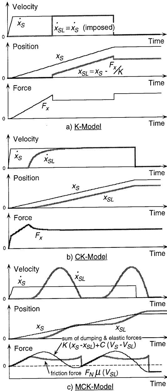
Fig. 5.1-3 Bristle responses
