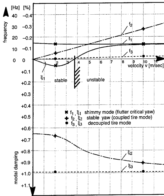
Fig. 5.2-2 EIGENFREQUENCIES AND MODAL DAMPINGS
