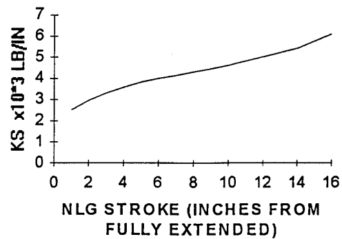
KS LATERAL SPRING RATE
