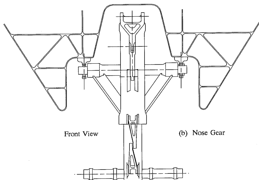
Figure 4. Landing Gear Arrangement.
