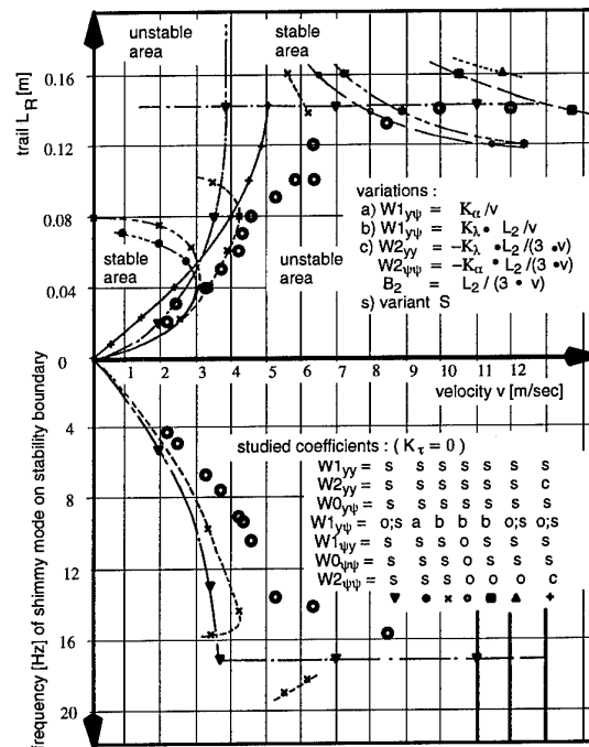
Fig. 5.2-5 INFLUENCE OF \gamma AND \psi COEFFICIENTS single wheel ● test results - - - d_s = 0.6 \text{ Nm/(rad/sec)}
