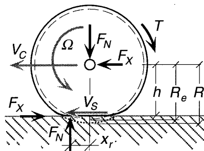
Fig. 4-1 Classical model
