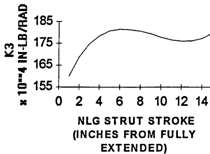
K3 TORSIONAL STIFFNESS
