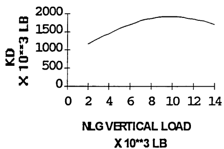
KD TIRE LATERAL SPRING RATE
