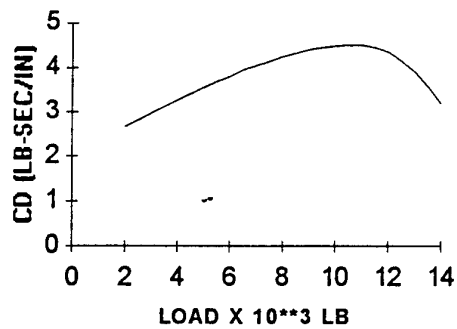
CD - TIRE LATERAL DAMPING
