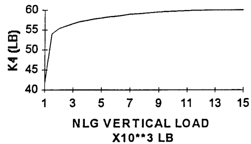
K4 CROSS COUPLED SPRING RATE
