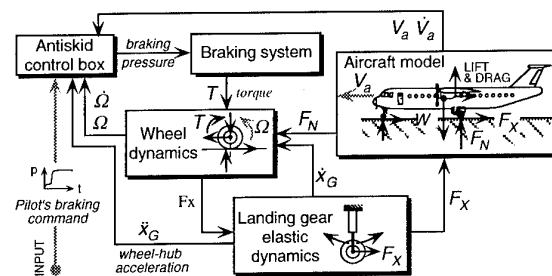
Fig. 3-1 Antiskid-landing gear-aircraft system
