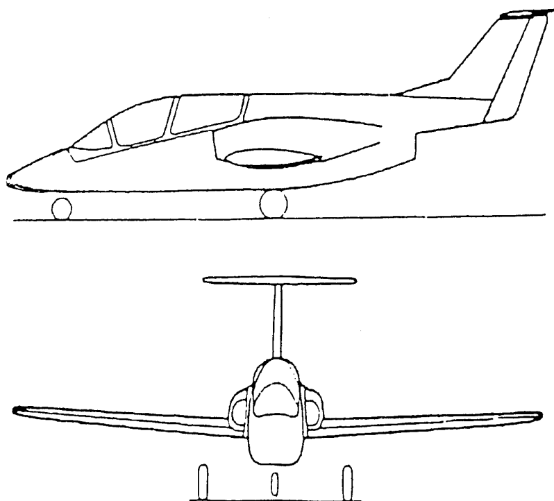
Fig. 2-1 Advanced Training Aircraft
