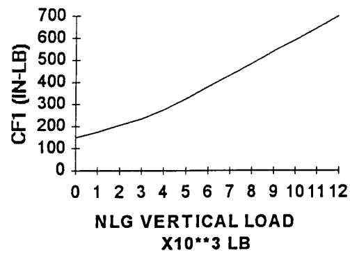
CF1 FRICTIONAL TORQUE
