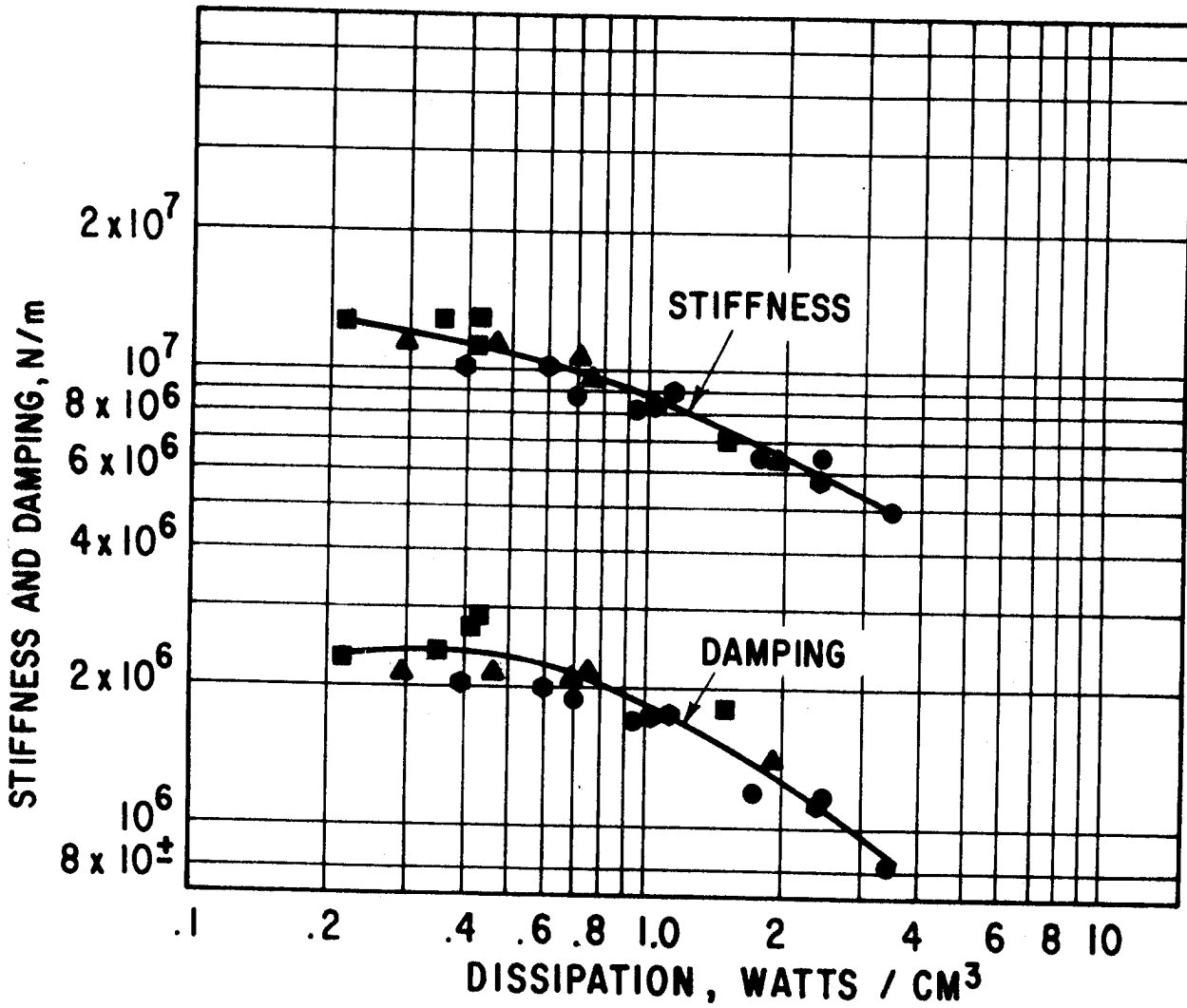
Fig. 11▲ Stiffness and Damping as a Function of Dissipation. Compression Specimen. 32 C (Ten Elements)
