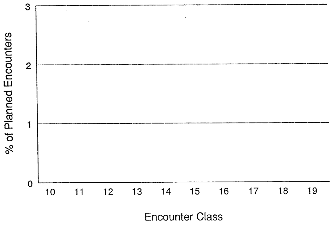
Figure 5-3. Unresolved NMACs.
