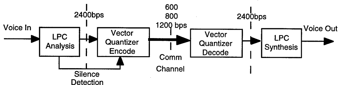
Fig. 3 — Vector quantization of LPC parameters
