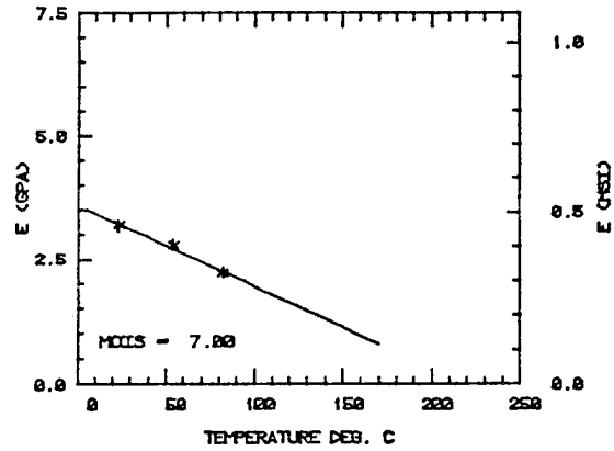
d) Fibredux 914
