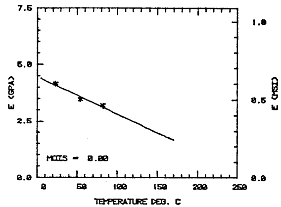
d) Fibredux 914
