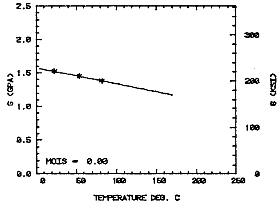
d) Fibredux 914
