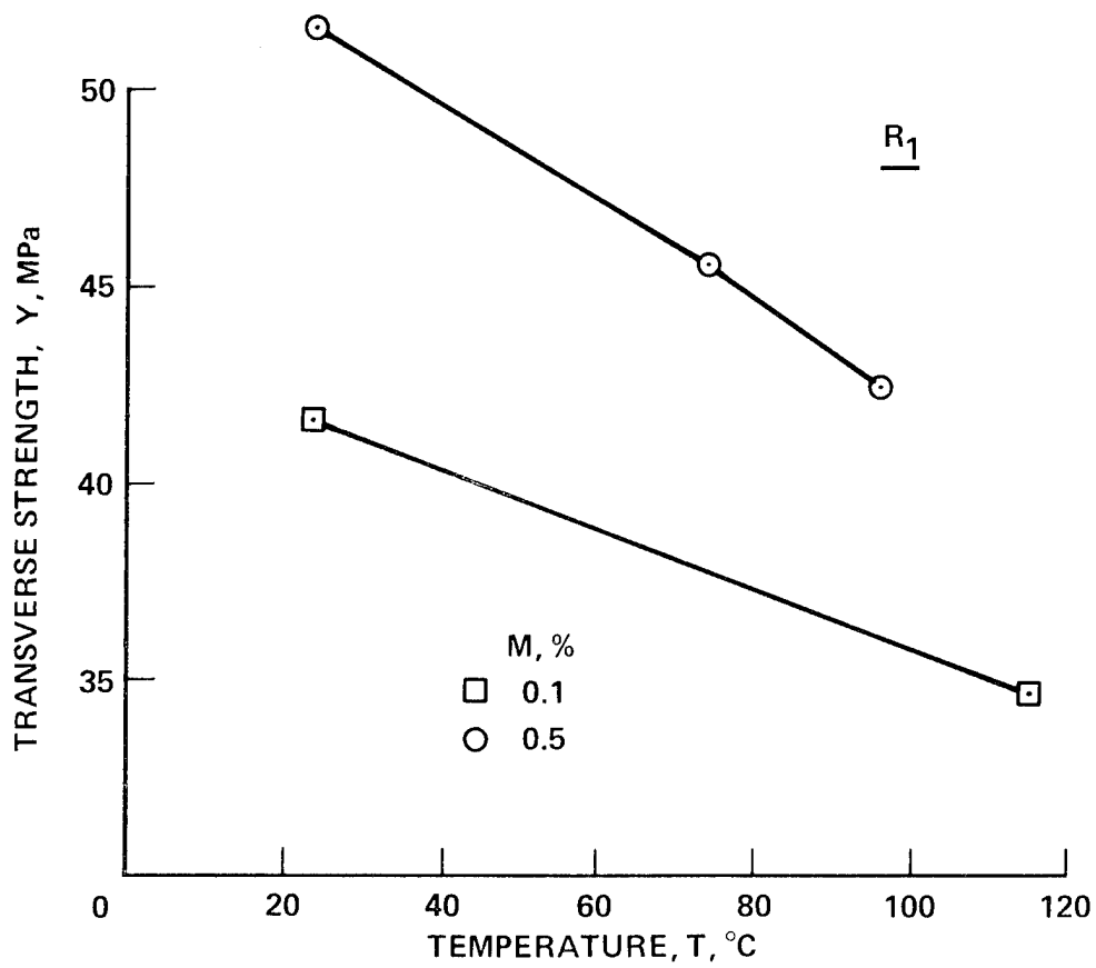
Figure 6.- Variation of transverse strength (Y) with temperature and moisture content.
