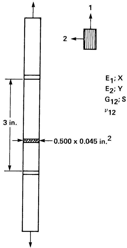
Figure 1.- Test specimen.
