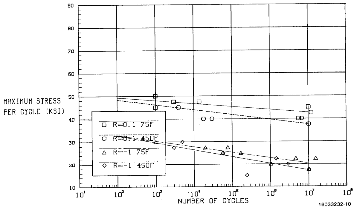
Figure 7. Axial fatigue data for HT-S/710 (0±45) S G/PI, unnotched, R=0.1, R=-1.
