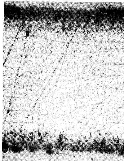
OC/PMR-15 2100 hr/316 °C 19.0% WEIGHT LOSS
