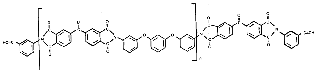
Figure 1. Specific designations: Thermid 600 when n = 1 , HR-60X when n = X .
