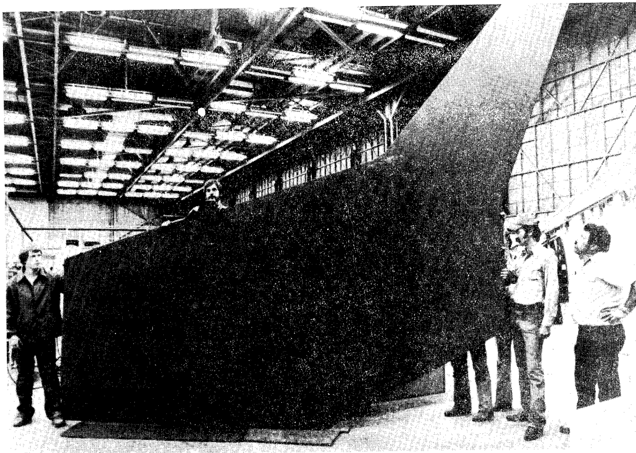
Figure 9. - Completed skin removed from tool after post cure.
