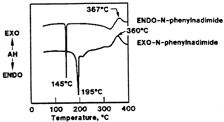
Figure 3.- Differential scanning calorimetry scans of endo- and exo-PN.
