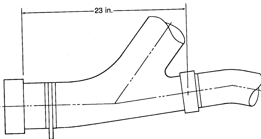
Figure 8. - 747 pneumatic duct.
