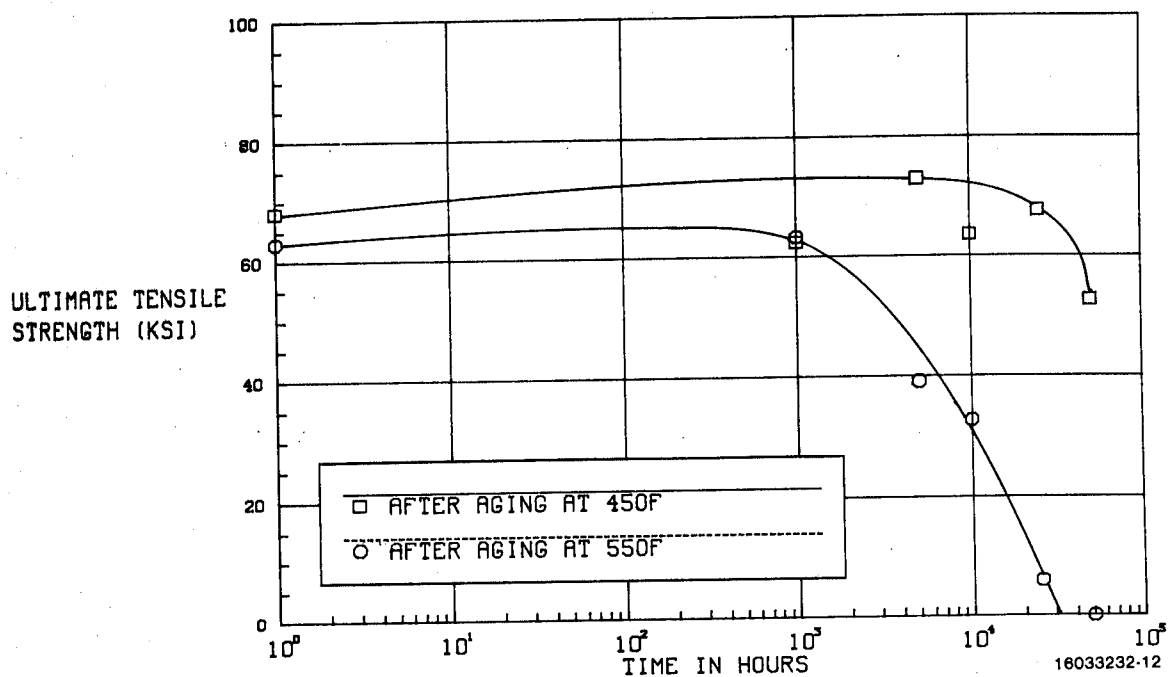
Figure 11. Tensile strength at aging temperature of HT-S/710 (0±45) S G/PI after thermal aging in 14.7 psi air at indicated temperatures.
