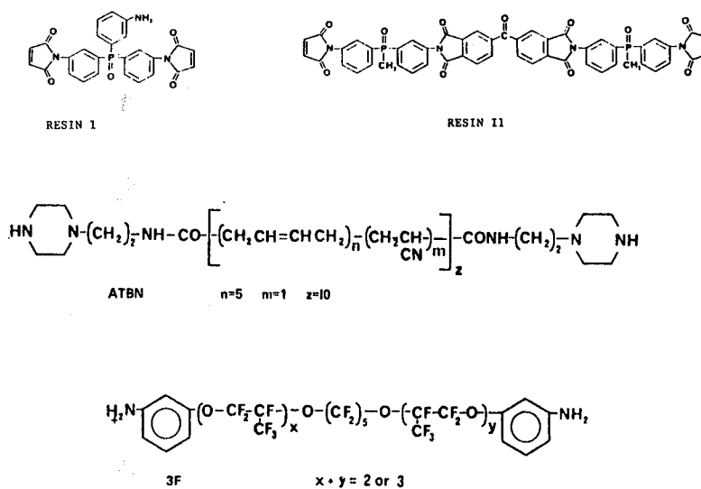
Figure 12. - Molecular structure of bismaleimide matrix resins prepared by replacing the methylene bridge with phosphonate linkages.
