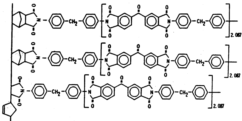
Figure 7. - Idealized structure for PMR-15.
