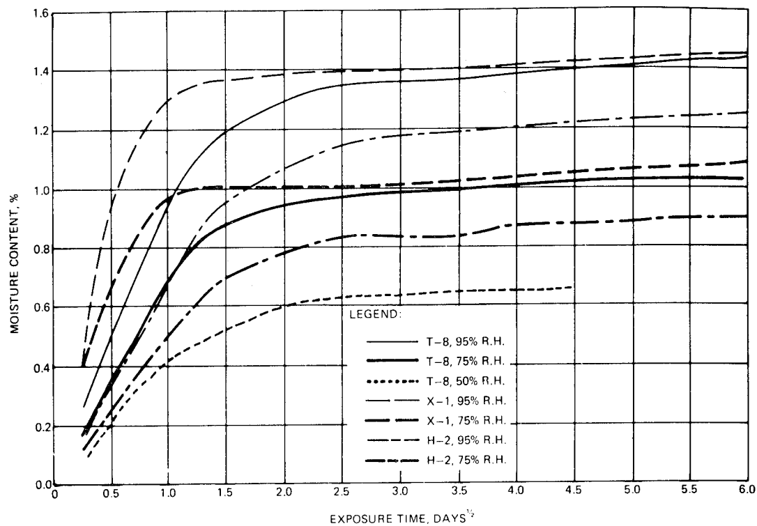
Figure 7. Effect of relative humidity on moisture content of 16-ply, T-300/F-178 graphite/polyimide panels at 77°C (170°F)
