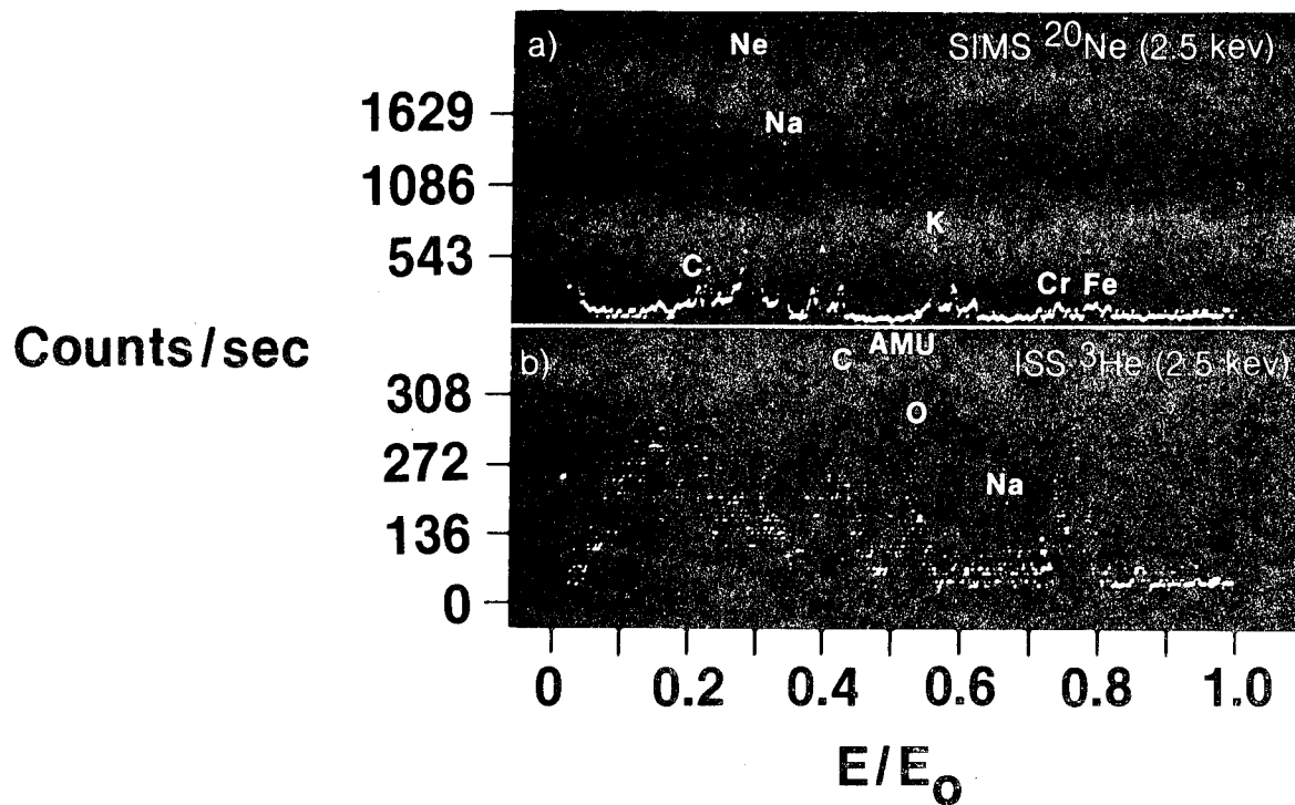
Figure 1. - ISS/SIMS spectra of Fortafil 5 unsized fiber \sim 10\text{\AA} .
