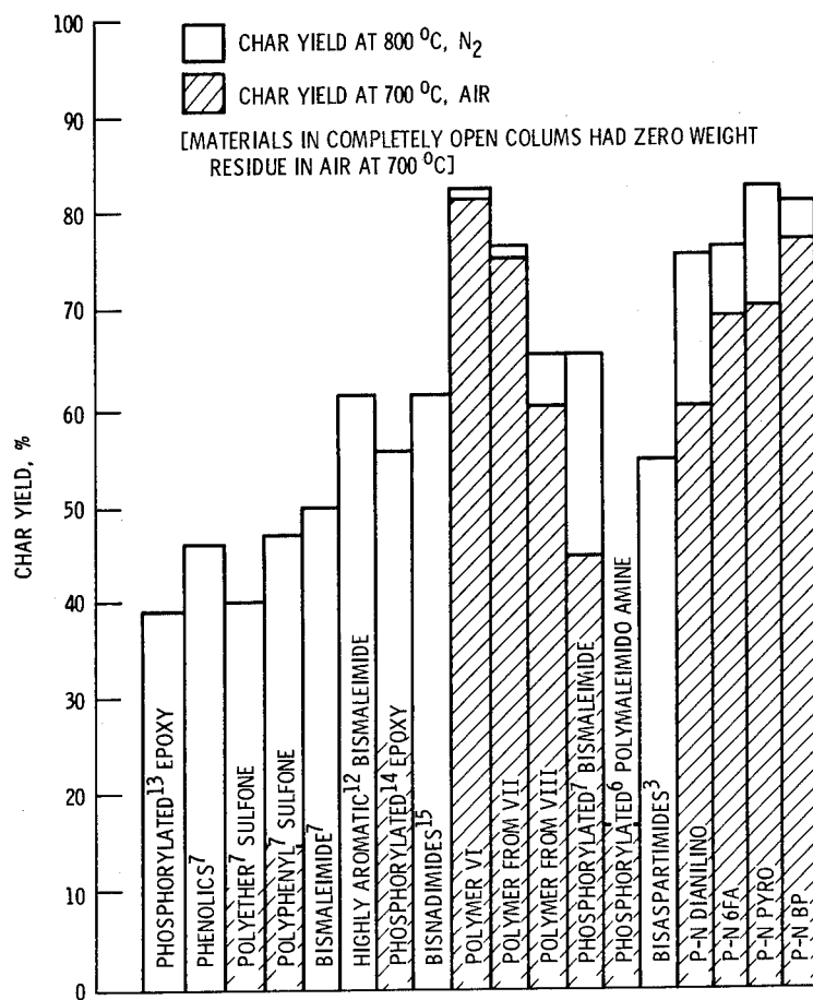
Figure 16. - Histogram comparing the thermal oxidative stability of tricyclic phosphazenes with state-of-the-art bisimides and aromatic matrix resin polymers.
