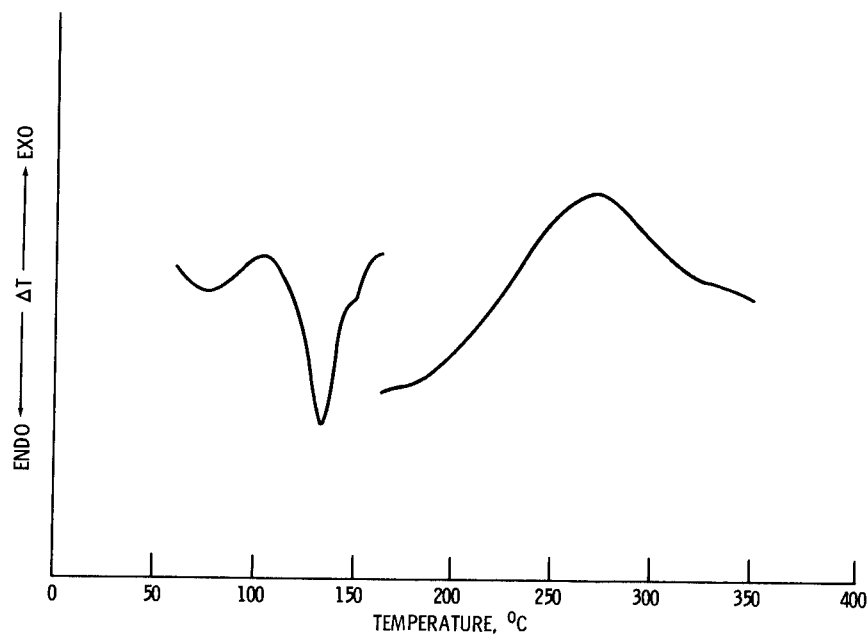
Figure 4. - Melting and polymerization behavior of bismaleimide resin M 751.
