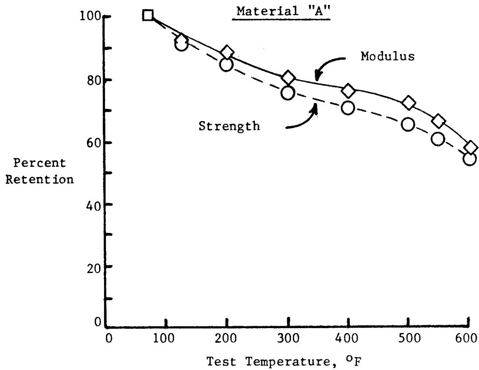
Figure 3. Effect of test temperature on the flexural properties of transfer-molded test bars of material "A".
