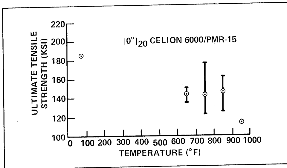
Figure 9 Short term thermal gradient tensile strength.
