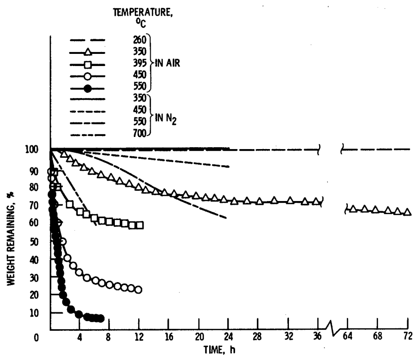
Figure 17. - Isothermal weight loss of (VI) at various temperatures.
