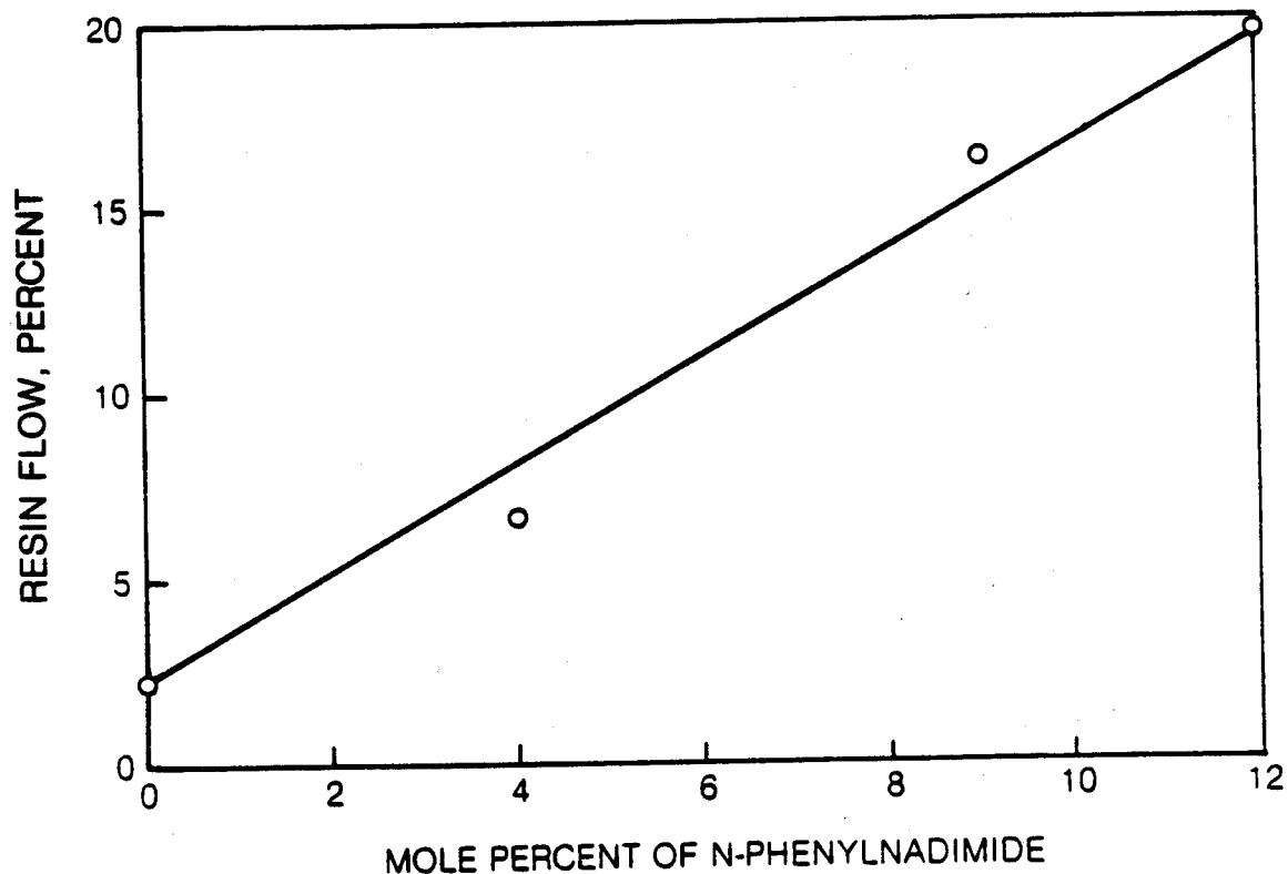
Figure 6. - Resin flow as function of PN concentration for Celson 6000/PMR-PN composites.
