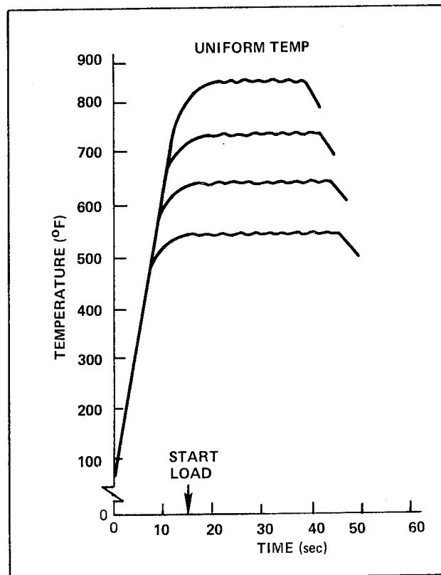
Figure 6 Transient temperature histories for 0° 6 ply tensile coupons.
