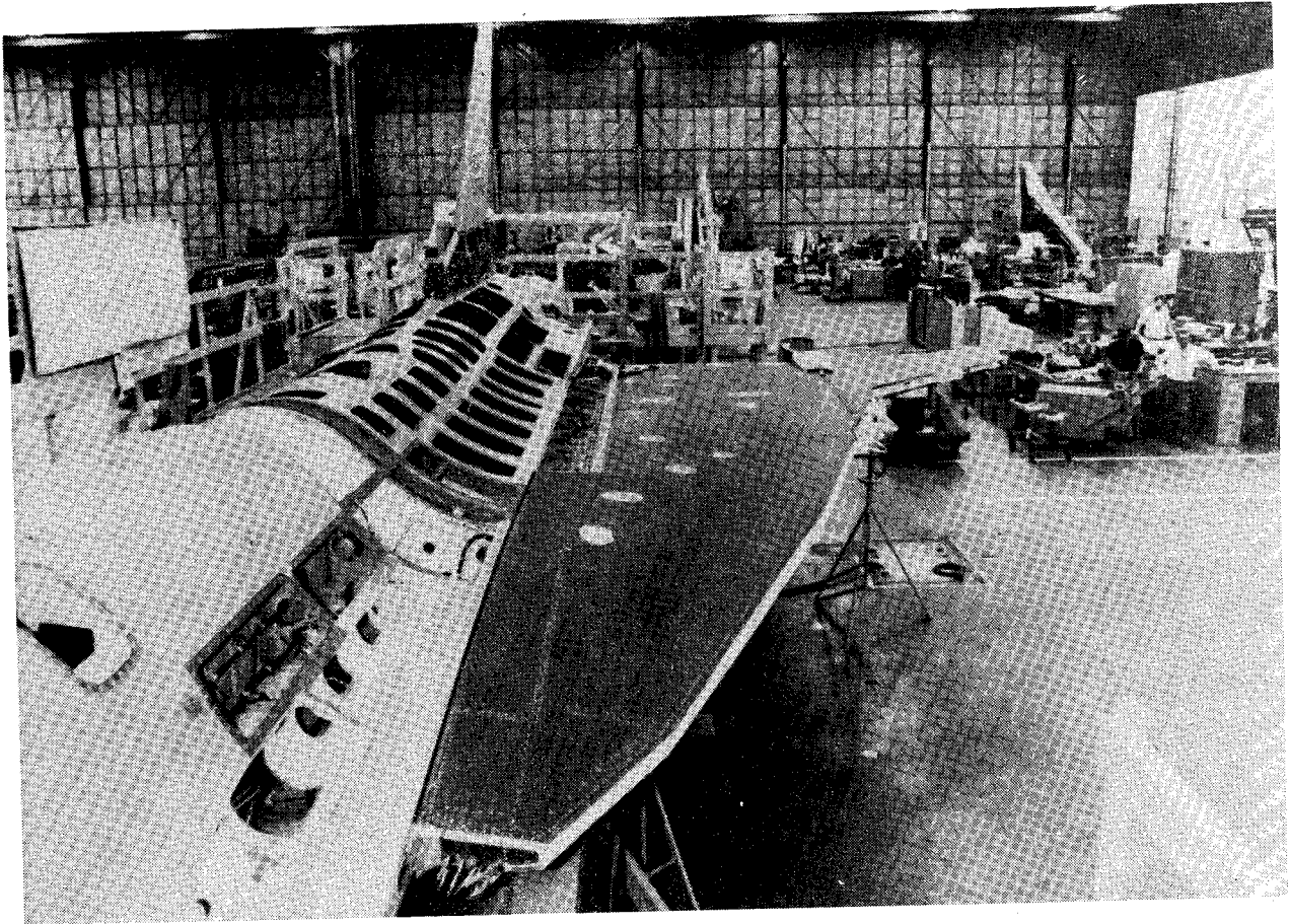
Figure 11. - Completed wing attached to fuselage.
