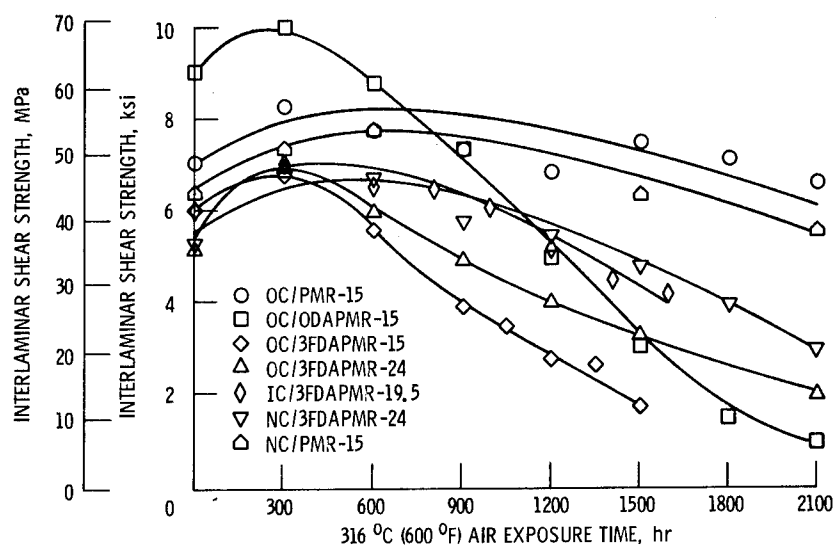
Figure 5. - 316 °C (600 °F) interlaminar shear strength of Celion 6000/PMR polyimide composites as function of 316 °C (600 °F) air exposure time.
