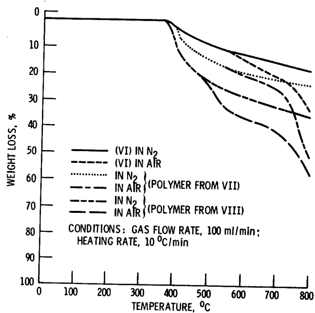
Figure 15. - Thermogravimetric analysis of cyclophosphazene polymers.
