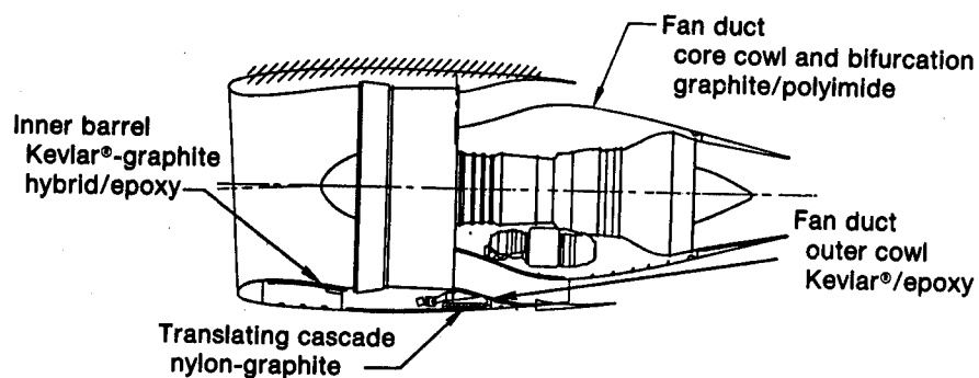
Figure 3. - Organic matrix composite applications in large turbofan engines.
