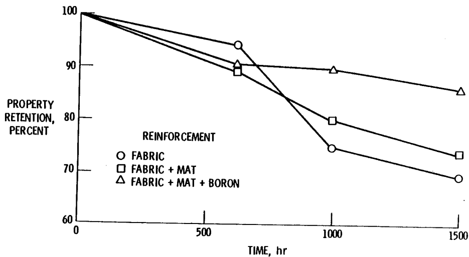
Figure 4. - Shear property retention of Cellion 3000 graphite fabric/PMR-15 laminates exposed in air at 316 °C and tested at 288 °C.
