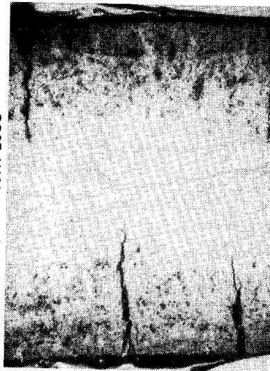
NC/3FDAPMR-24 2100 hr/316 °C 21.7% WEIGHT LOSS
