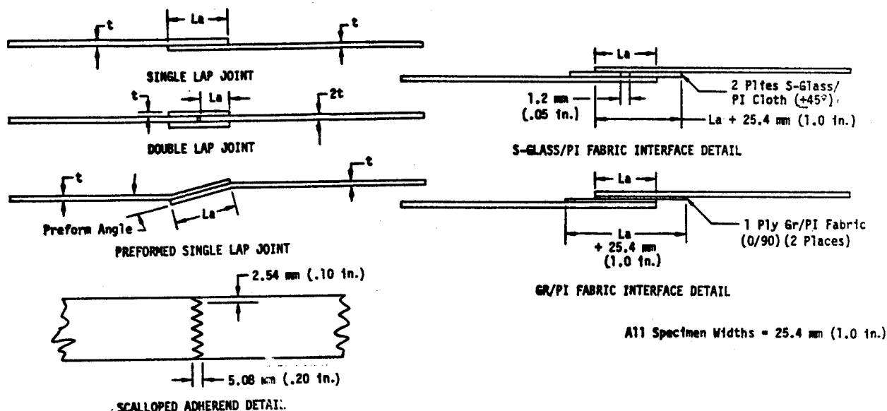
Figure 4: Advanced Joint Configurations
