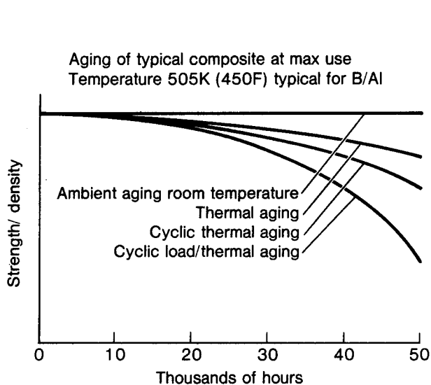
Figure 1. Characterization of composite material for up to 50,000 hours of supersonic cruise aircraft environment.
