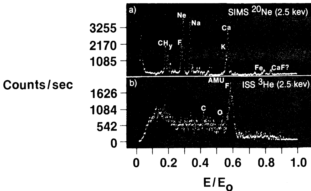
Figure 3. - ISS/SIMS spectra of Celion 6000 NR150B2 sized fiber \sim 10\text{\AA} .
