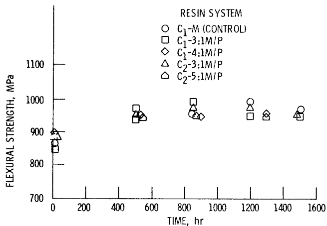
Figure 4. - Flexural strength of autoclave molded modified PMR-15/Celion 6000 graphite fiber composites exposed and tested at 316 °C.
