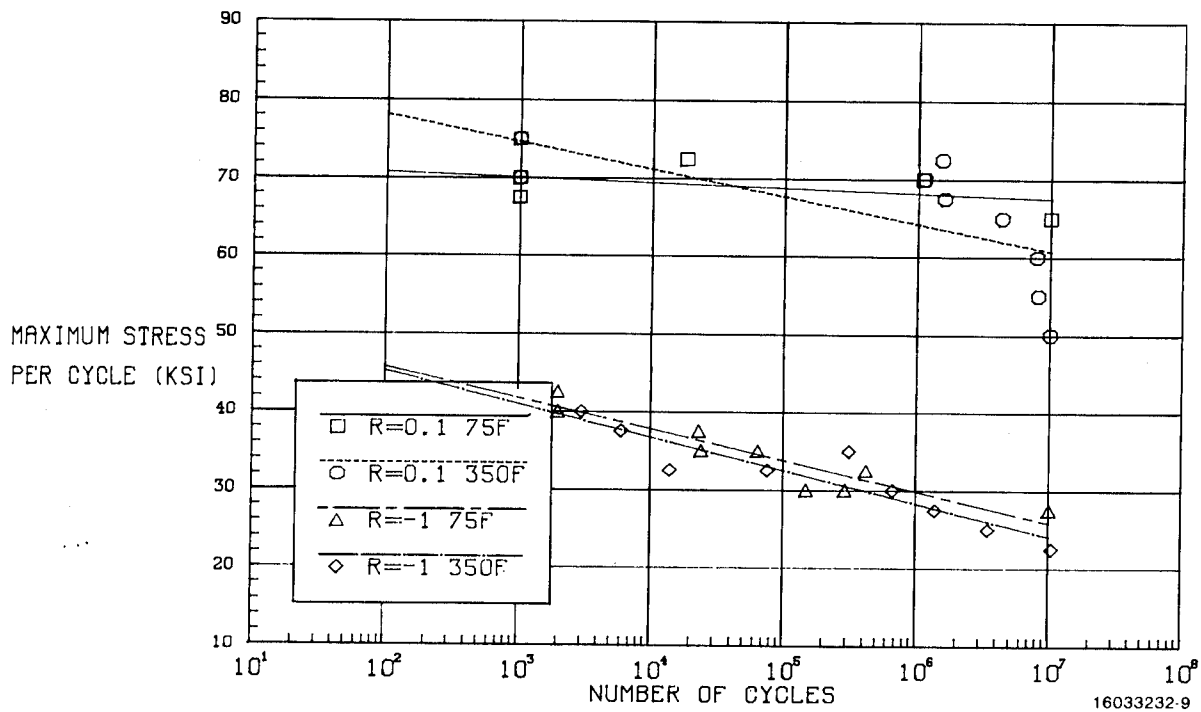
Figure 10. Axial fatigue data for Celion 6000/LARC-160 (0±45) S G/PI, notched, R=0.1 , R=-1 .
