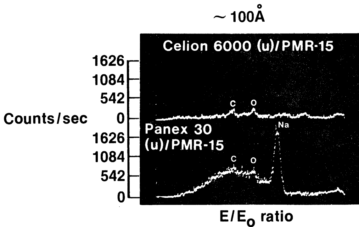
Figure 4. - ISS spectra of isothermally aged composites. (350 °C, 220 hrs, 1000 cc/min airflow)
