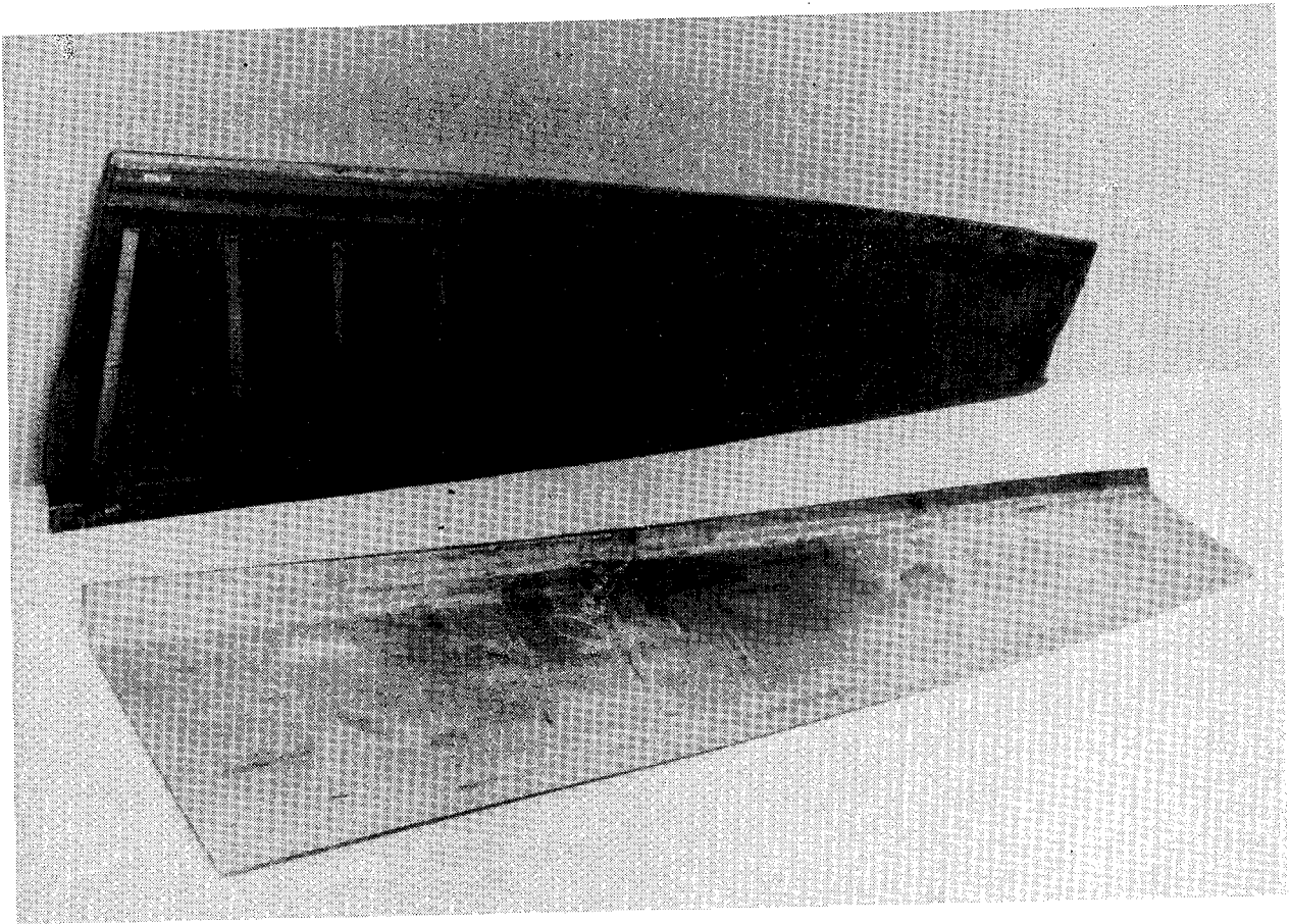
Figure 14. - Wing flap from another prototype aircraft with integrally cored V-378A/T-300 ribs bonded to a wing skin.
