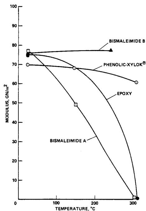
Figure 8. - Plot of modulus as function of temperature showing stability of bisimide B composite at temperatures which degrade both epoxy and bisimide A.
