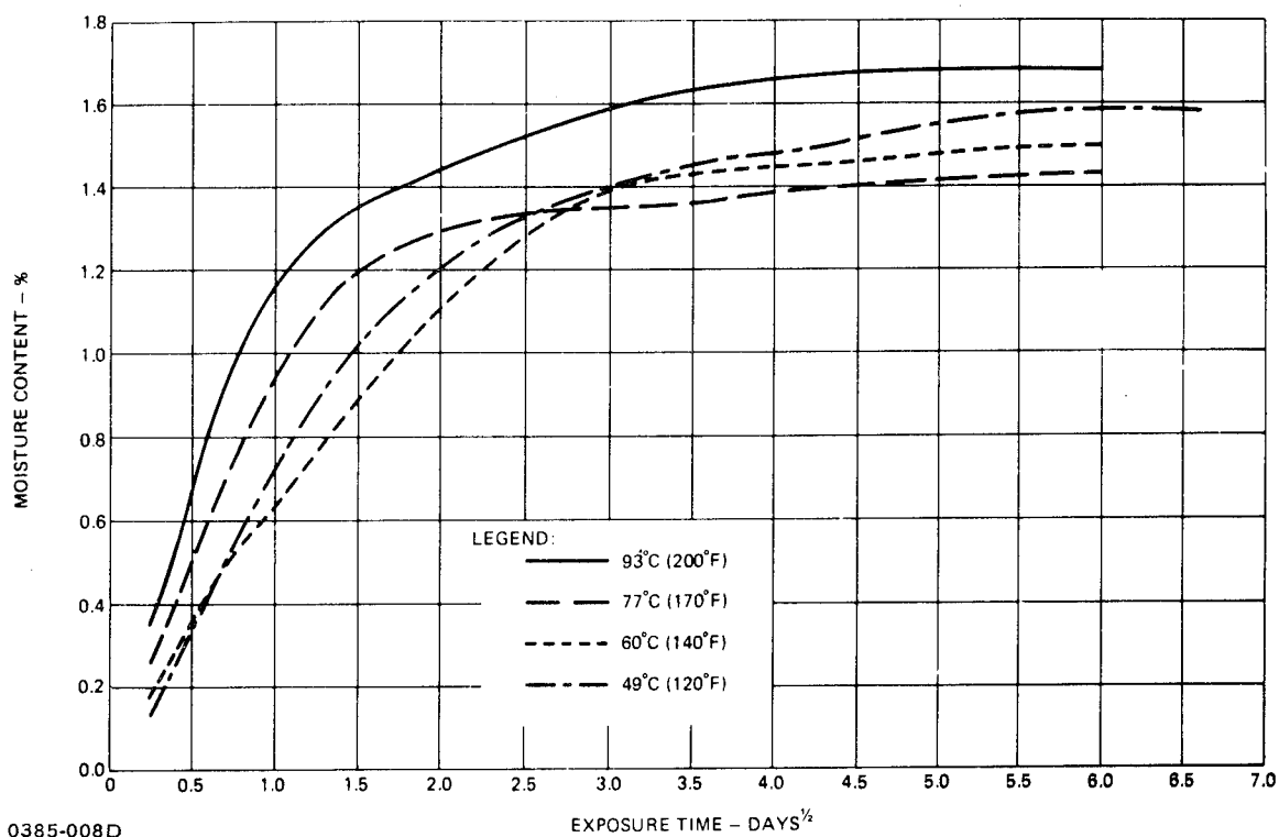
Figure 8. Effect of temperature on moisture diffusivity in 16-ply, T-300/F-178 graphite/polyimide panel No. T8 at 95% relative humidity
