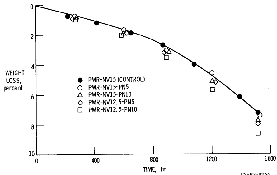
Figure 5. - Weight loss of Celion 6000 graphite fiber/PMR-NV polyimide composites in air at 316° C.
