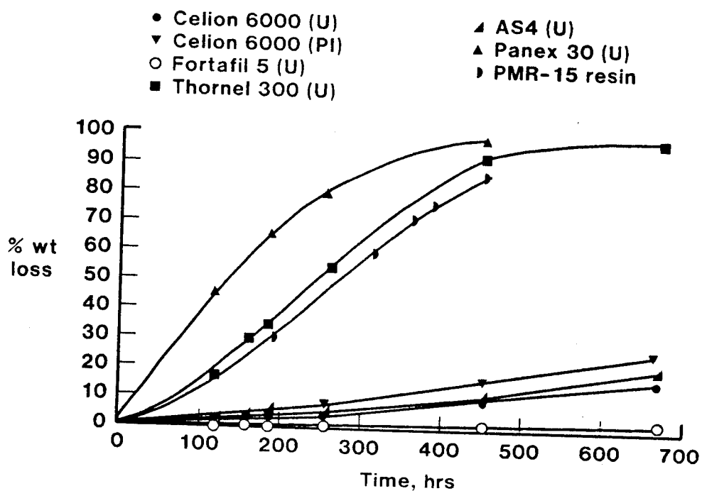
Figure 12. - Weight loss of component materials. (350 °C, 1000 cc/min airflow)
