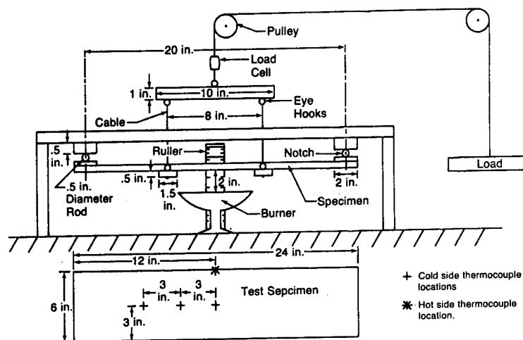
Figure 4. - Subcomponent hot side compression test rig. (900°F-2600°F.)
