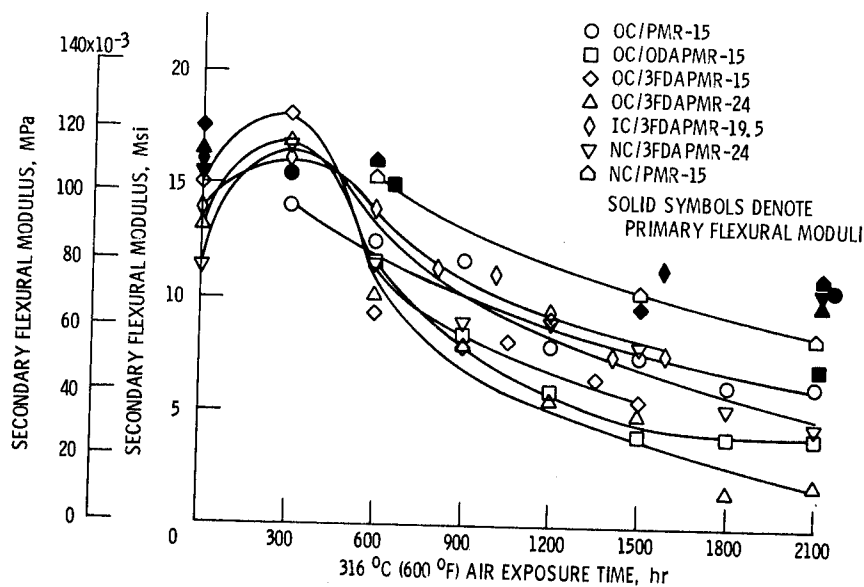
Figure 8. - 316 °C (600 °F) secondary flexural modulus of Celson 6000/PMR polyimide composites as function of 316 °C (600 °F) air exposure time.
