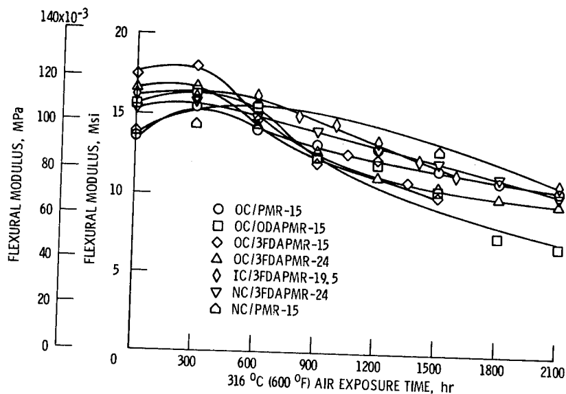
Figure 7. - 316 °C (600 °C) flexural modulus of Celson 6000/PMR polyimide composites as function of 316 °C (600 °F) air exposure time.
