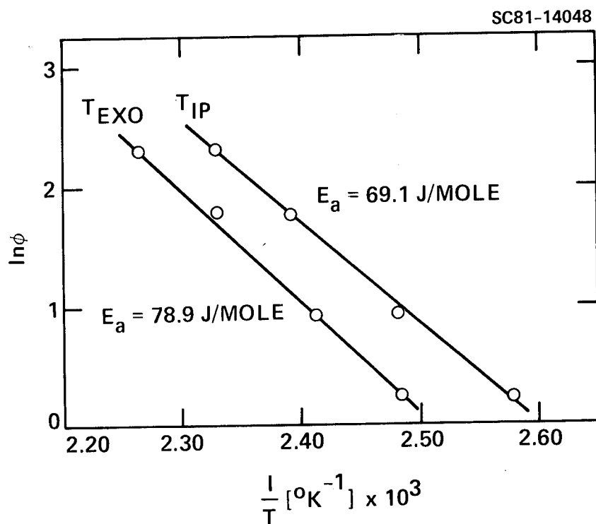
Figure 10. Dependence of DSC exotherm peak and inflection point temperature with heating rate for U.S. Polymeric V378A resin.
