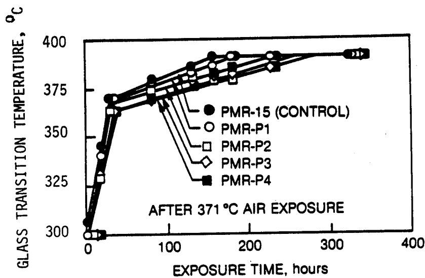
Figure 10. - Glass transition temperature as function of exposure time for as fabricated Cellion 6000/PMR-PN composites.
