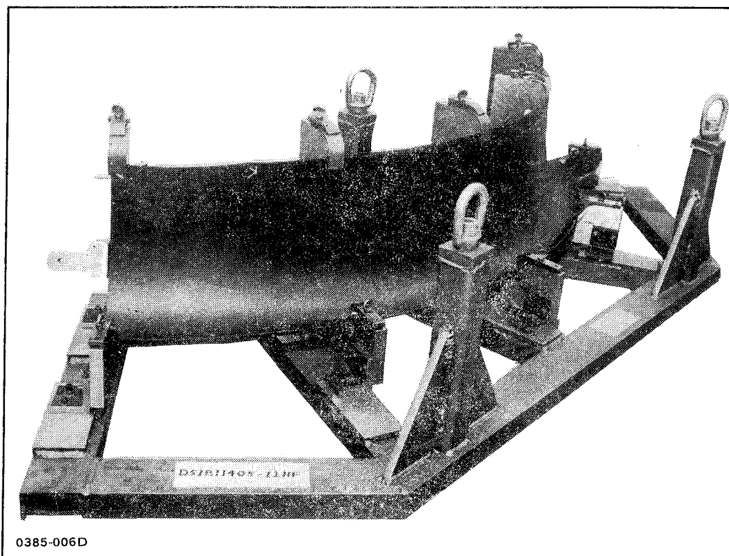
Figure 6. Section of graphite/polyimide DC-8 nacelle anti-ice plenum in postcuring fixture
