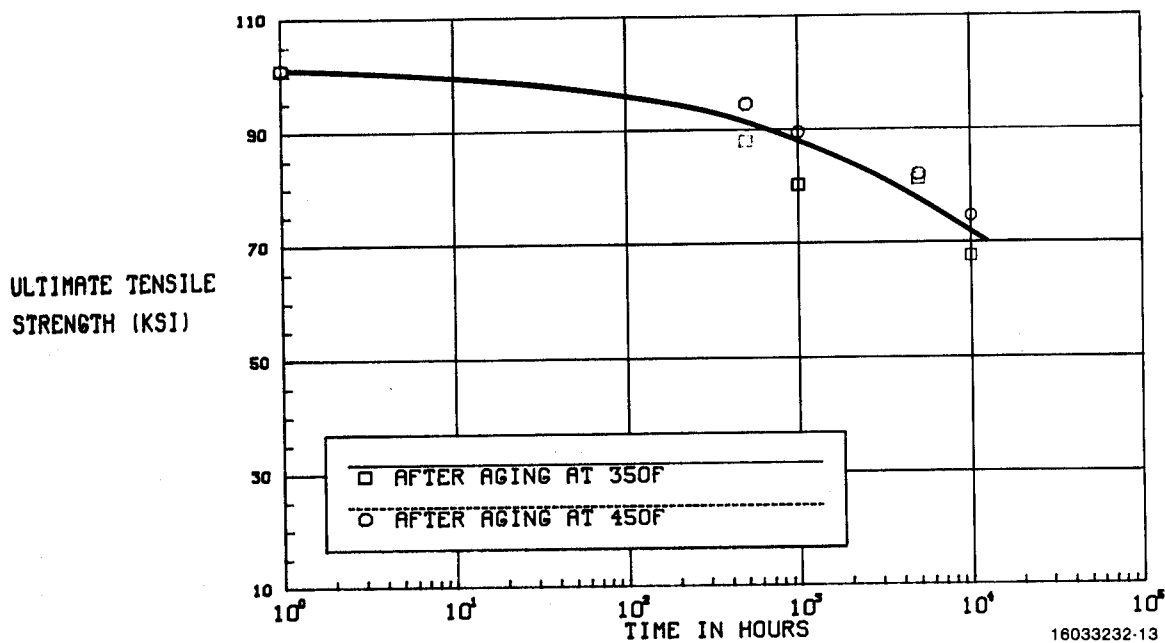
Figure 12. Tensile strength of Celion 6000/LARC-160 (0±45) S G/PI at 350F after thermal aging in 14.7 psi air at the indicated temperatures.
