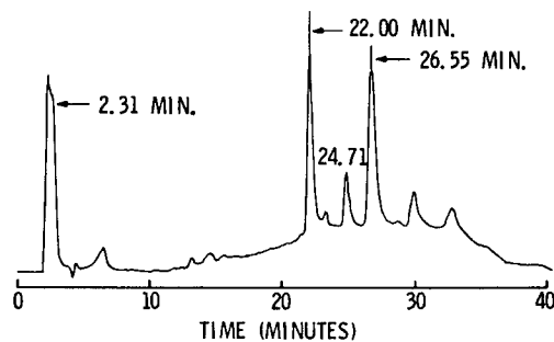
FIGURE 6 CHROMATOGRAM OF LARC 160 WITH AP-22
