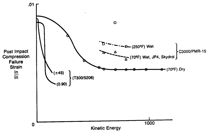
Figure 3. - Damage tolerance.
