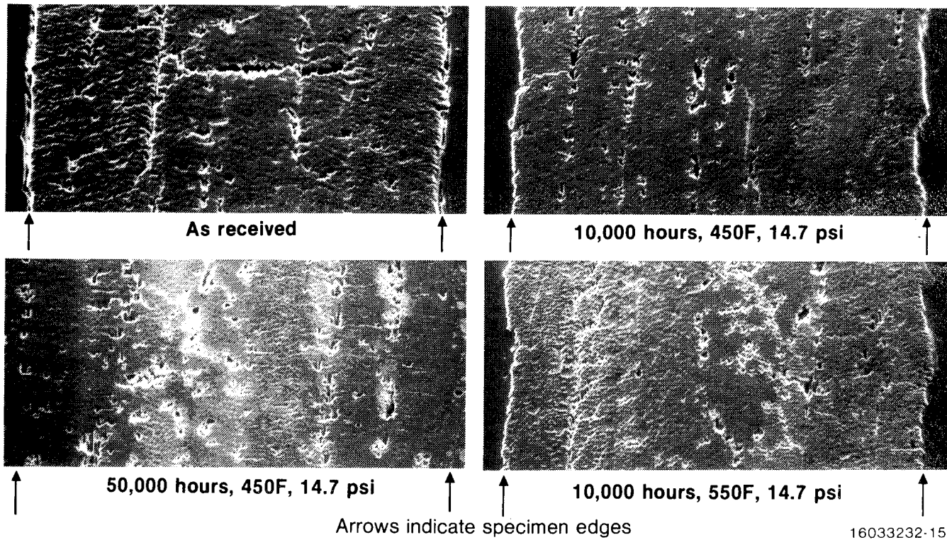
Figure 13. HT-S/710 graphite/polyimide after thermal aging at indicated conditions (100 \times ).
