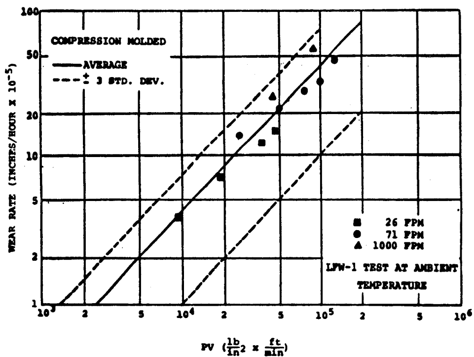
Figure 5. Wear of compression-molded material "A".
