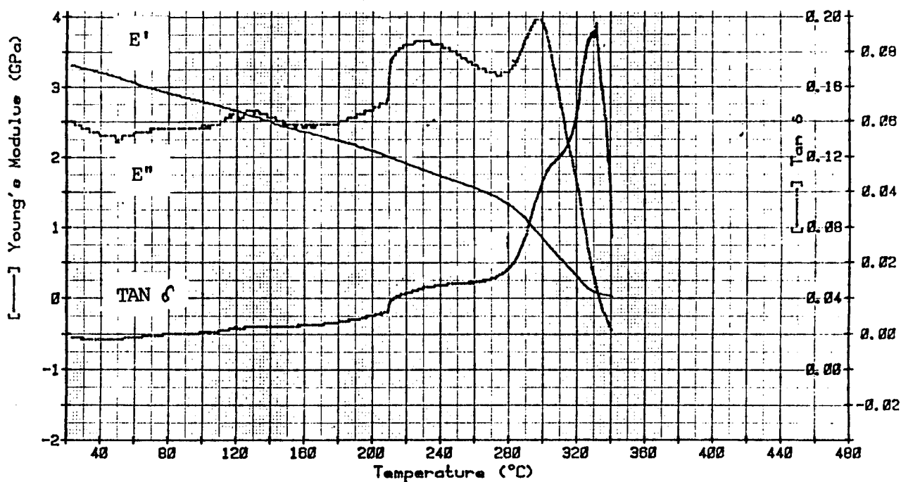
Figure 3. Dynamic mechanical analysis of EA9673, dry.
