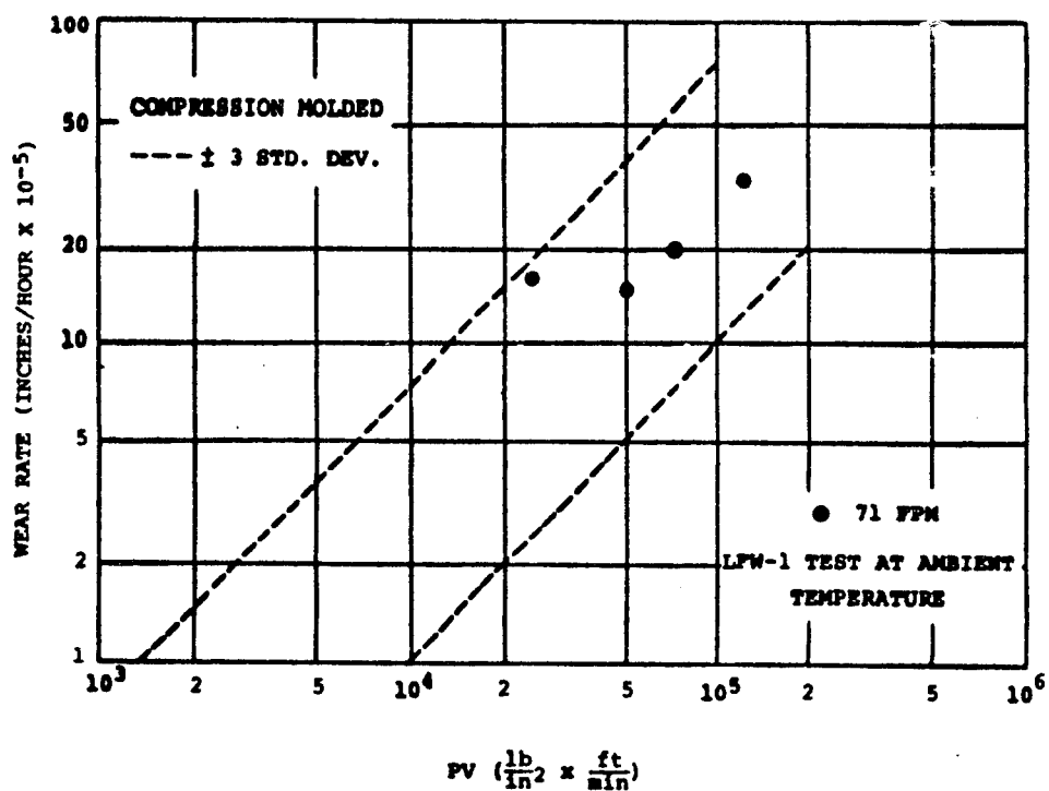
Figure 6. Wear of transfer-molded material "A".
