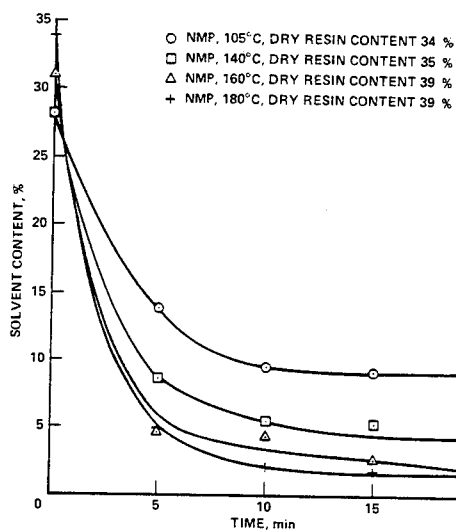
Figure 5. - Plot of solvent content as function of time showing remaining traces of solvent.
