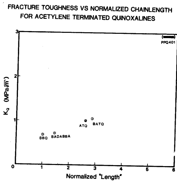
FIGURE 7. Fracture Toughness of the Quinoxaline Resins.
