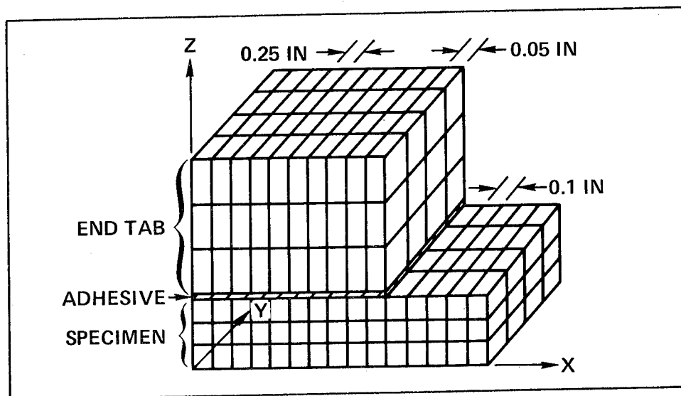
Figure 10 F.E. idealization of test coupon.
