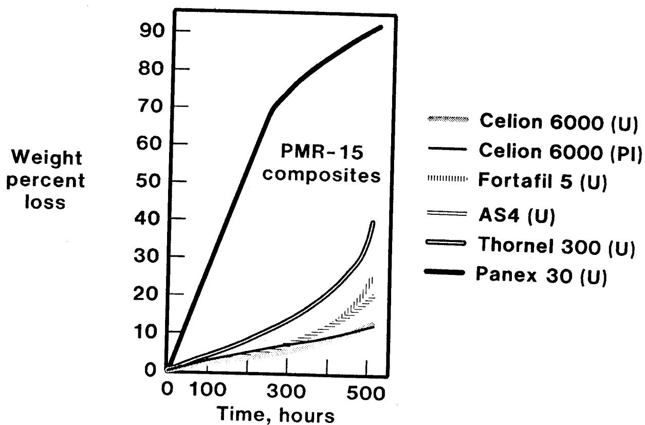
Figure 13. - Composite weight loss. (350 °C, 1000 cc/min airflow)
