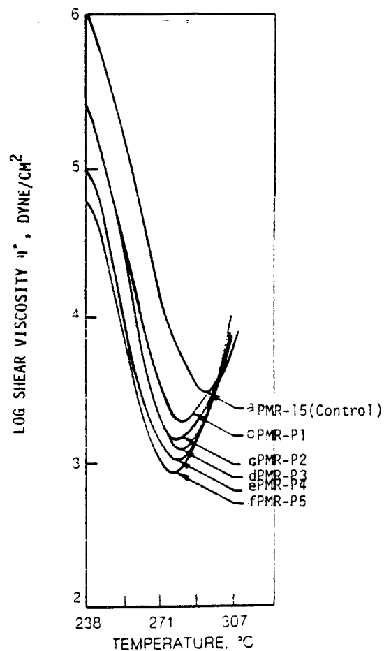
Figure 4. - Log shear viscosity as function of temperature for PMR-PN molding powders.
