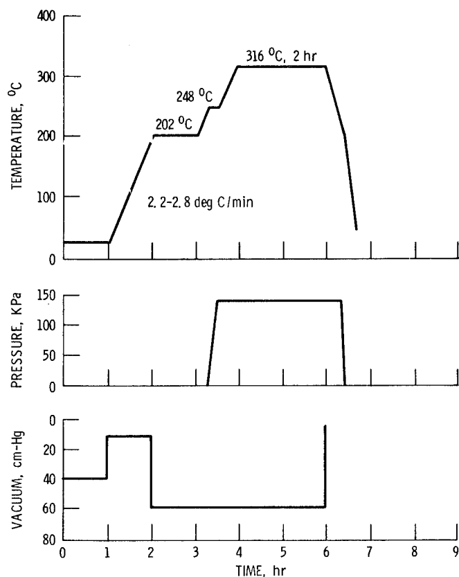
Figure 3. - Typical autoclave cure cycle for PMR-15 materials.
