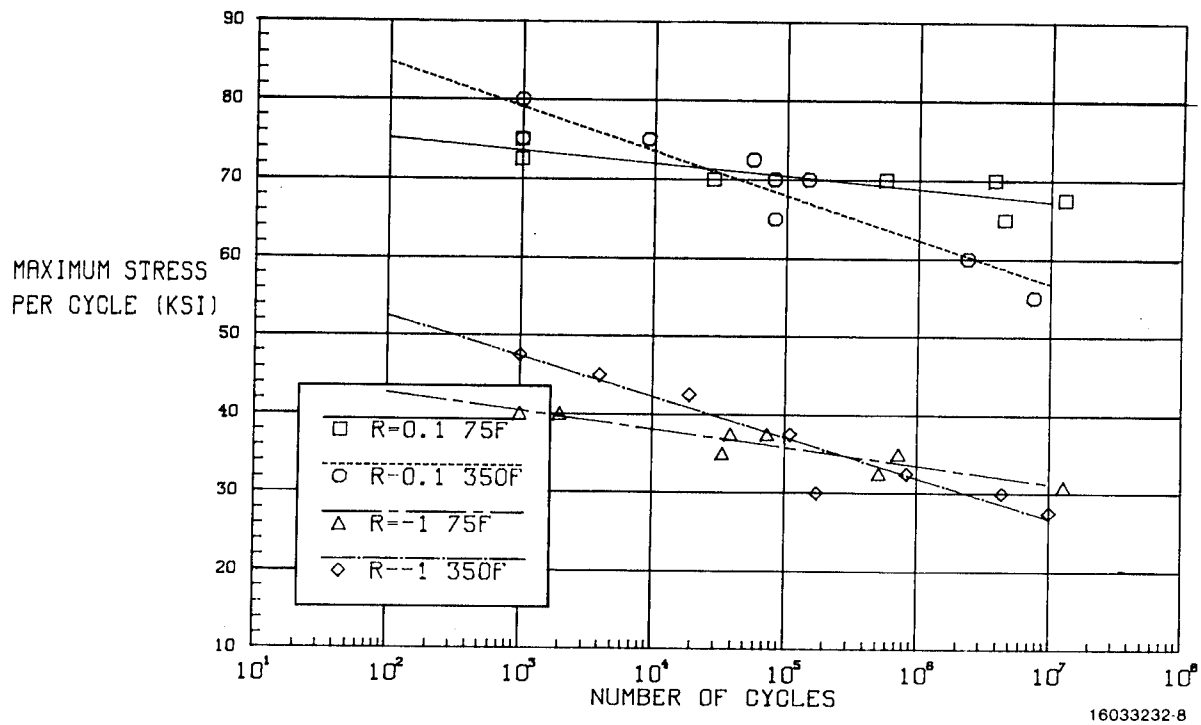
Figure 9. Axial fatigue data for Celion 6000/LARC-160 (0±45) S G/PI, unnotched, R=0.1 , R=-1 .
