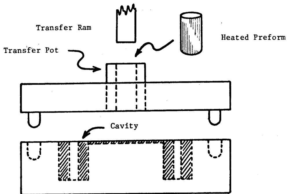
Figure 1. Simplified schematic of a typical transfer mold.
