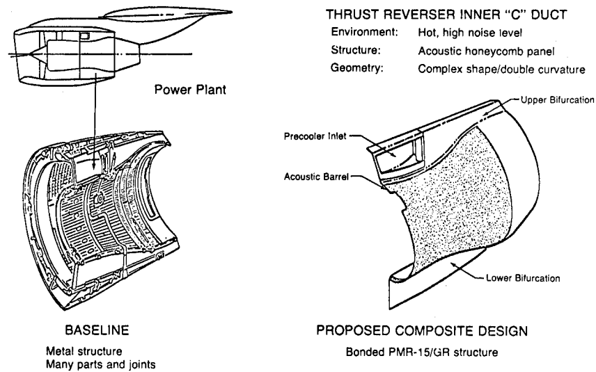
Figure 4. - Schematic of Thrust Reverser Fixed Structure "C" duct of 757 aircraft.
