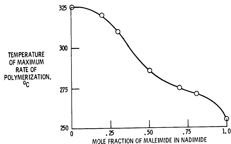
Figure 5. - Calculated dependence of maximum polymerization rate on concentration of maleimide in nadimide.
