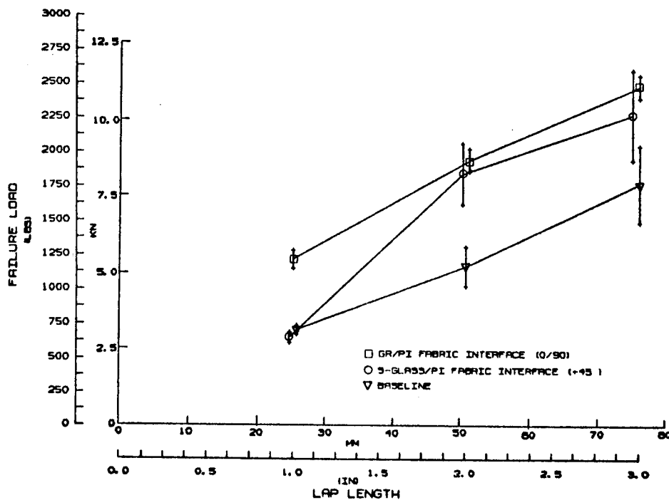
Figure 14: Effect of Fabric Interfaces - Single-Lap Joints
