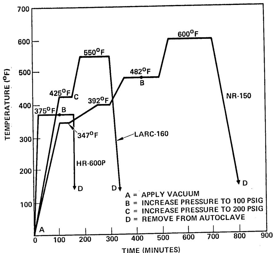
Figure 11. - Comparison of autoclave cycles of HR600P with high performance resins LARC-160 and NR-150.
