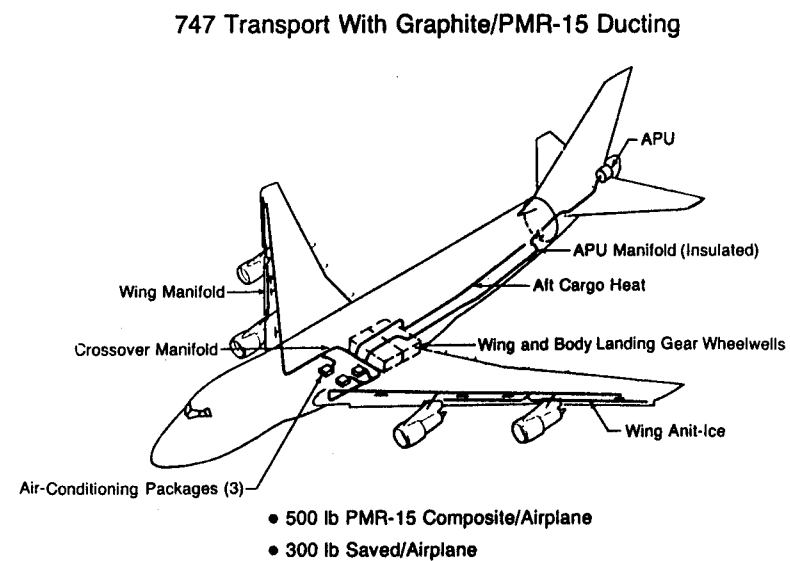
Figure 6. - Potential near term applications of PMR-15.
