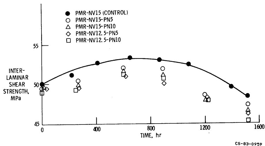
Figure 6. - Interlaminar shear strength of Celion 6000 graphite fiber/PMR-NV polyimide composites exposed and tested in air at 316° C.
