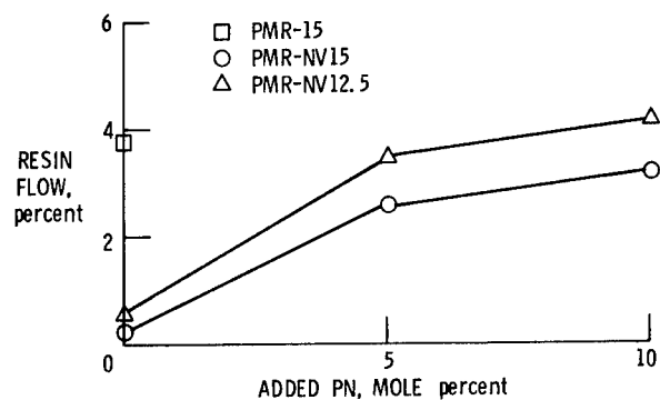
Figure 4. - Resin flow of PMR-NV polyimides.
