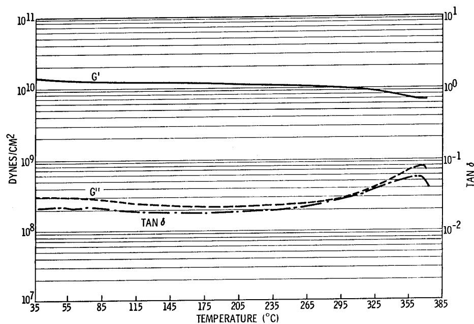
FIGURE 22 LARC 160, AP-22 (NEAT RESIN CASTING)
