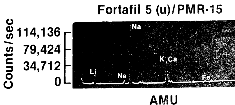
Figure 5. - SIMS spectra of isothermally aged composites. (350 °C, 220 hrs, 1000 cc/min airflow)
