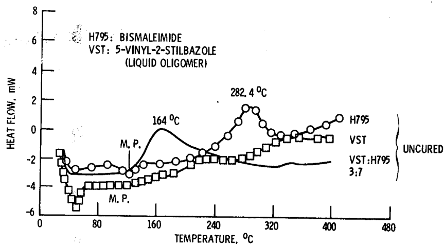
Figure 11. - DSC of bismaleimide (H 795) and VST/H 795 copolymers.
