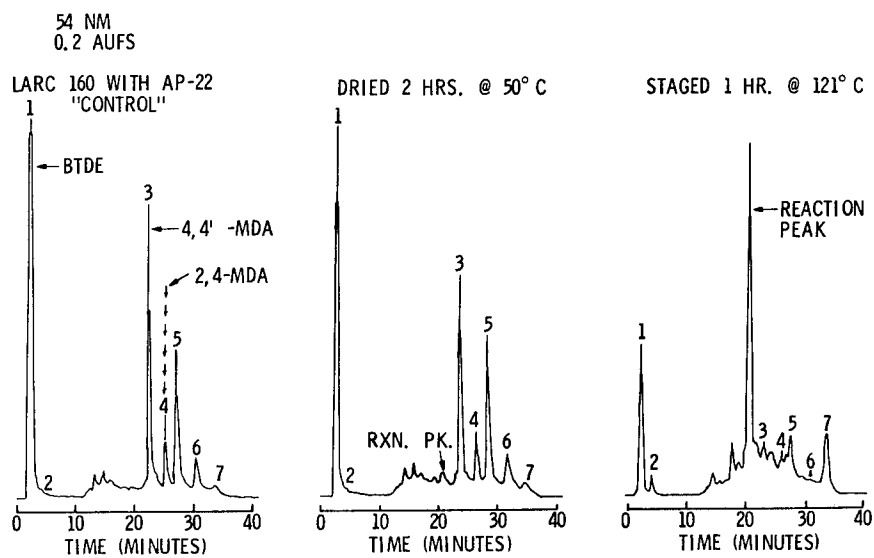
FIGURE 8 EFFECTS OF STAGING ON HPLC CHROMATOGRAMS
