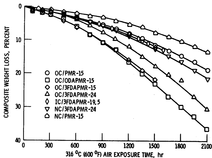
Figure 2. - Composite weight loss of Celson 6000/PMR polyimide composites as function of 316 °C (600 °F) air exposure time.
