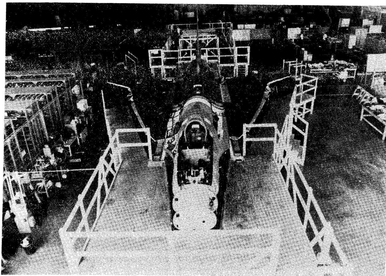
Figure 12. - Fuselage with both wings attached.
