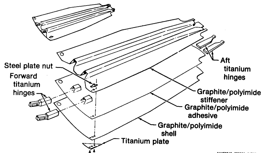
Figure 7. - Schematic of F100 composite nozzle flaps.
