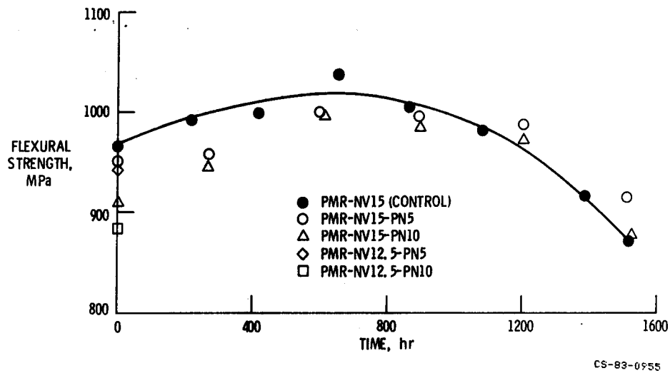
Figure 7. - Flexural strength of Celion 6000 graphite fiber/PMR-NV polyimide composites exposed and tested in air at 316° C.
