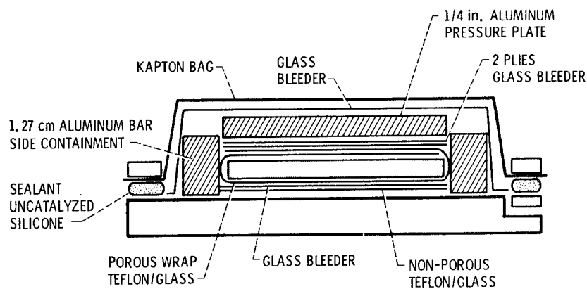
Figure 1. - Vacuum bag layup for unidirectional reinforced PMR-15/Celion 6000.
