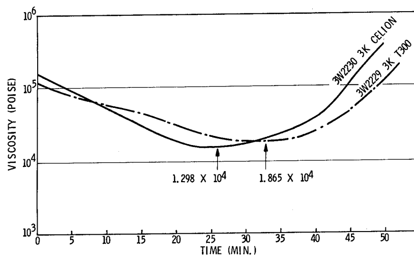
FIGURE 21 V378 PREPREG VISCOSITY VS TIME
