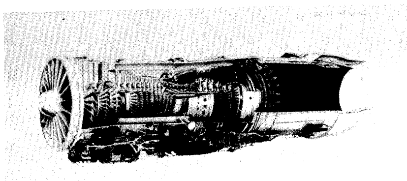
Figure 1. - F100 turbofan engine.
