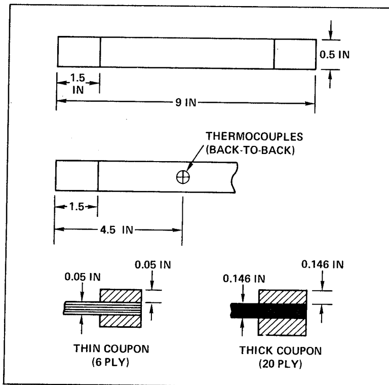
Figure 2 Test coupon and instrumentation details.
