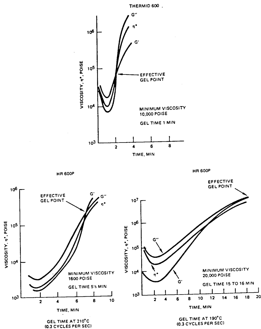
Figure 9. - Gel times of Thermid 600 and HR600P.
