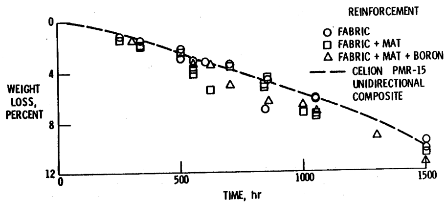
Figure 1. - Weight loss of Celion 3000 graphite fabric/PMR-15 laminates exposed in air at 316 °C.
