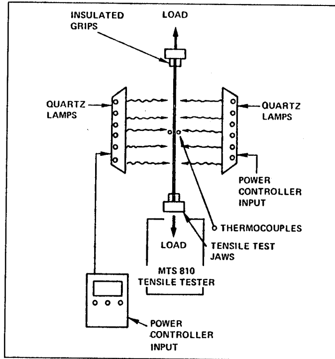
Figure 3 Transient heating/tensile loading schematic.
