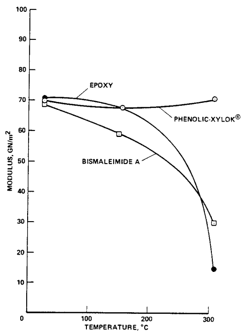
Figure 6. - Plot of modulus as function of temperature showing the decrease in modulus from room temperature to 300 °C.
