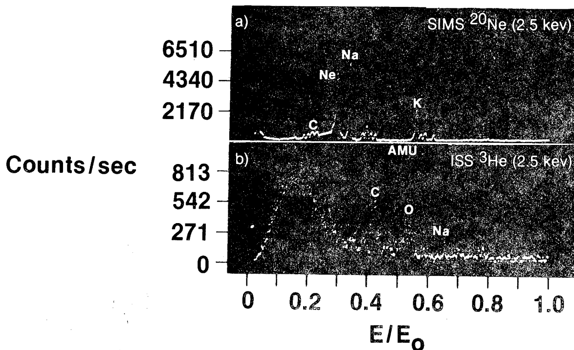
Figure 2. - ISS/SIMS spectra of Fortafil 5 sized fiber \sim 10\text{\AA} .
