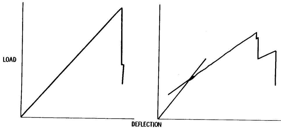
Figure 3. - Typical flexural load - deflection curves of Cellion 3000 graphite fabric/PMR-15 laminates; (a) tested at 288 °C after postcure (b) tested at 288 °C after 624 hr exposure in air at 316 °C.
