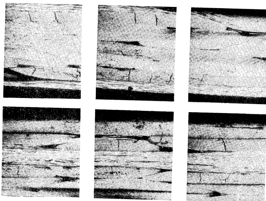
Figure 10. - 4 ply composite following exposure at 473°F. (Top: Along 0° axis. Bottom: Along -45° axis.)
