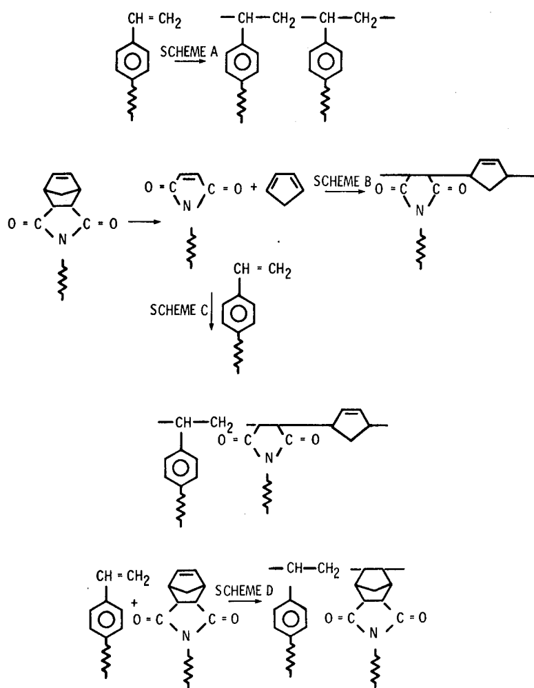
Figure 3. - Possible crosslinking reactions of PMR-NV polyimides.
