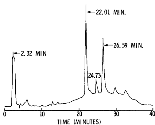
FIGURE 7 CHROMATOGRAM OF LARC 160 WITH CURITHANE 103
