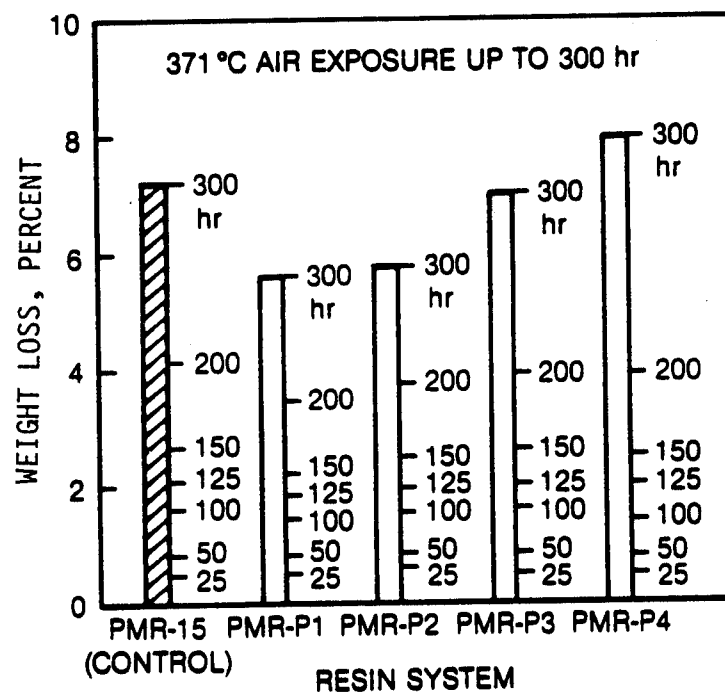
Figure 9. - Weight loss of postcured Cellion 6000/PMR-PN composites.
