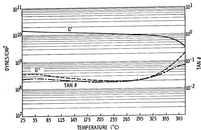
FIGURE 23 LARC 160, CURITHANE 103 (NEAT RESIN CASTING)
