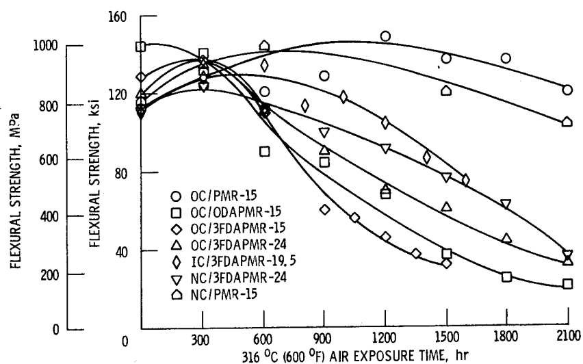
Figure 6. - 316 °C (600 °F) flexural strength of Celion 6000/PMR polyimide composites as function of 316 °C (600 °F) air exposure time.
