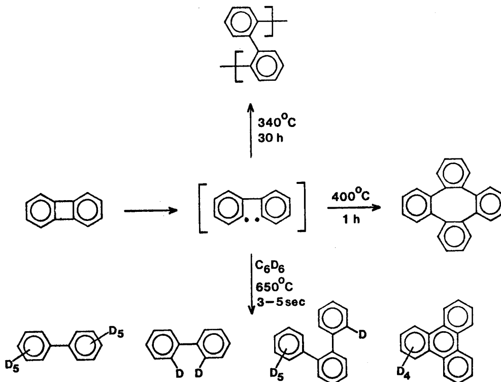
Figure 1. The products of the pyrolysis of biphenylene under various conditions.
