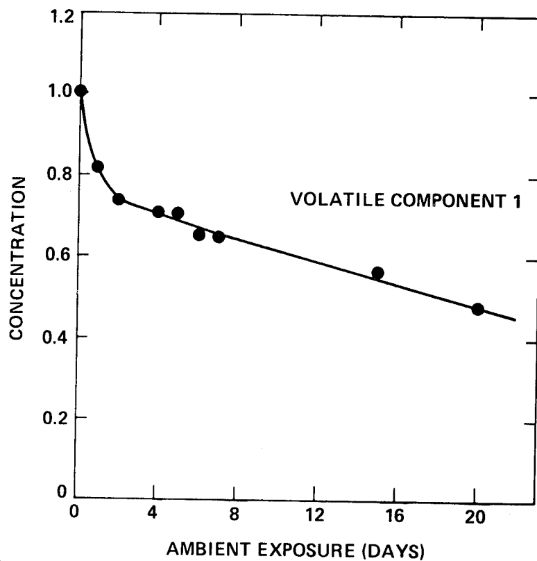
Figure 11. Effect of ambient aging on the concentration of Volatile Component 1 in U.S. Polymeric V378A resin.
