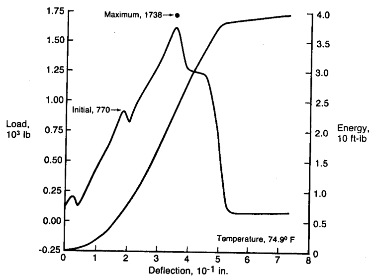
Figure 2. - Through penetration impact test.
