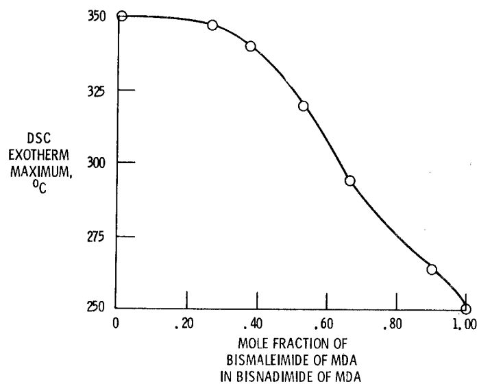
Figure 3. - Variation of cure exotherm maximum with concentration of bismaleimide in nadimide.
