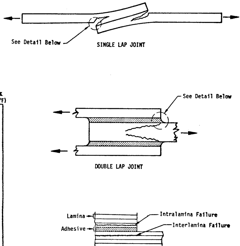
Figure 6: Peel Failures of Composite Bonded Joints
