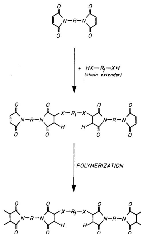
Figure 7. - Chemistry of H 795 resin.
