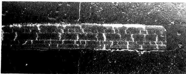
Figure 14. Celion 6000/LARC-160 graphite/polyimide after thermal aging at indicated conditions (13 \times ).
