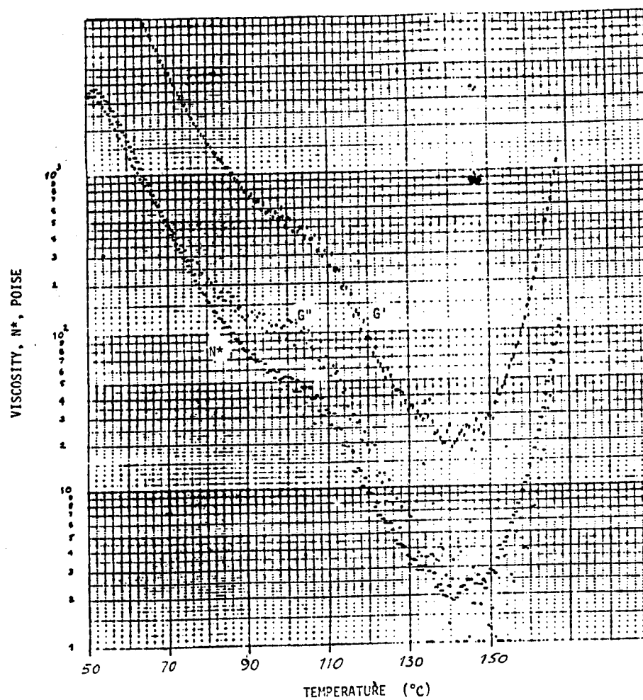
Figure 2. Rheometrics plot for EA9673 resin.
