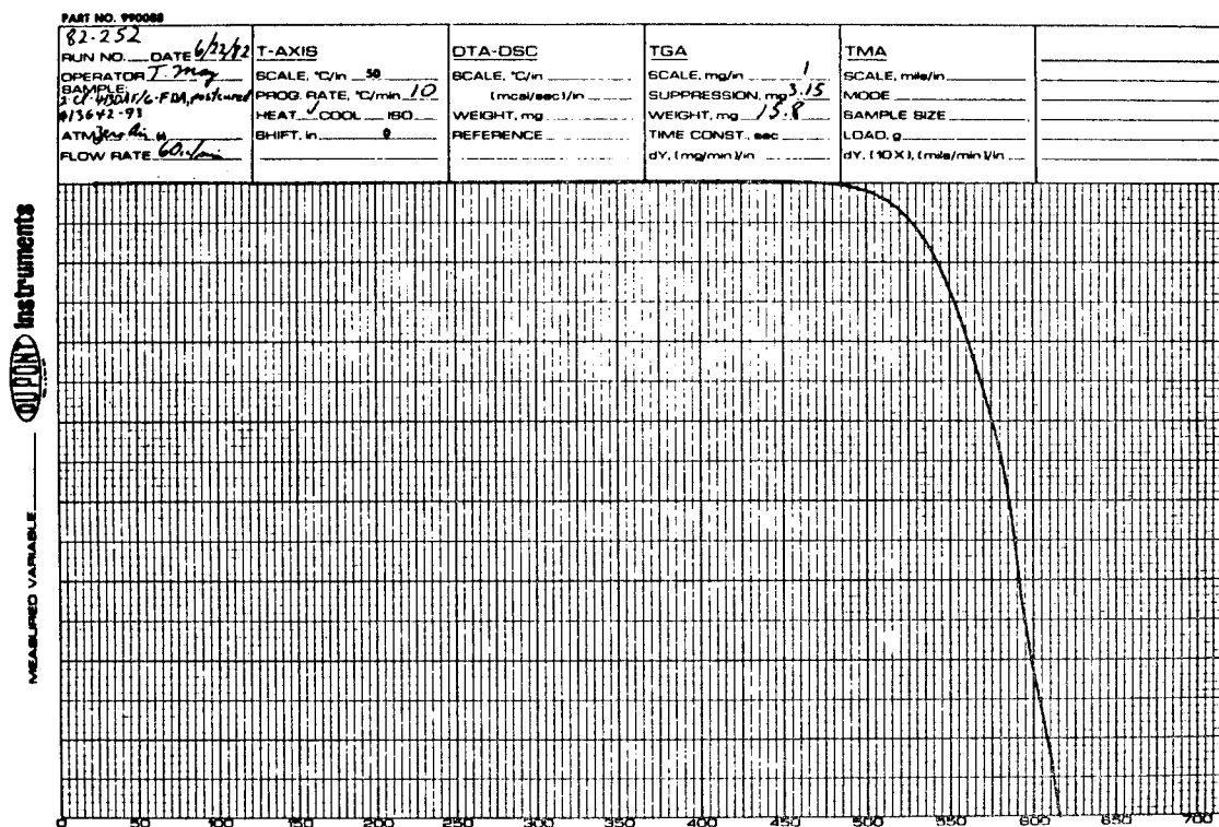
Figure 2. Thermogram of 2-CL-4-BDAF/6-FDA.
