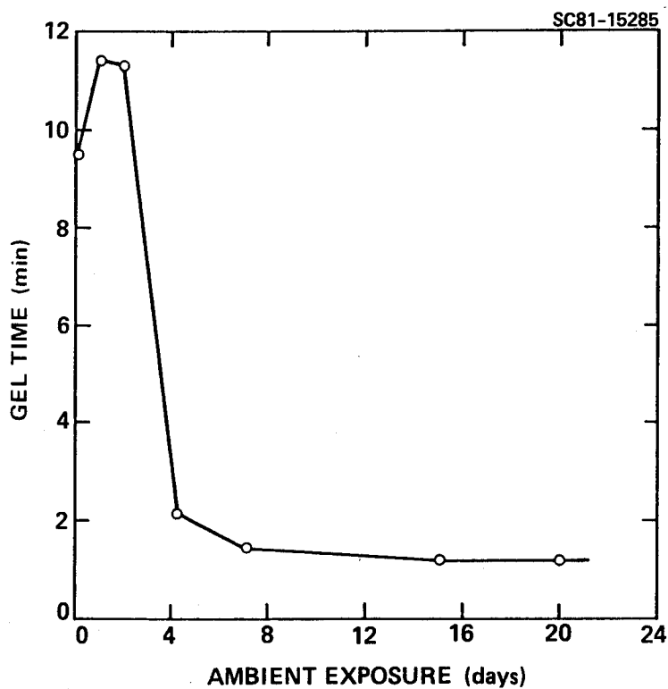
Figure 14. Effect of ambient aging on the time of gelation at 398K for U.S. Polymeric V378A resin.
