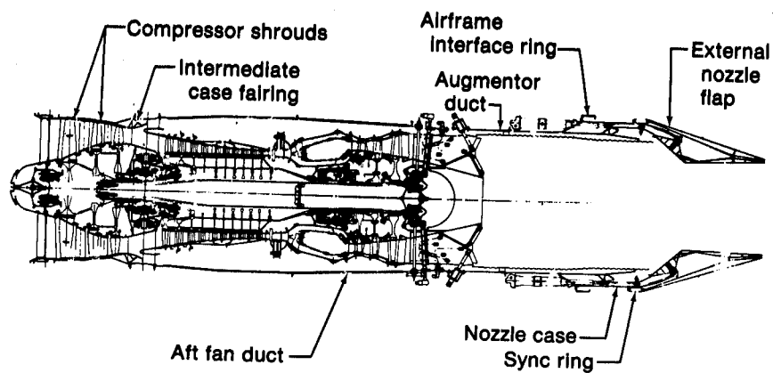
Figure 4. - Organic matrix composite applications in augmented turbofan engines.
