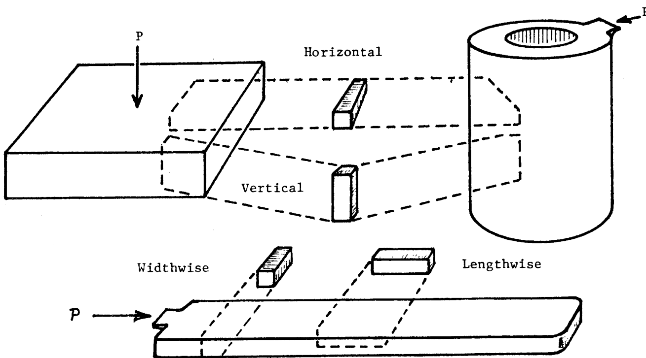
Figure 2. The three basic kinds of molded pieces from which test specimens were taken. "P" indicates the direction of applied pressure (compression molding) or the point of resin injection (transfer molding).
