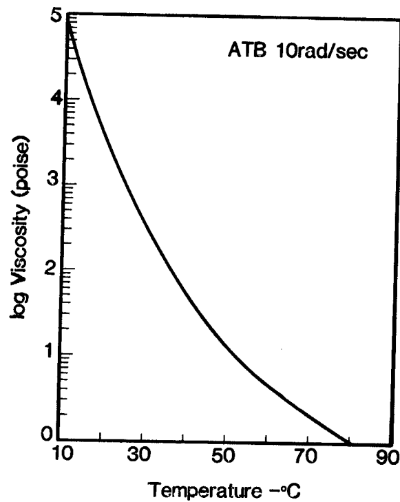
FIGURE 6. Viscosity of ATB.
