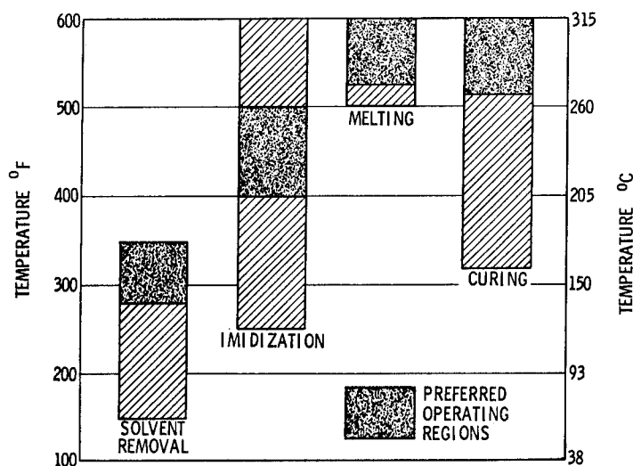
FIGURE 1 PROCESSING PARAMETERS FOR TYPICAL ADDITION PI
