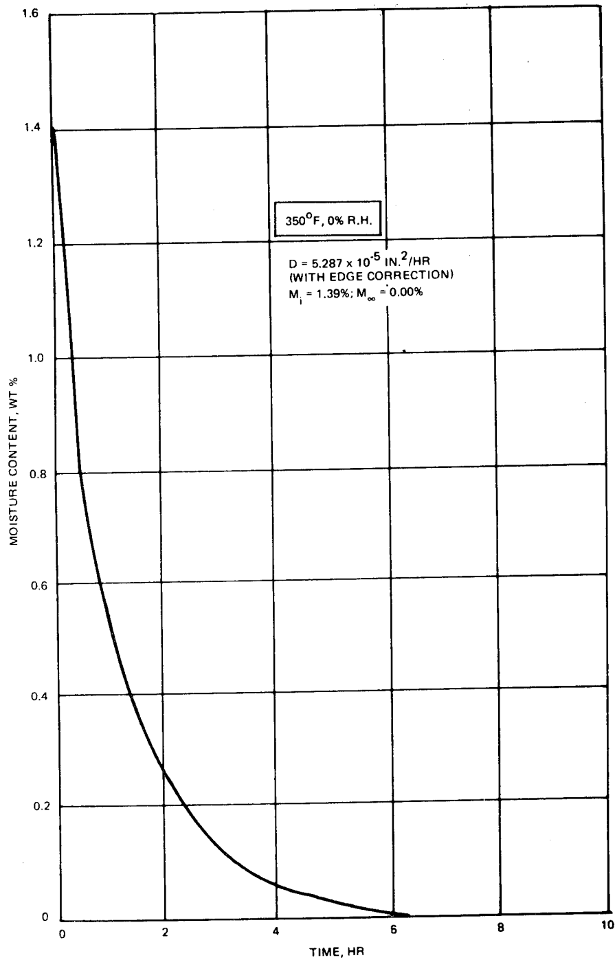
Figure 10. Projected moisture content time history for 16-ply graphite/polyimide specimens ( M_i = 1.39\% , M_\infty = 0.00\% )
