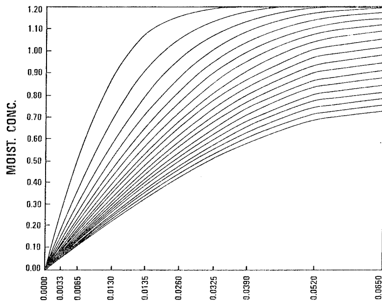
Figure 15. - Moisture concentration profile of a 4 ply specimen during thermal cycling.
