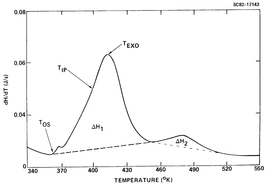
Figure 9. DSC thermogram for the curing of U.S. Polymeric V378A resin.
