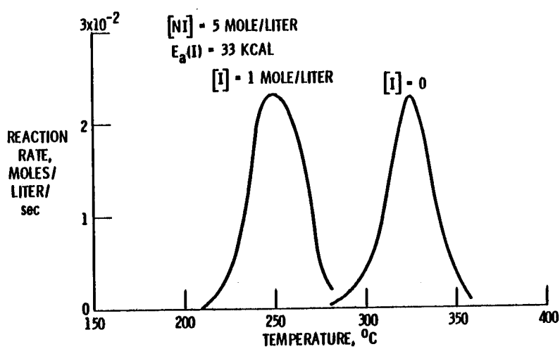
Figure 6. - Calculated effect of retarder on nadimide reaction rate.
