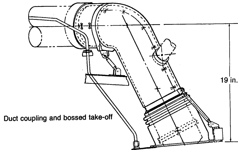
Figure 9. - 747 pneumatic duct.
