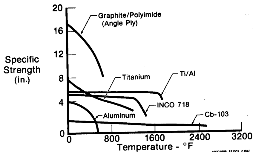
Figure 2. - Specific strength versus temperature.
