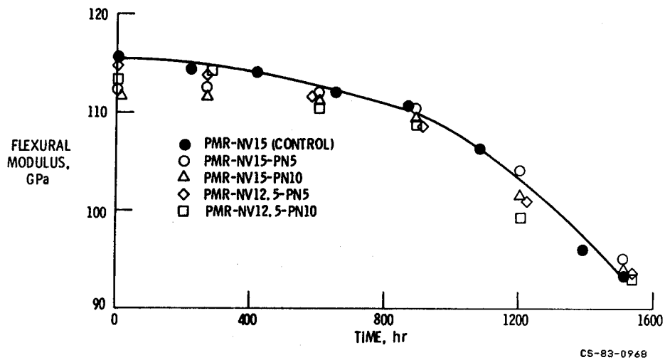
Figure 8. - Flexural modulus of Celion 6000 graphite fiber/PMR-NV polyimide composites exposed and tested in air at 316° C.
