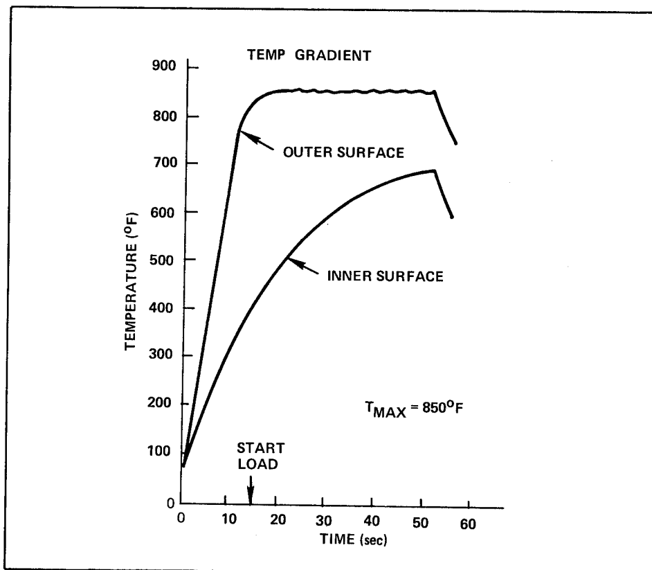
Figure 8 Transient temperature history for [0°] 20 coupons.
