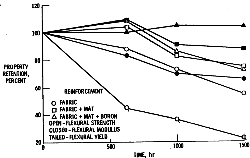
Figure 2. - Flexural properties of Celion 3000 graphite fabric/PMR-15 laminates exposed in air at 316 °C and tested at 288 °C.
