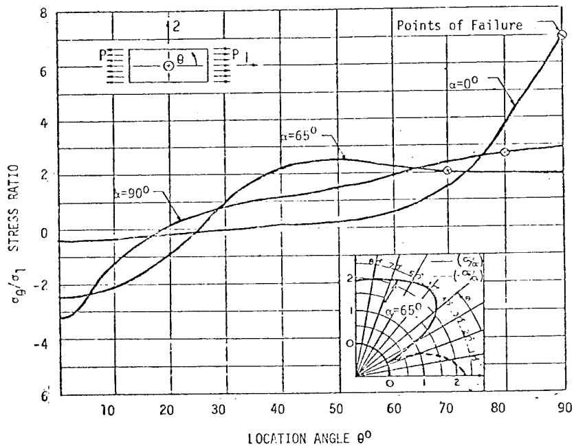
FIG. 5 STRESS DISTRIBUTION AT PERIPHERY OF HOLE, BORON EPOXY [+a/-a/-a/+a]
