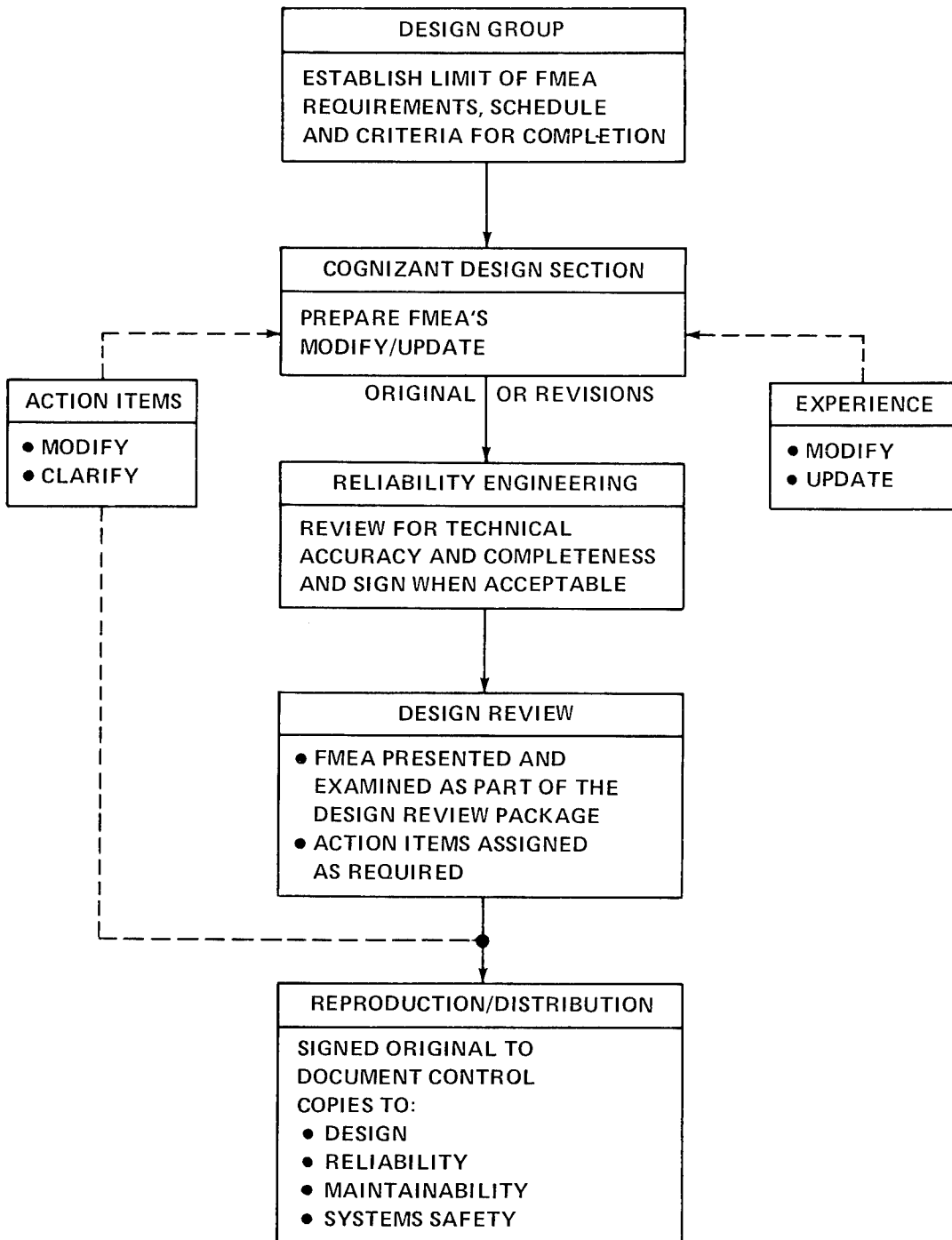
FIGURE 2. FMEA PROCEDURES FLOW CHART
