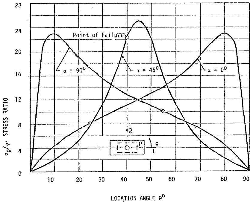
FIG. 10 STRESS DISTRIBUTION AT PERIPHERY OF HOLE IN SHEAR PANEL BORON EPOXY [+ \alpha /- \alpha /- \alpha /+ \alpha ]
