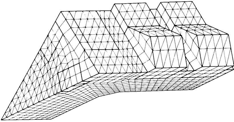
(c) Finite element idealization (tetrahedral elements)
