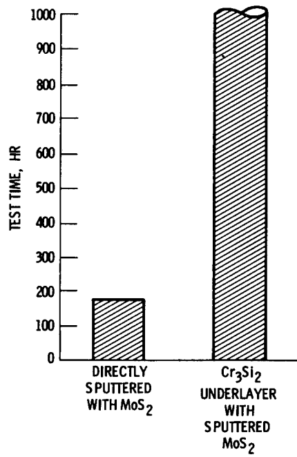
Figure 7. - Endurance lives of 440C stainless-steel ball bearings with sputtered MoS 2 films on races and cage - with and without a Cr 3 Si 2 underlayer.
