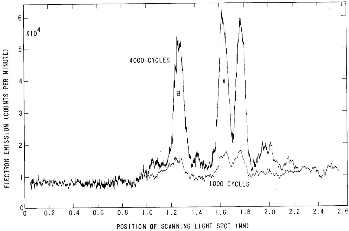
FIG. 3. Exoelectron emission from 1100 aluminum after 1000 and 4000 fatigue cycles. Fatigue life = 140,000 cycles.
