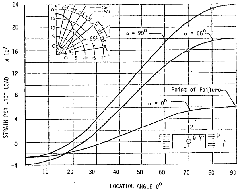
FIG. 7 STRAIN DISTRIBUTION AT PERIPHERY OF HOLE, BORON EPOXY [+ \alpha /- \alpha /- \alpha /+ \alpha ]
