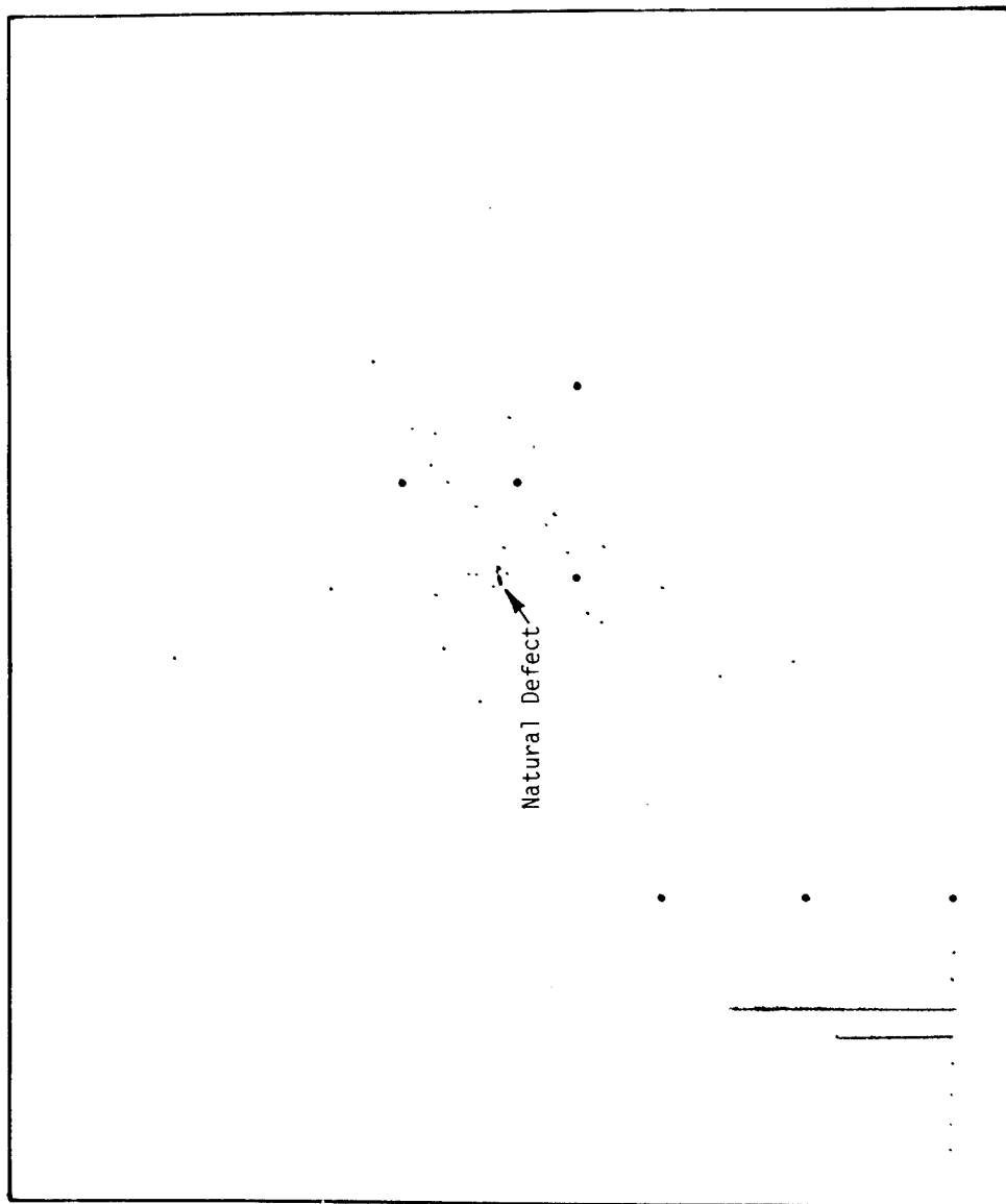
FIGURE 11. AE Sources Received from a Petrochemical Vessel Containing a 7.6 cm Crack - Early in Test
