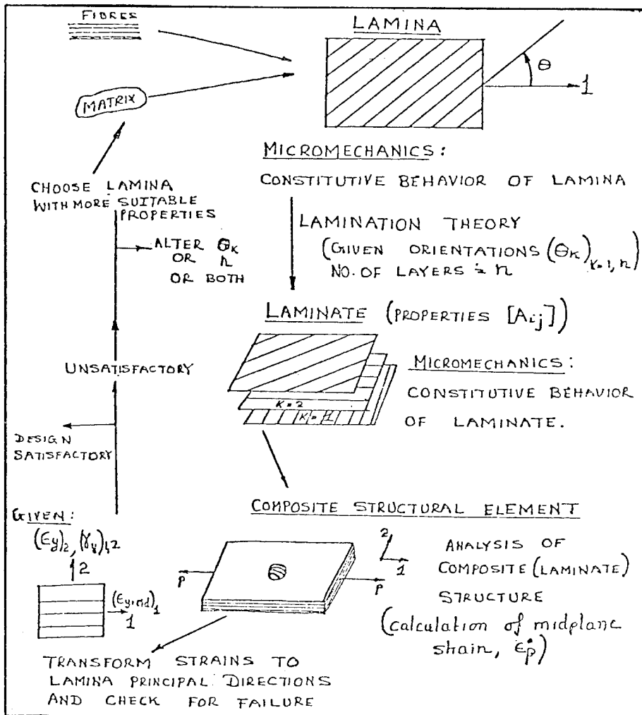
FIG. 1 DESIGN PROCEDURE FOR LAMINATED COMPOSITES
