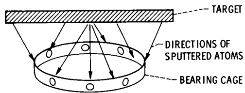
Figure 3. - Schematic of sputter coating complex surfaces.
