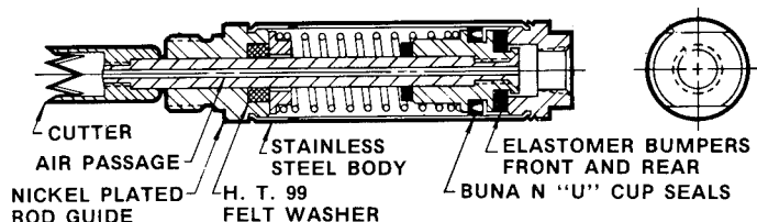
Figure 2. Cross-section showing internal construction of pneumatic cylinder designed for punching holes in plastic film.
