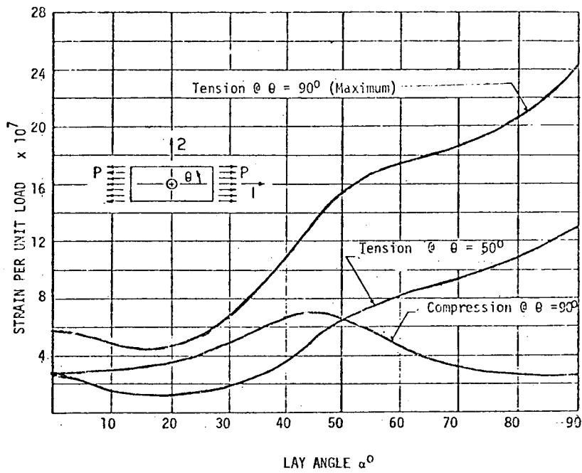
FIG. 6 TANGENTIAL STRAIN VS. LAY ANGLE, BORON EPOXY [+ \alpha /- \alpha /- \alpha /+ \alpha ]
