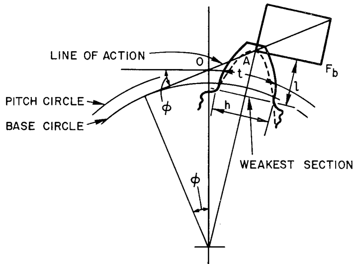
Figure 1. Beam Model of Gear Tooth
