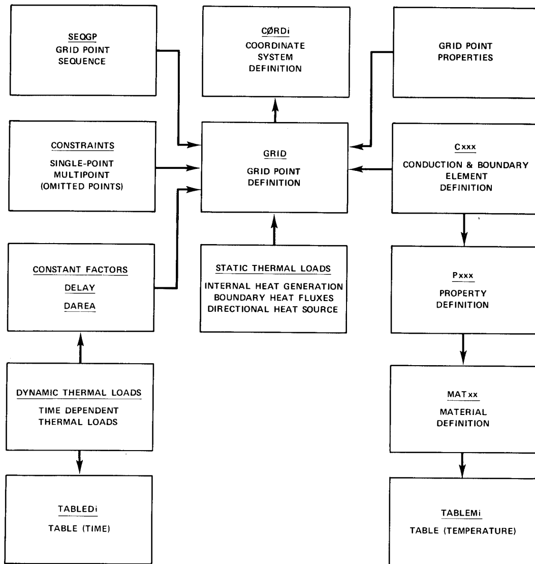
Figure 5. Functional diagram of the \bar{N}TA thermal model.
