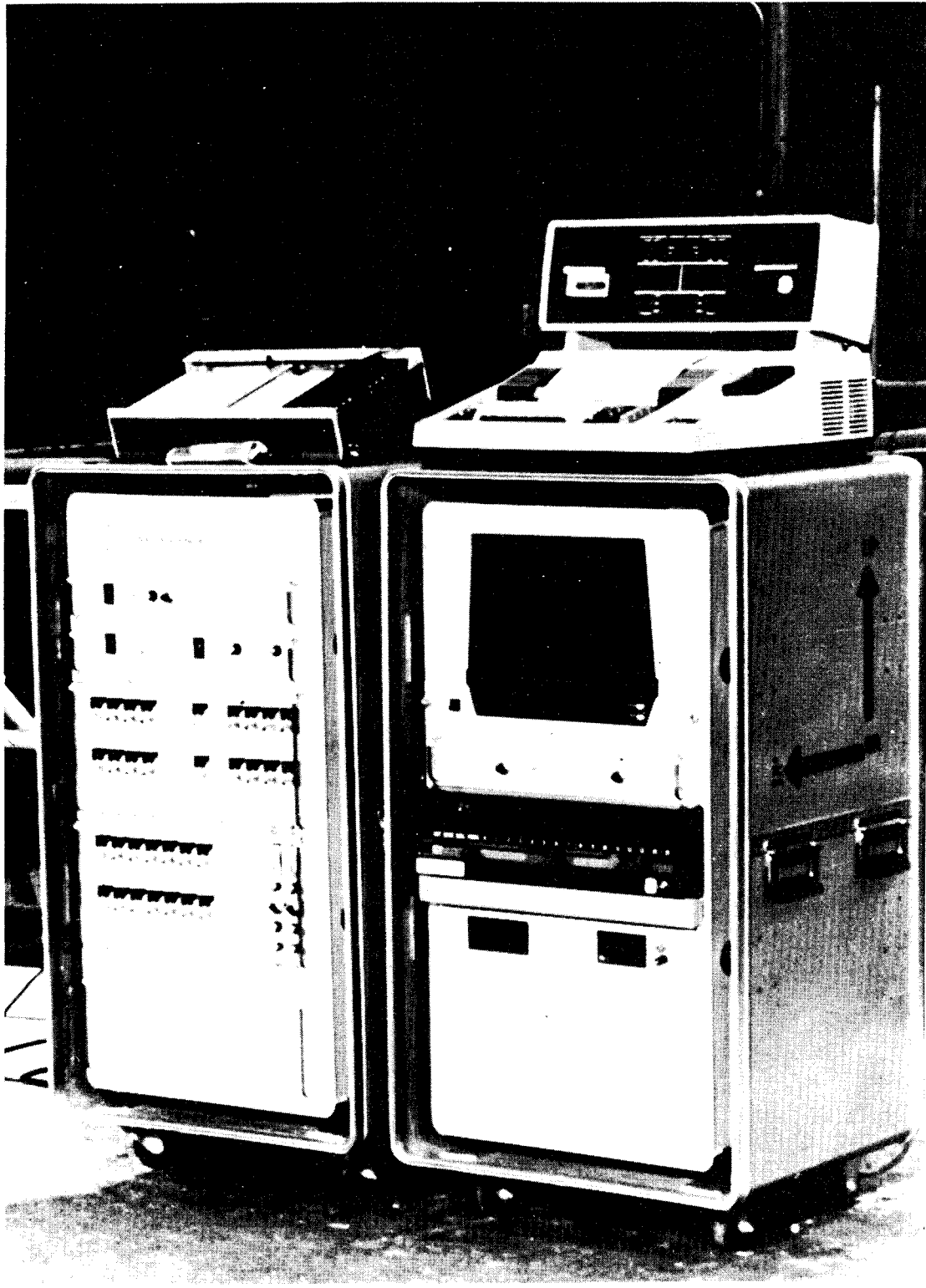
FIGURE 1. Portable Source Location System
