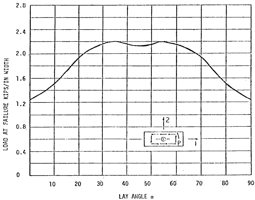
FIG. 11 LOAD CAPACITY OF PANELS IN SHEAR, BORON EPOXY [+ \alpha /- \alpha /- \alpha /+ \alpha ]
