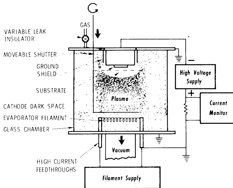
APPARATUS FOR ION PLATING
