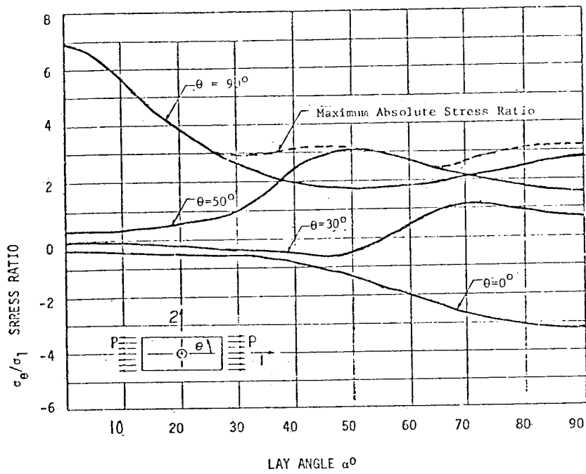
FIG. 4 MAXIMUM STRESS VS. APPLIED STRESS, BORON EPOXY [+a/-a/-a/+a]
