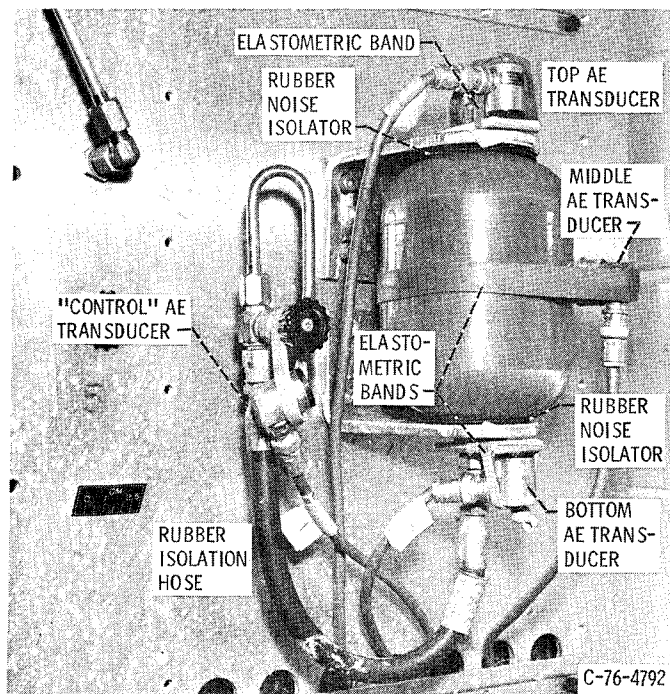
Figure 2. - View of Kevlar 49/epoxy composite vessel mounted in test fixture.
