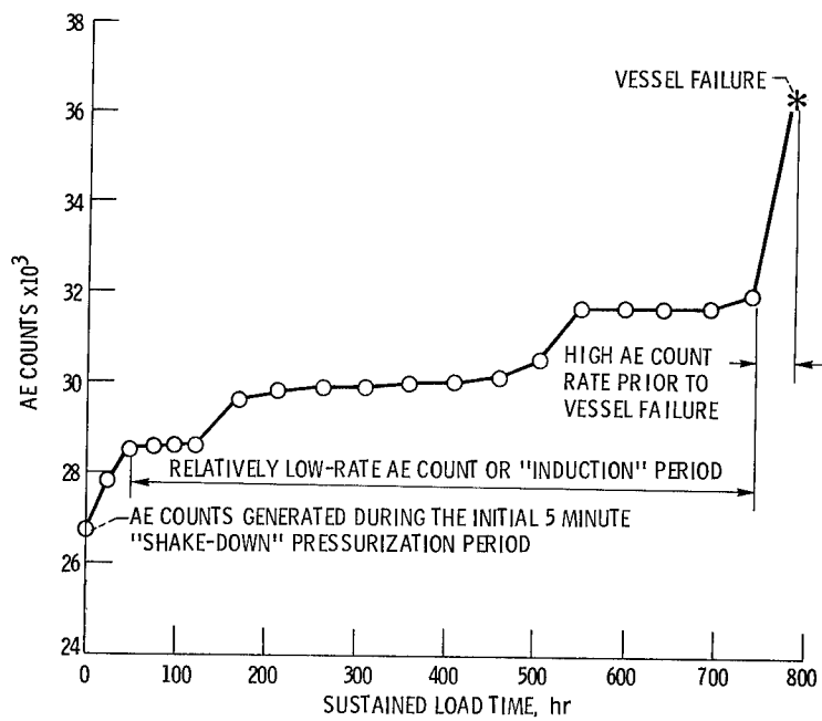
Figure 7. - Summation of AE counts vs sustained load time for vessel K-39.
