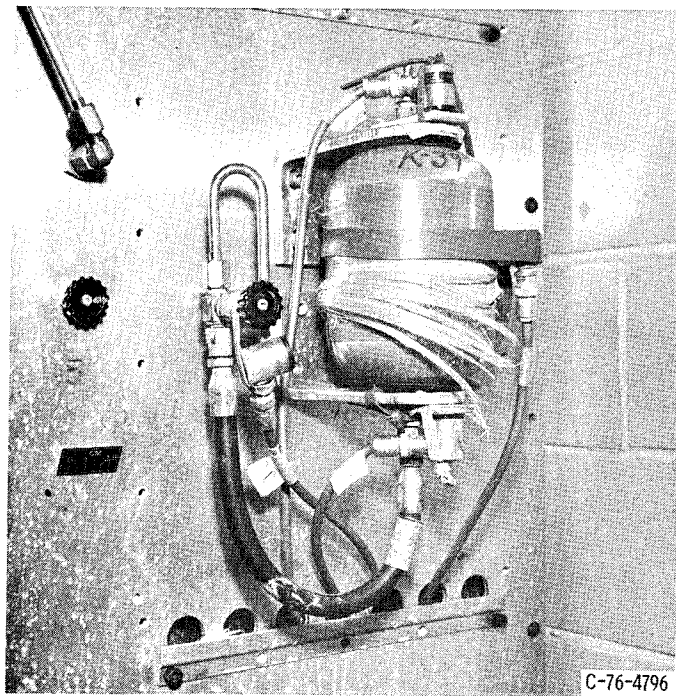
Figure 6. - View of typical vessel after failure.
