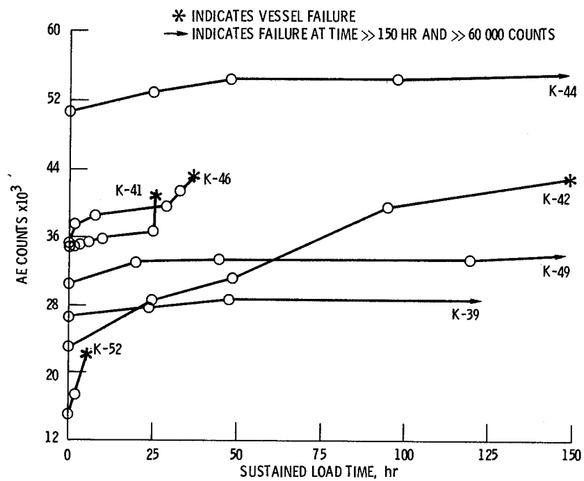
Figure 14. - Summation of AE counts vs sustained load time for all vessels.
