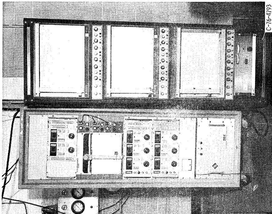
Figure 4. - Acoustic emission data conditioning and recording apparatus.
