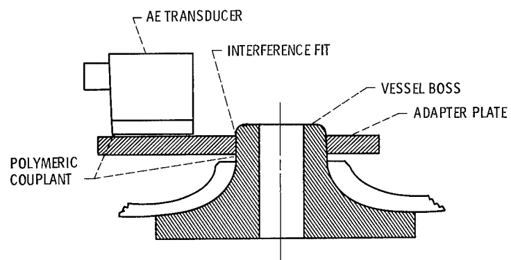
(b) CROSS SECTIONAL VIEW OF ADAPTER PLATE FASTENED TO VESSEL BOSS.
