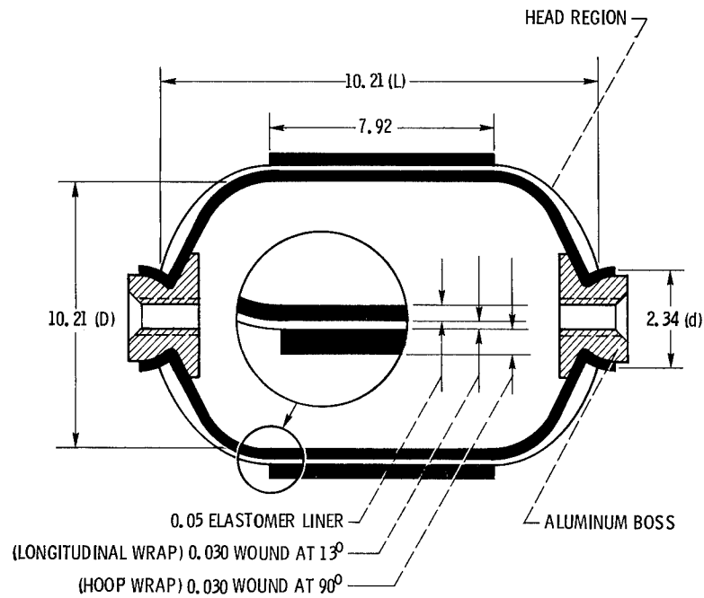
Figure 1. - Design of the 10.16 centimeters (4 in.) diameter Kevlar 49/epoxy composite pressure vessel. (Dimensions are in centimeters.)
