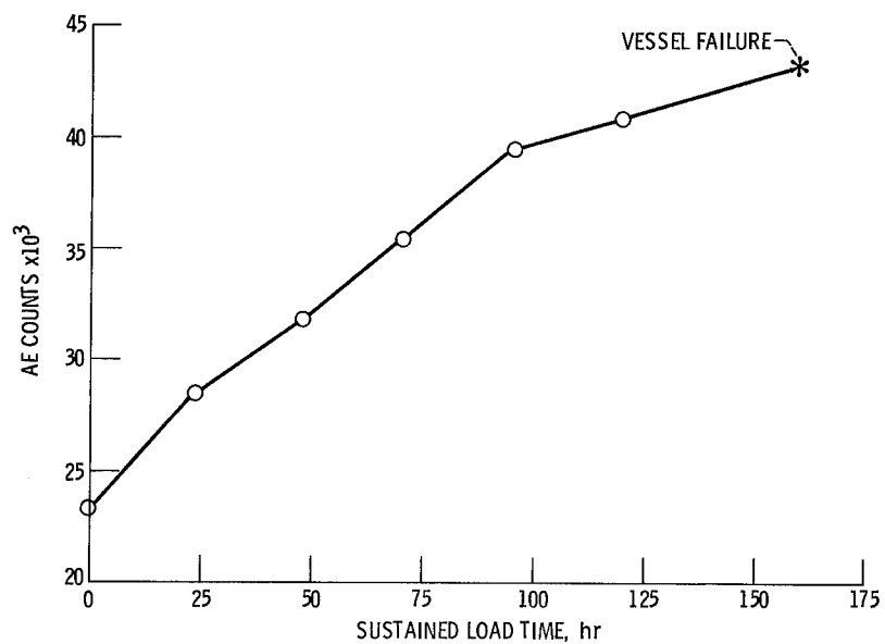
Figure 9. - Summation of AE counts vs sustained load time for vessel K-42.
