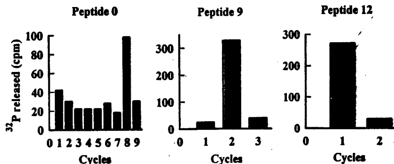
Fig. 2. Identification of the Position of the Phosphoamino Acids by Manual Edman Degradation
