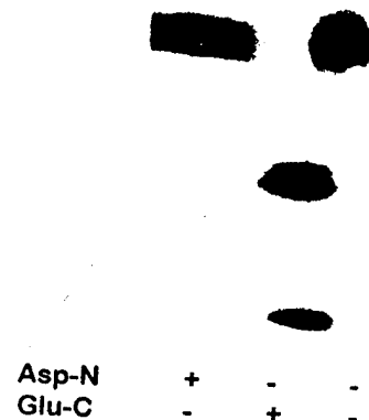
Figure 6. Characterization of peptide 5 by specific protease digestion
