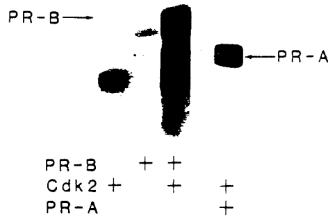
Figure 7. In vitro phosphorylation of PR by Cdk2
