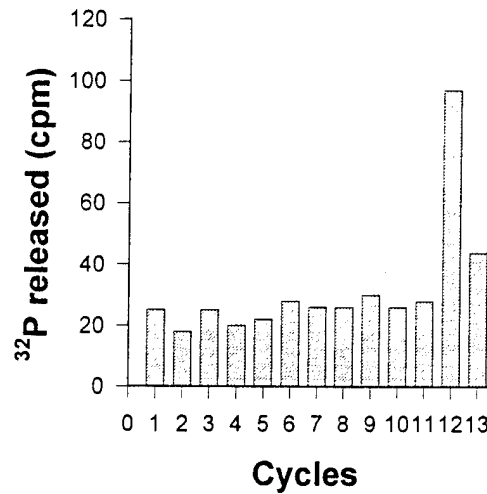
Figure 5. Phosphate release analysis of peptide 5
