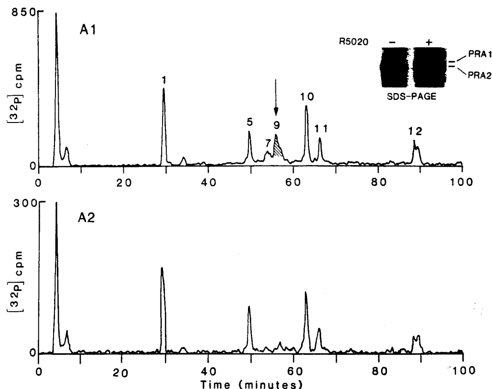
Fig. 5. Identification of Ser 345 as the Phosphorylation Site Associated with Altered Mobility of PR
