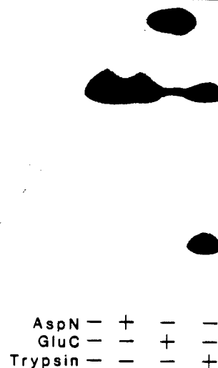
Figure 3. Characterization of phosphopeptide 2 by redigestion with additional proteases
