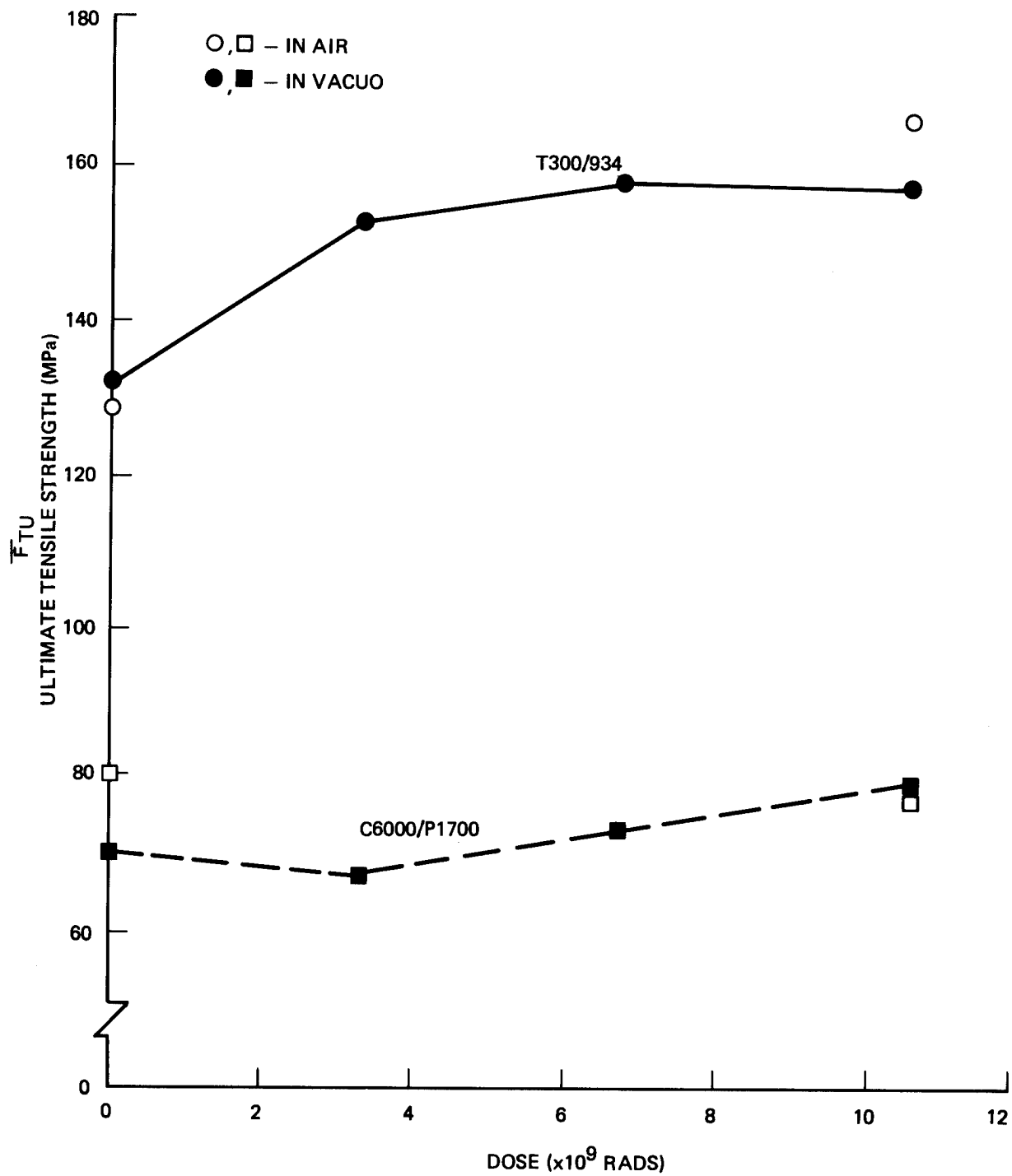
Figure 6-4. Effect of Radiation on Ultimate Tensile Strength, T300/934 and C6000/P1700 [±45/∓45] Laminate Composite Materials.
