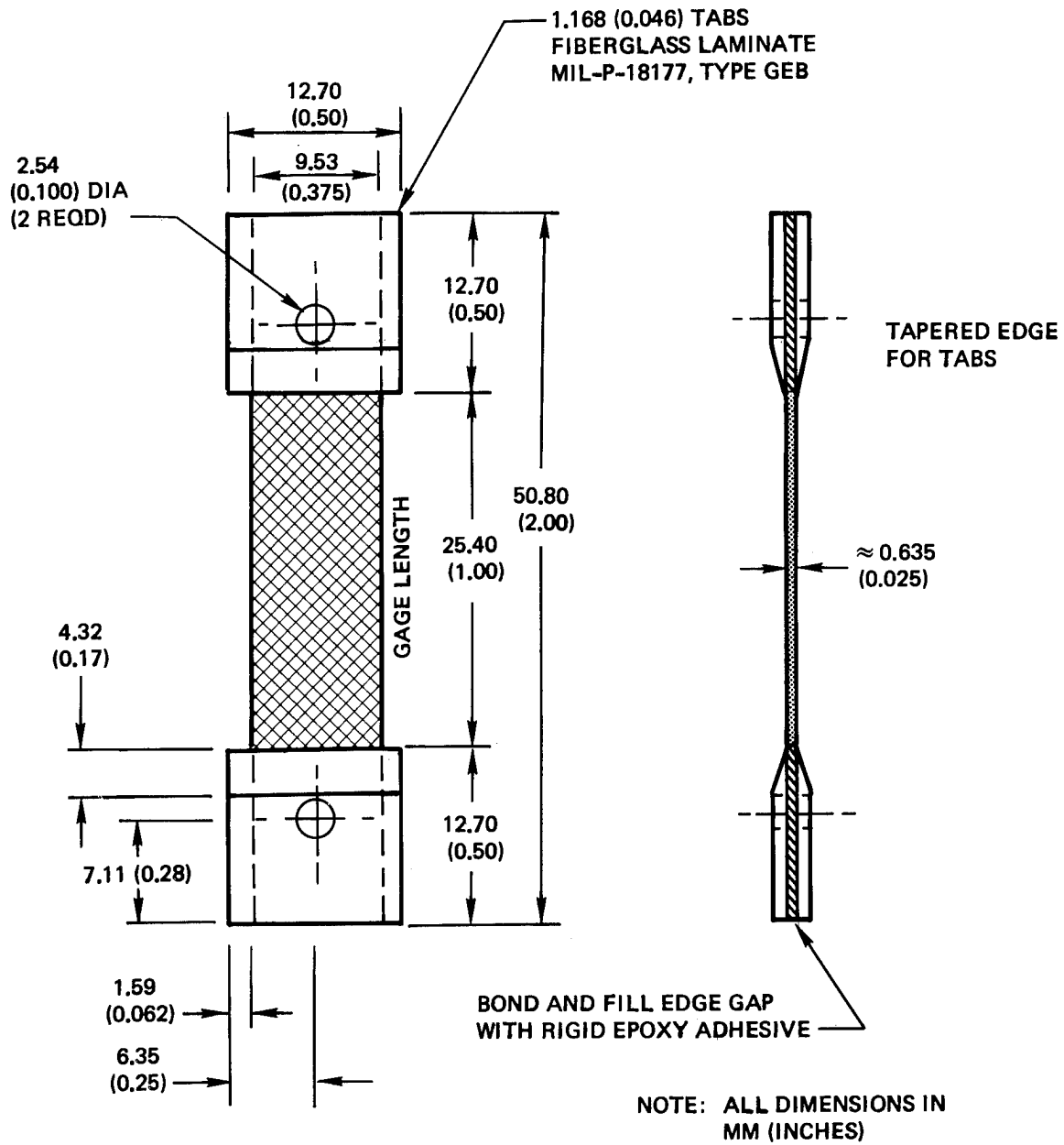
Figure 3-2. Test Specimen Dimensions.
