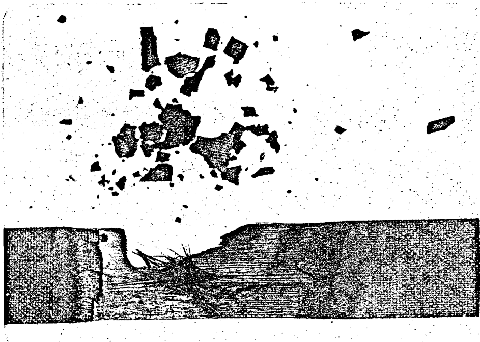
FIGURE 11. SAMPLE AND EJECTA OF PANEL EK2 (KYNOL FACED PANEL)
