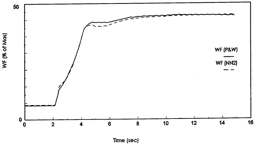
Figure 6. Simulator vs. NN2 Estimated WF at Transient Condition
