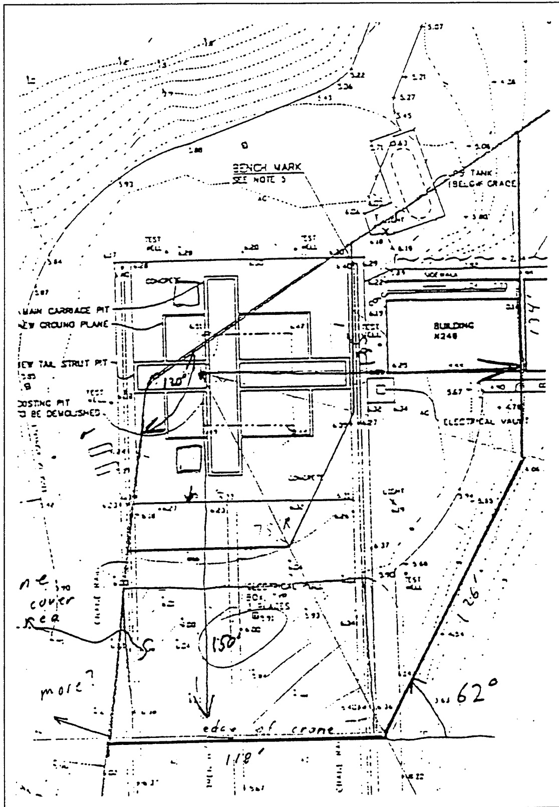
Figure 5 Proposed Wall Configuration at NASA's OARF
