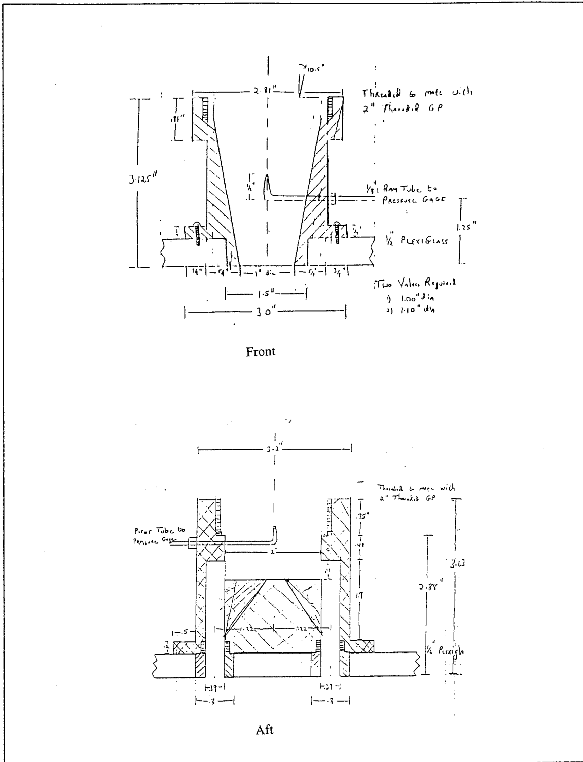
Figure 3 0.39" and 1" Nozzle Design
