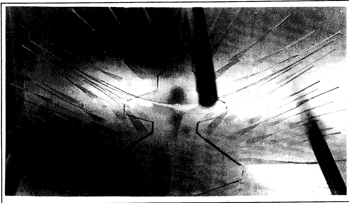
Figure 14 Large Stagnation Point ( NTR = 4.9 h/De = 15 )
