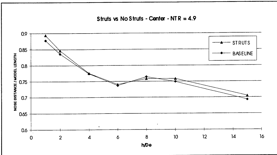
Figure 17 Stagnation Point Location for NTR = 4.9
