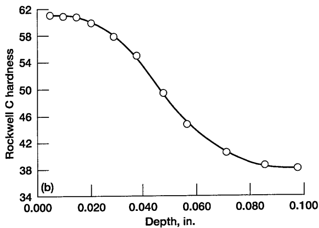
Figure 5.—Hardness profile of AISI 1552 steel test gear contour hardened case and a carburized and hardened AISI 9310 gear. (a) AISI 1552 gear. (b) Carburized and hardened AISI 9310 gear.
