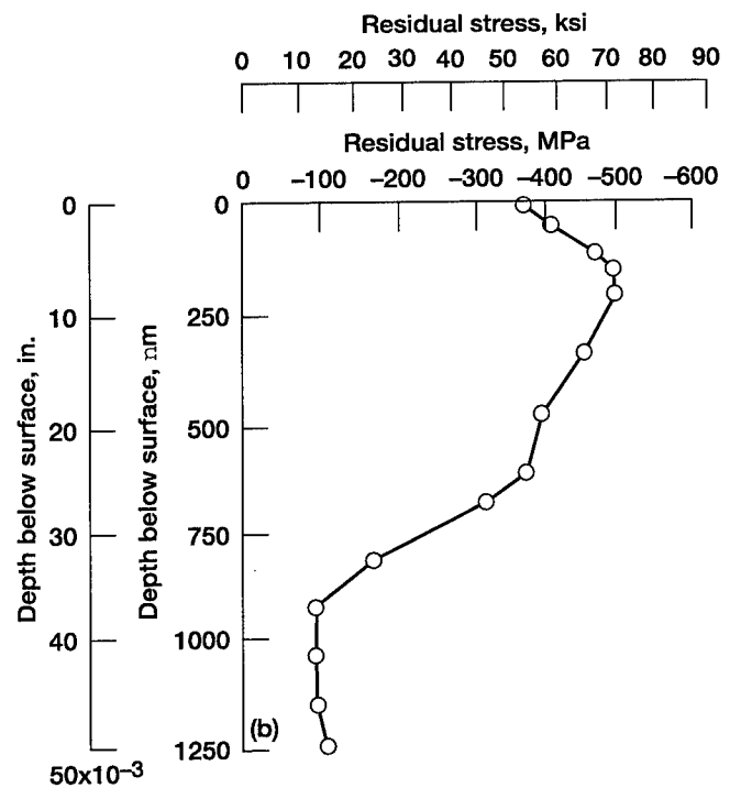
Figure 6.—Residual stress versus depth for carburized, hardened and ground AISI 9310 test gears and dual frequency induction hardened AISI 1552 gears. (a) AISI 9310. (b) AISI 1552.
