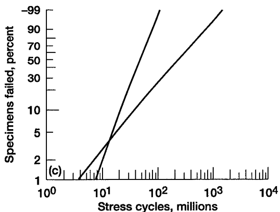
Figure 7.—Surface fatigue lives of surface hardened AISI 9310 and AISI 1552 test gears. Speed 10 000 rpm; maximum Hertz stress, 1.71 GPa (250 ksi); temperature, 350 K (170 °F); lubricant, synthetic paraffinic with 5-percent by volume EP additive. (a) AISI 9310. (b) AISI 1552. (c) Summary.
