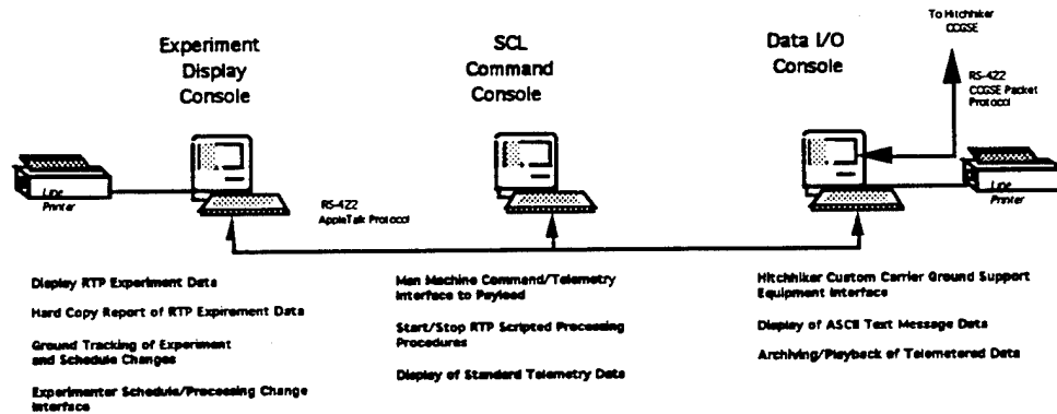
FIGURE 4. Requirement Mapping of Ground Station Subsystems.
