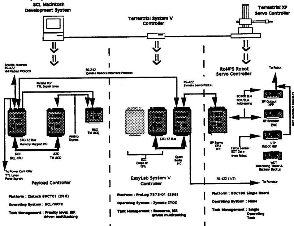
FIGURE 2. Migration of Terrestrial Architecture to a Space-Hardened Architecture.
