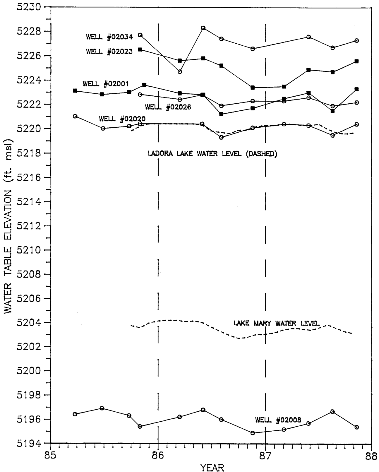
Figure 2.4-28 LAKE AND WELL LEVELS BY LAKES LADORA AND MARY
