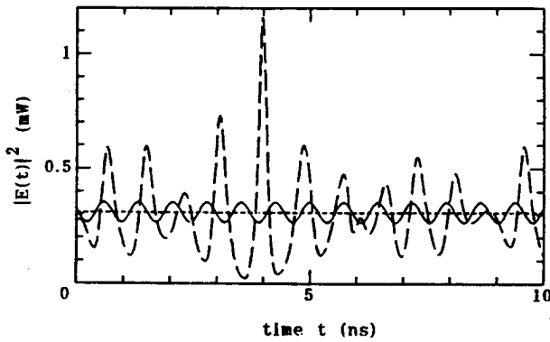
Fig. 2 Numerical results for J=1.07 J_{th} , L_1=30 cm, and R_1=1.5\% . Broken line: single feedback; Dotted line: L_2/L_1=0.925 , R_2/R_1=1/3 ; Solid line: L_2/L_1=0.925 , R_2/R_1=2/3 .
