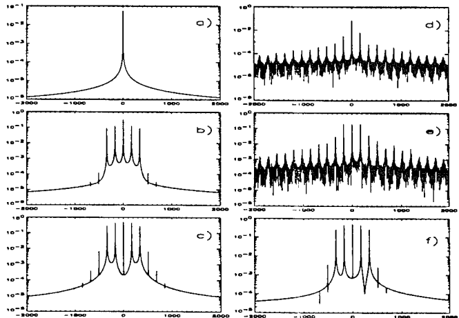
Figure 1 FPS (log scale, frequency in GHz). Pump values: (J/J_{th}) = 1.02(a, d), 1.7(b, e), 3.5(c, f) . Spontaneous emission noise: \beta = 0 (left column: a, b, c), \beta = 10^{-4} s^{-1} (right column: d, e, f). \delta = 0 , D = 0 .
