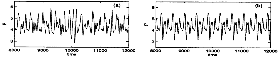
Figure 1: Time evolution of the output power P of a multi-transverse mode laser before (a) and after (b) the application of the control signals.
