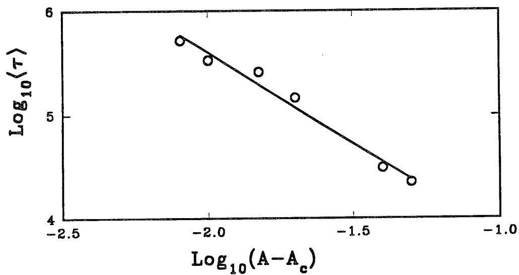
Figure 2 Critical exponent \gamma = \log_{10}\langle \tau \rangle / \log_{10}(A - A_c)
