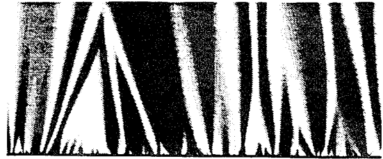
Figure 4: Space-time plot of the modulus of A_x in gray levels (white=maximum amplitude) from t = 0 to t = 2000 . Model Parameters as in Fig. 1. The system size is 4096 and the initial condition is Gaussian-noise with a mean squared amplitude equal to 0.001.
