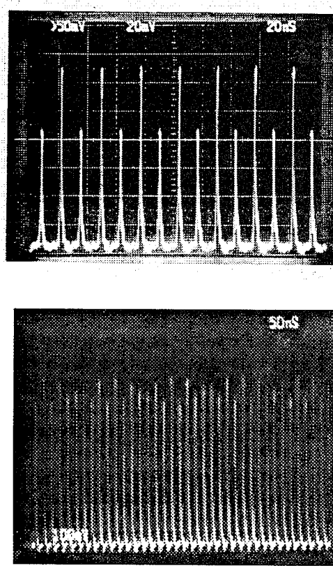
Figure 1. Period-doubled pulse train (a) and quasiperiodic pulse train (b) from APM laser. Note that pulse spacing is 13 nsec in both traces.
