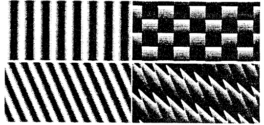
Figure 1: Space-time plot of the modulus (left) and the phase (right) of the amplitude A_x for a standing wave with K = 0.7 and d = 0.098 (top) and a depolarized solution K = 0.074 and d = 0.123 (bottom). The horizontal axis represents space and the vertical axis time. The maximum of the modulus has been scaled to white and the phase ranges from 0 (white) to 2\pi (black). The parameters are: \mu = 0.2 , \alpha = 2.6 , \beta = 0.2 , \delta = -0.25 ; the system size is 512 and the last plotted time is 300 time units.
