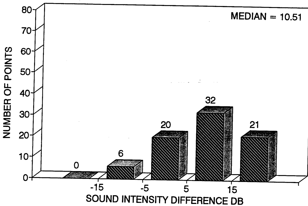
Figure 4. NAPS and microphone measurement predicted frequency distribution of sound intensity differences for trials matched with early meteorological data (top) and the 5-lb trials (bottom).
