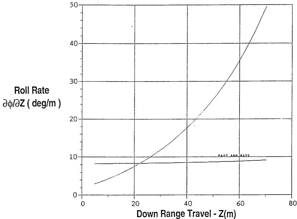
Figure 19. Vehicle roll rate vs. range (round no. 20447).
