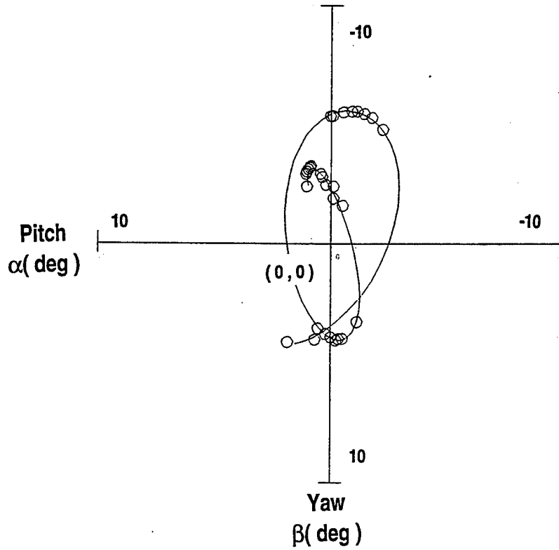
Figure 11. Pitch vs. yaw (round no. 20448).
