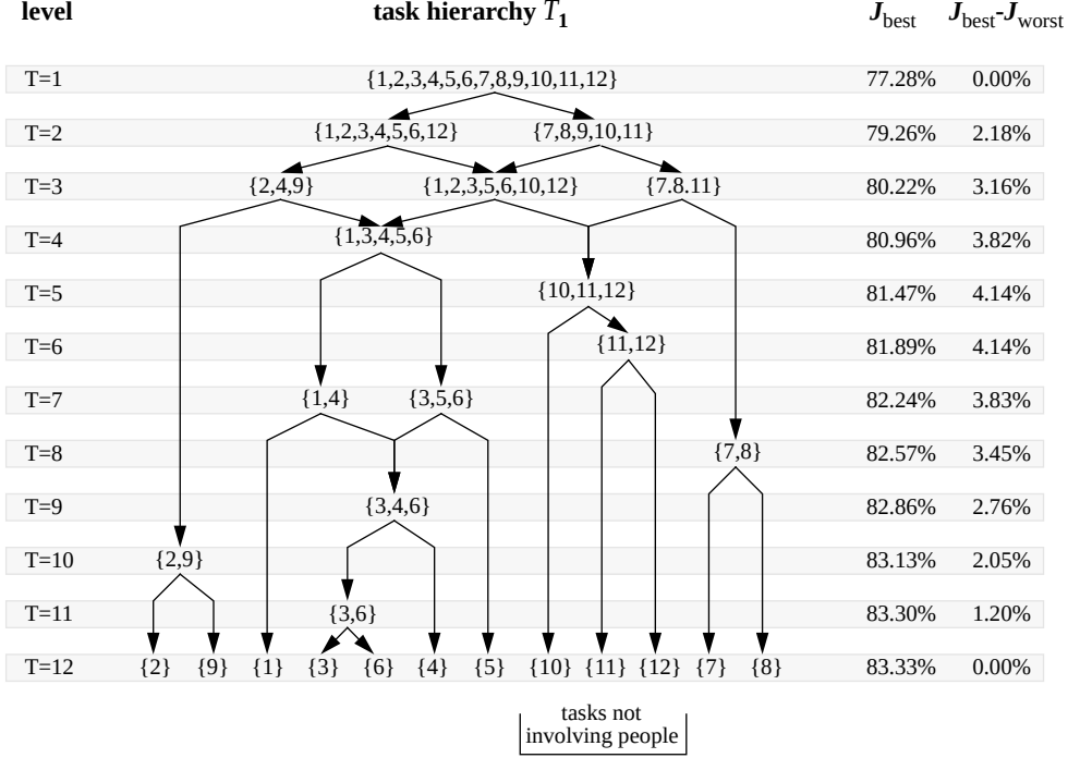
Figure 8: The task hierarchy for task family \mathcal{T}_1 . The hierarchy is obtained by clustering the task space using different numbers of clusters T . The right part of the diagram depicts the corresponding value for J , and the difference between the best and the worst partitioning.
