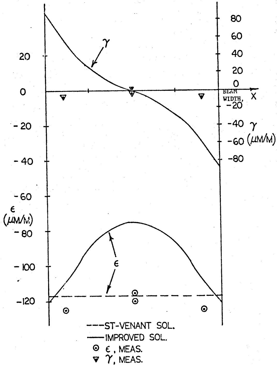
Figure IV-A-5. Strain Distributions Across the Beam Width, Near Center Span ( z/L = 0.45 ), in the Upper Panel of the Balanced Beam Under 500 Newton Center Load.
