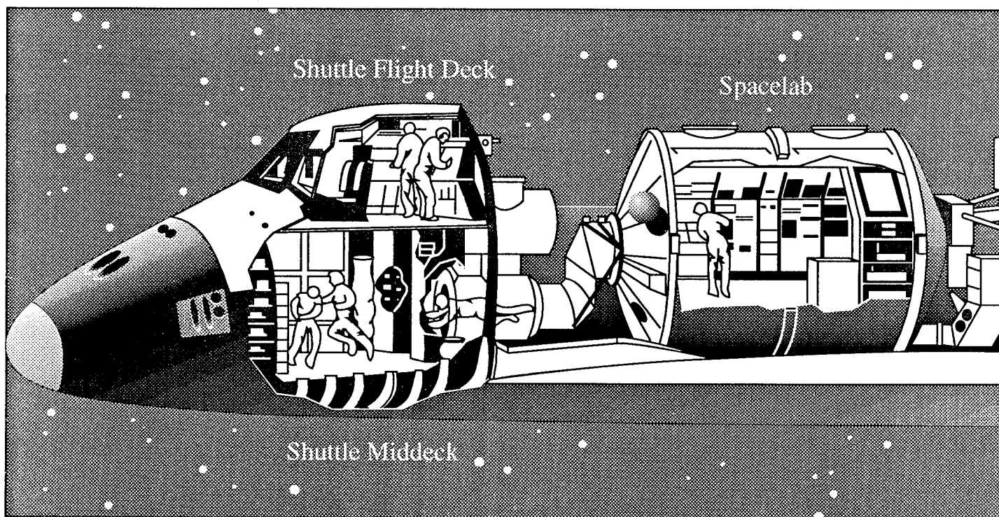
Figure 1: Spacelab in Space Shuttle Payload Bay
