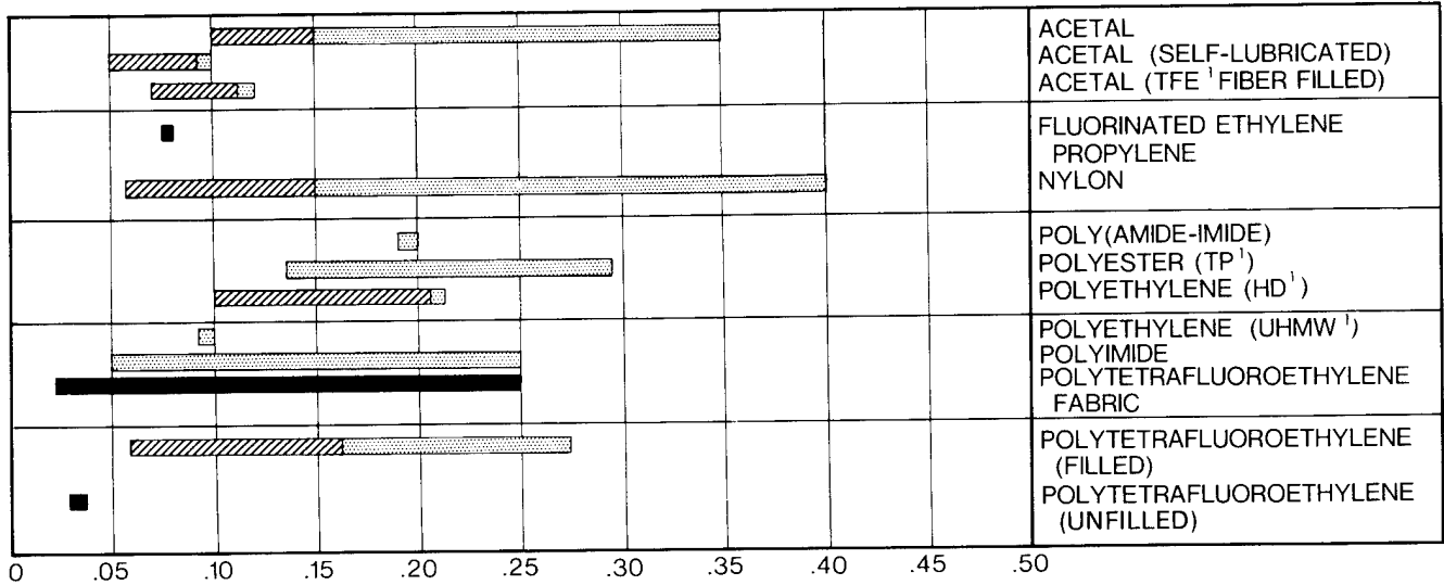
CHART 6. COEFFICIENT OF FRICTION
