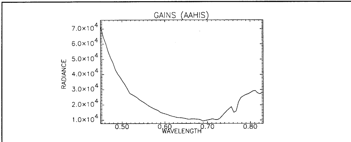
Figure 5.3 (AAHIS Gains)
