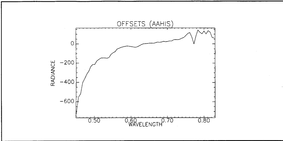
Figure 5.2 (AAHIS Offsets)
