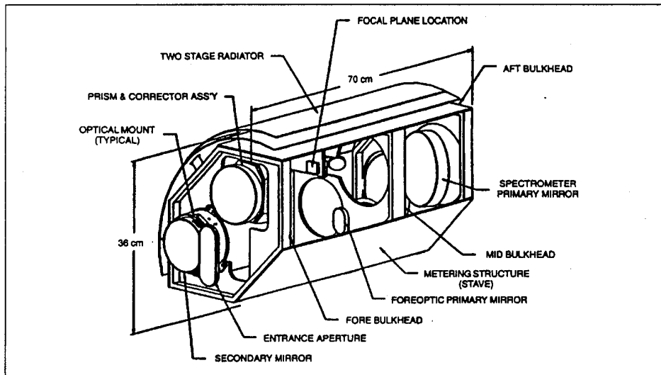
Figure 2.21 (HYDICE spaceborne concept, Silvergate, et al, 1994)
