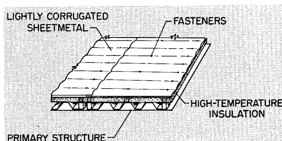
FIGURE 73-9.—Heat-shield concept.
