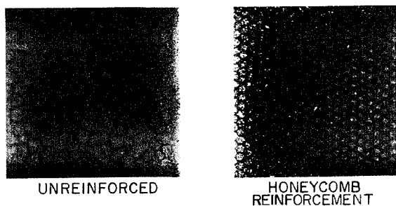
FIGURE 74-11.—Low-heating-rate problems.
