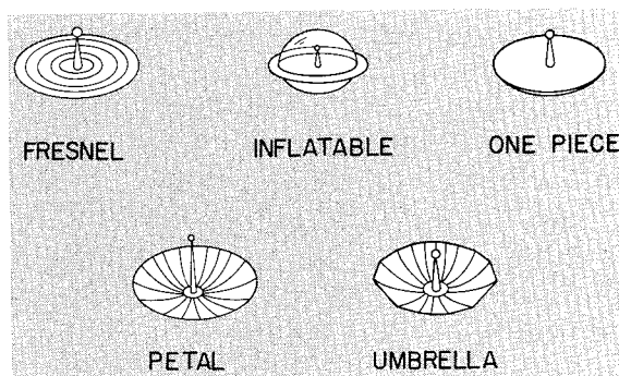
FIGURE 75-15.—Types of solar collectors.
