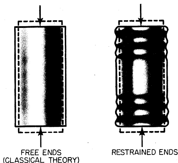
FIGURE 72-3.—Prebuckling state of axially compressed cylinders.
