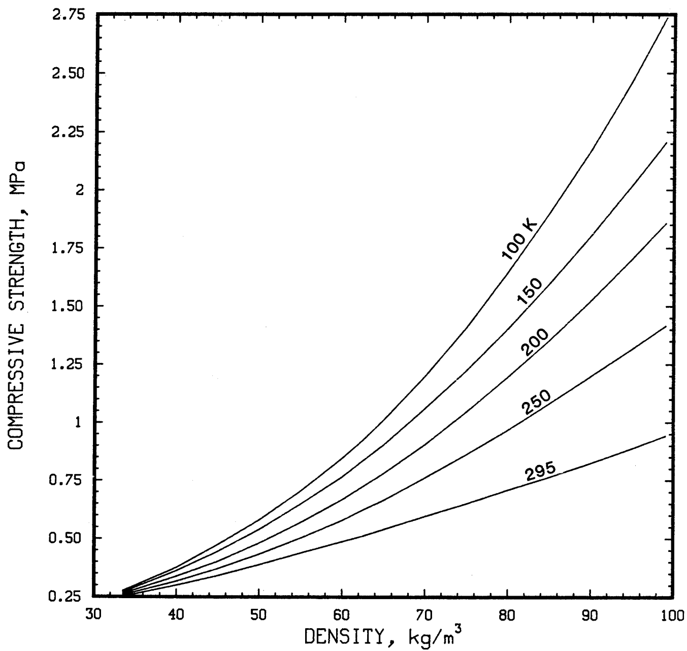
Figure 48. Compressive strength of polyurethane foam as a function of density with temperature as the parameter. The strength obtained here must be modified by a function of (H/W) for a particular material.
