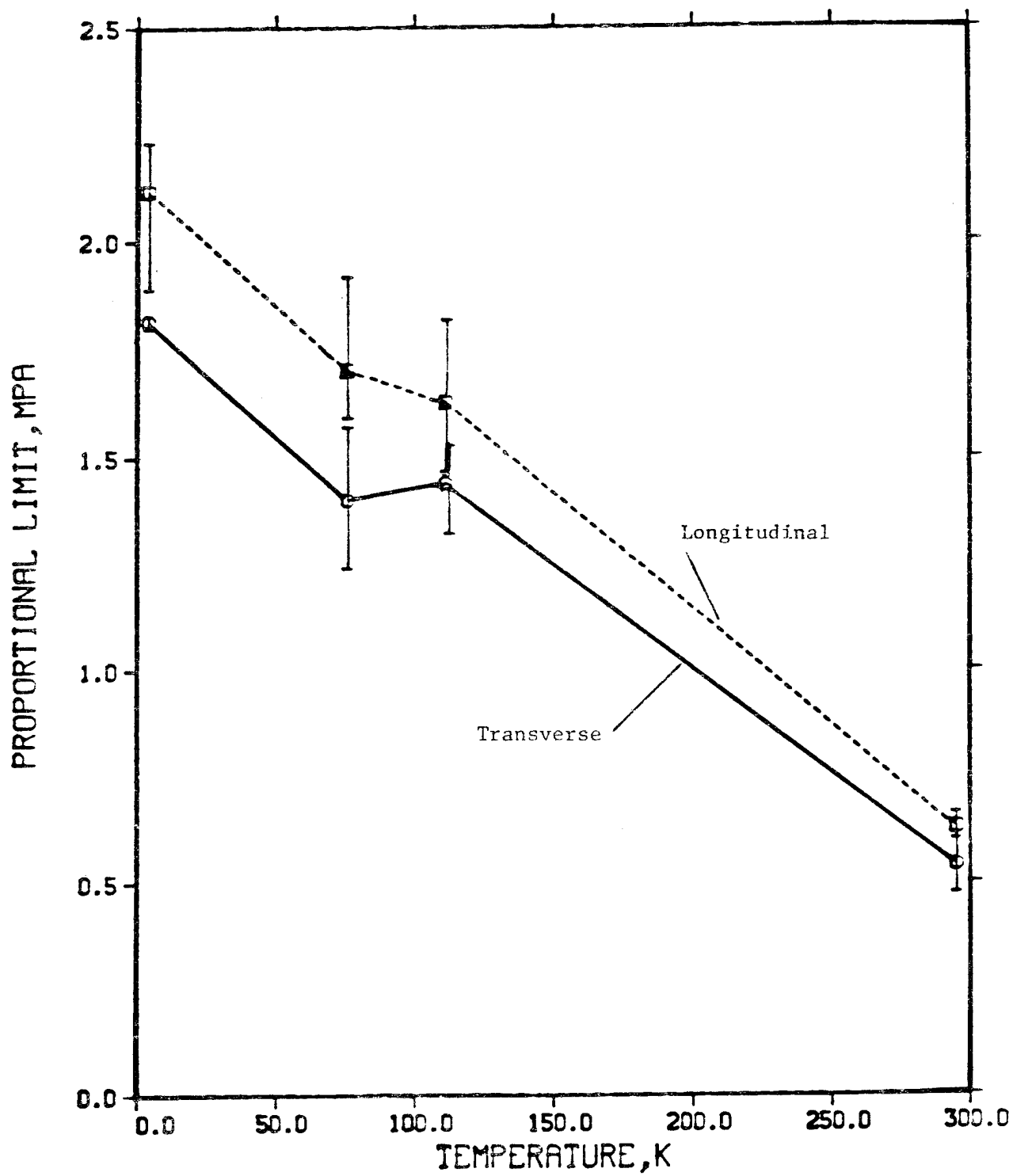
Figure 36. Compressive proportional limit versus temperature for a 96-kg/m 3 polyurethane foam.
