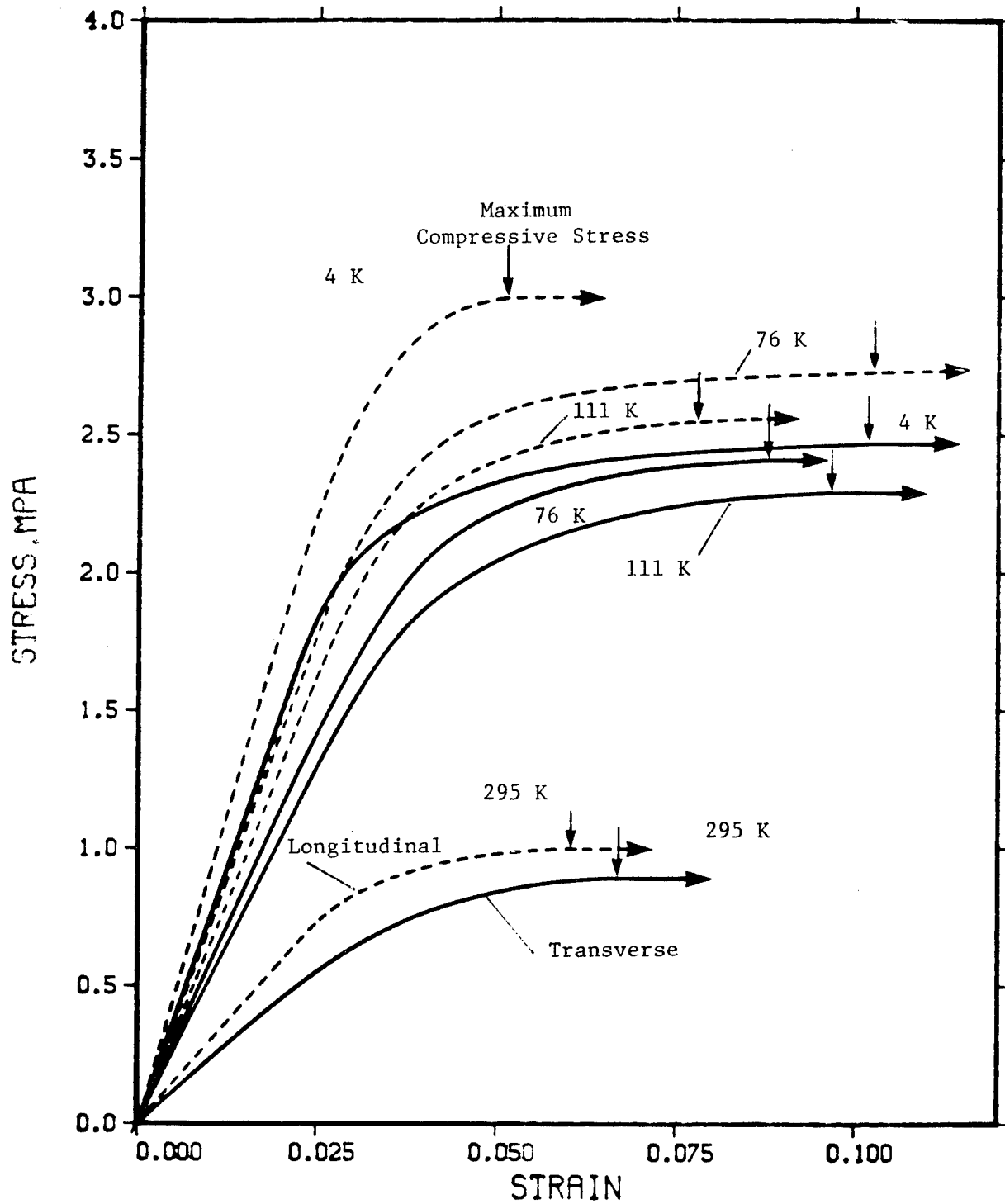
Figure 39. Compressive stress versus strain for a 96-kg/m 3 polyurethane foam.
