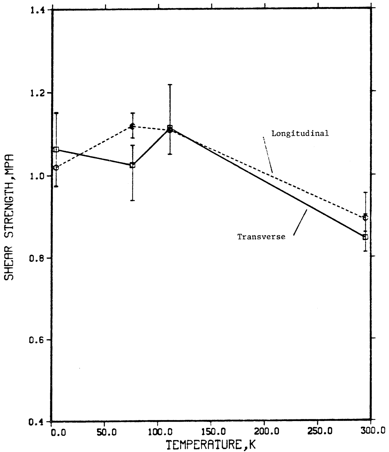
Figure 40. Shear strength versus temperature for a 96-kg/m 3 polyurethane foam.
