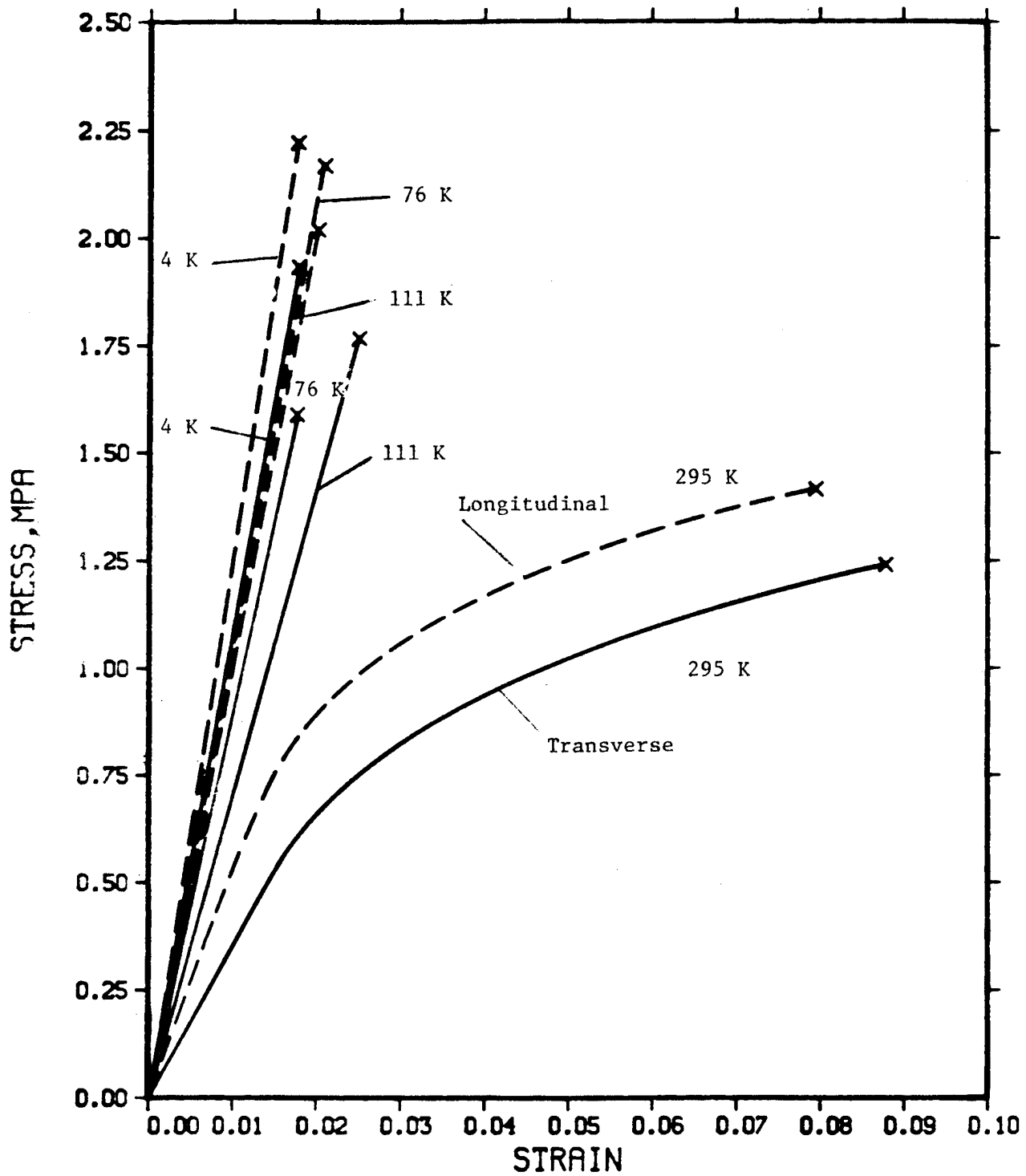
Figure 33. Tensile stress versus strain for a 96-kg/m 3 polyurethane foam.
