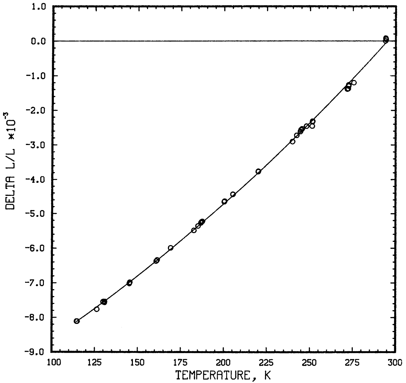
Figure 11. Thermal expansion of a 54-kg/m 3 polyurethane foam specimen. Experimental data are represented by discrete points and the solid line represents a three-term polynomial fit to these data. The reference temperature is 295.180 K
