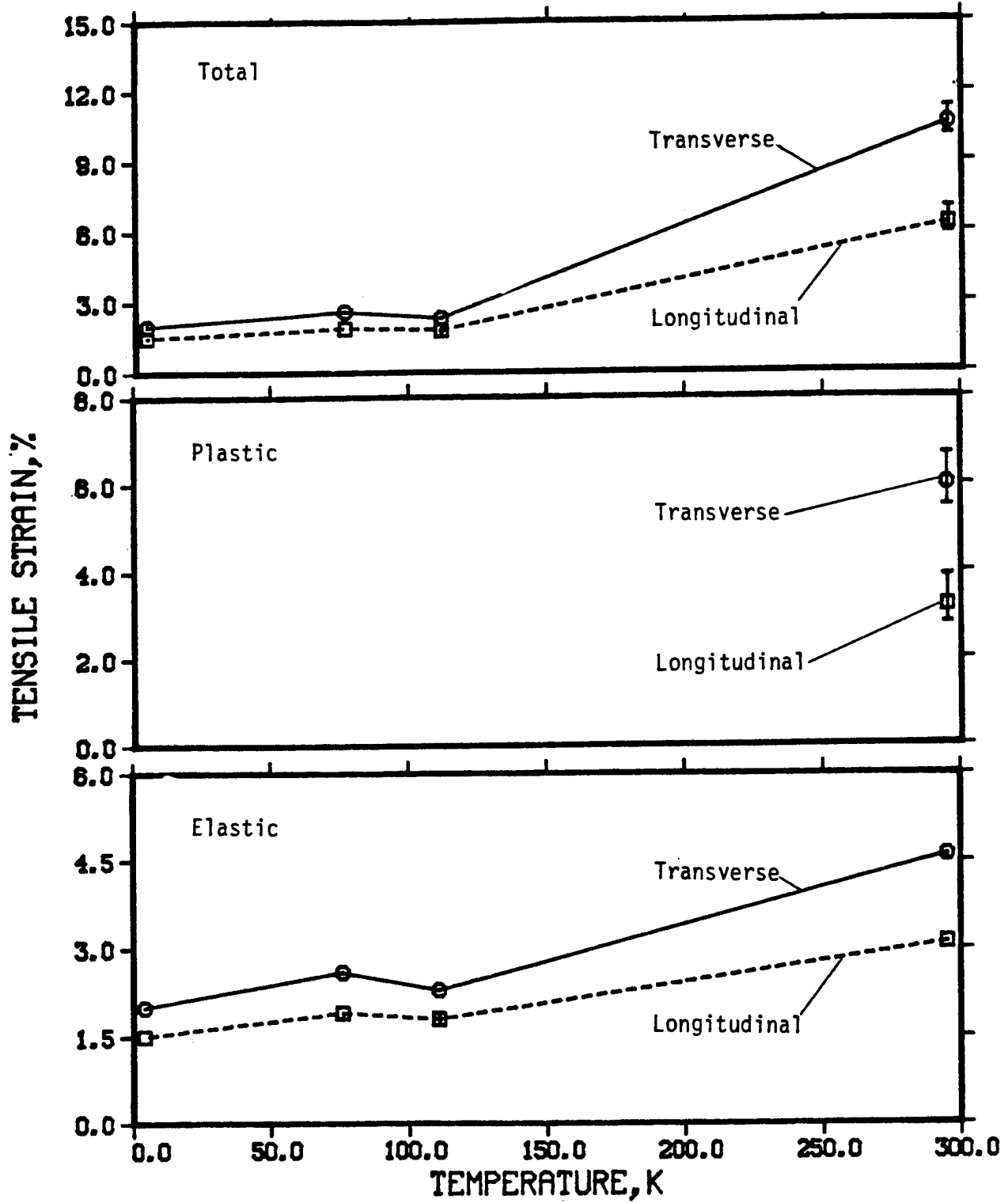
Figure 25. Tensile strain versus temperature for a 64-kg/m 3 polyurethane foam.
