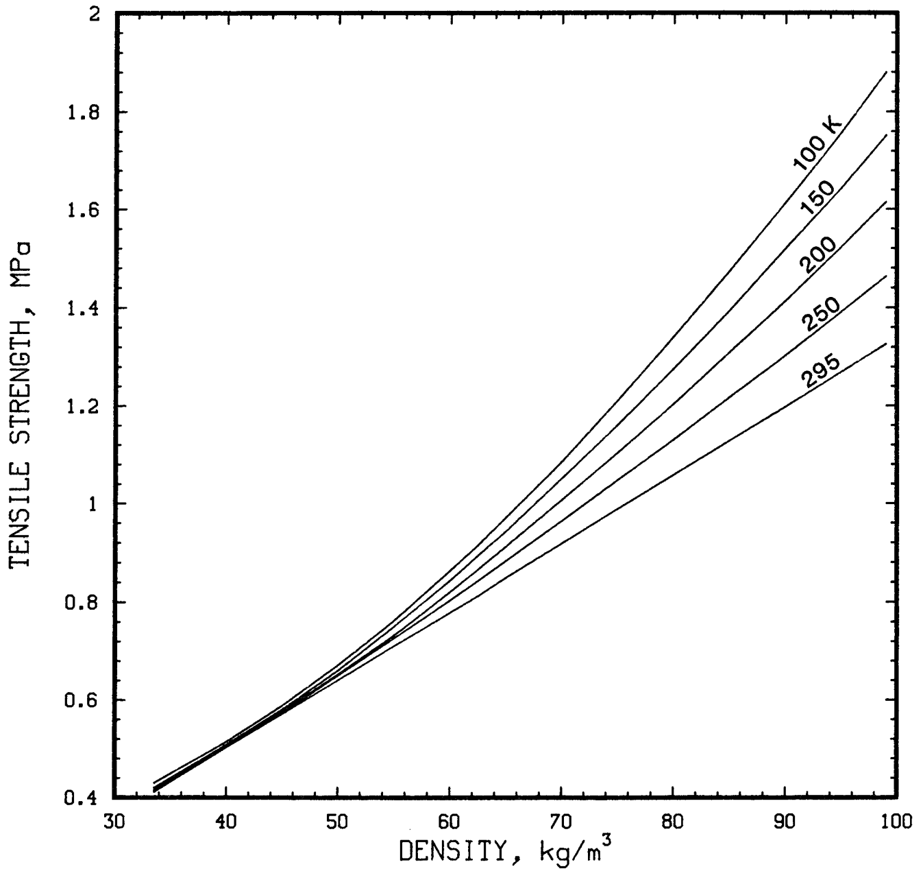
Figure 46. Strength of polyurethane foams in tension as a function of density with temperature as the parameter. Strength obtained here must be modified by a function of (H/W) for a specific material.
