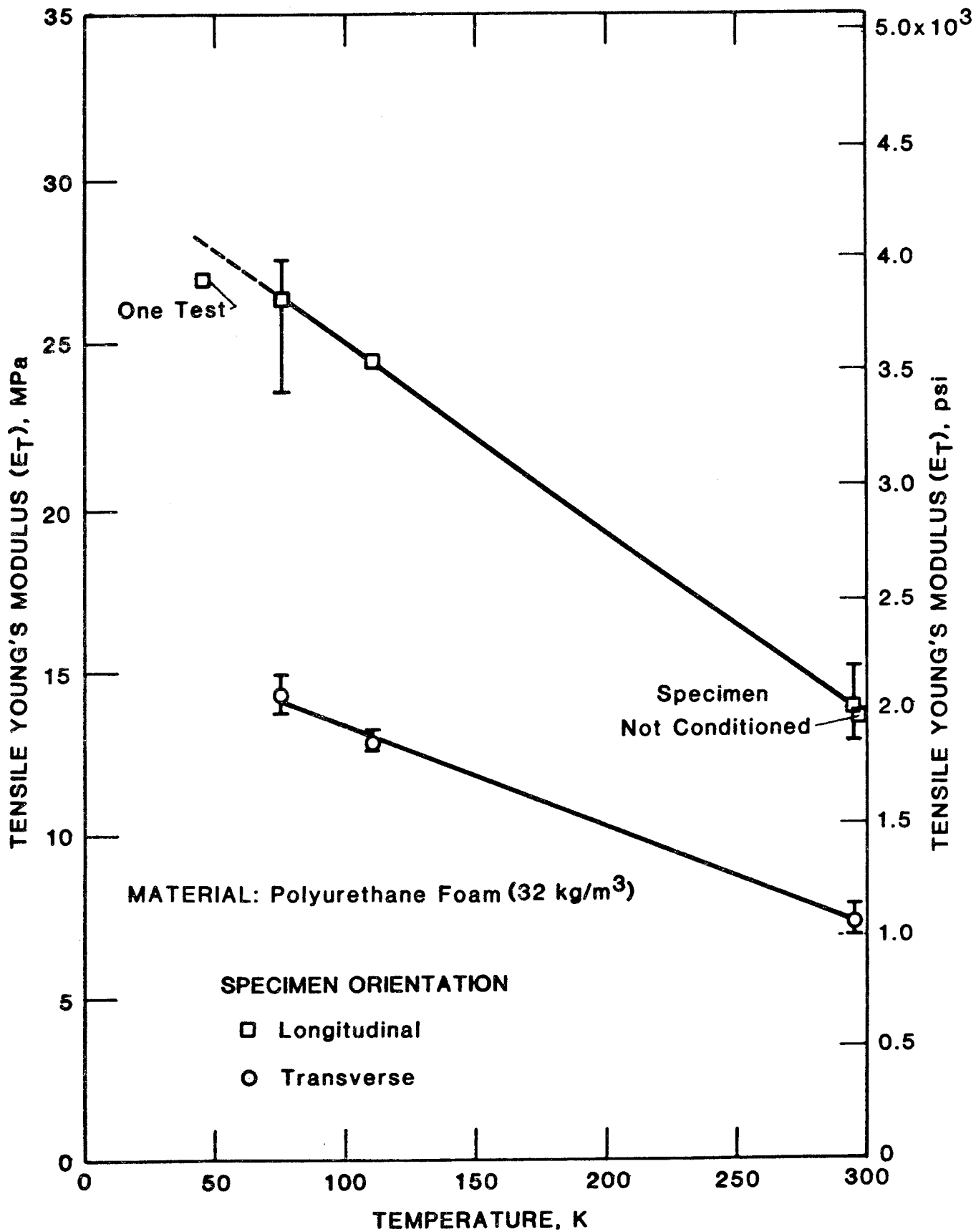
Figure 16. Tensile Young's modulus versus temperature for a 32-kg/m 3 polyurethane foam.
