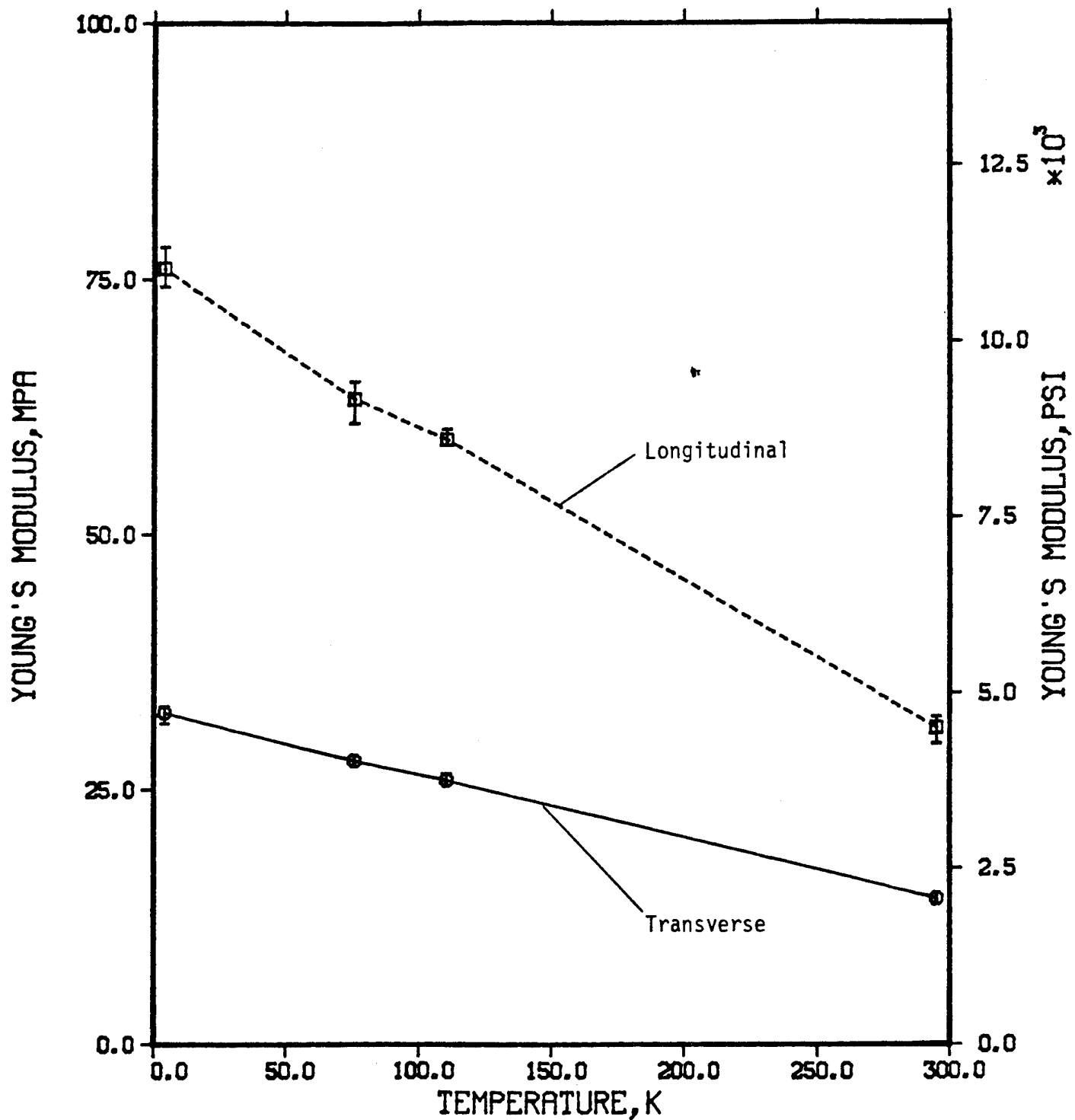
Figure 23. Tensile Young's modulus versus temperature for a 64-kg/m 3 polyurethane foam.
