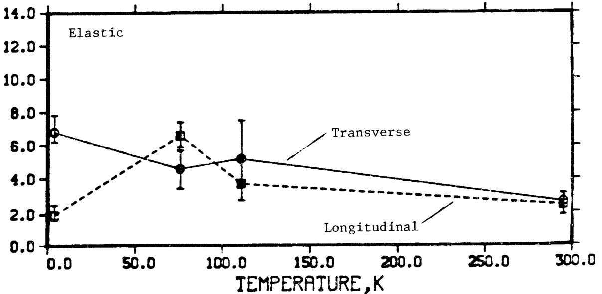
Figure 38. Compressive strain versus temperature for a 96-kg/m 3 polyurethane foam.
