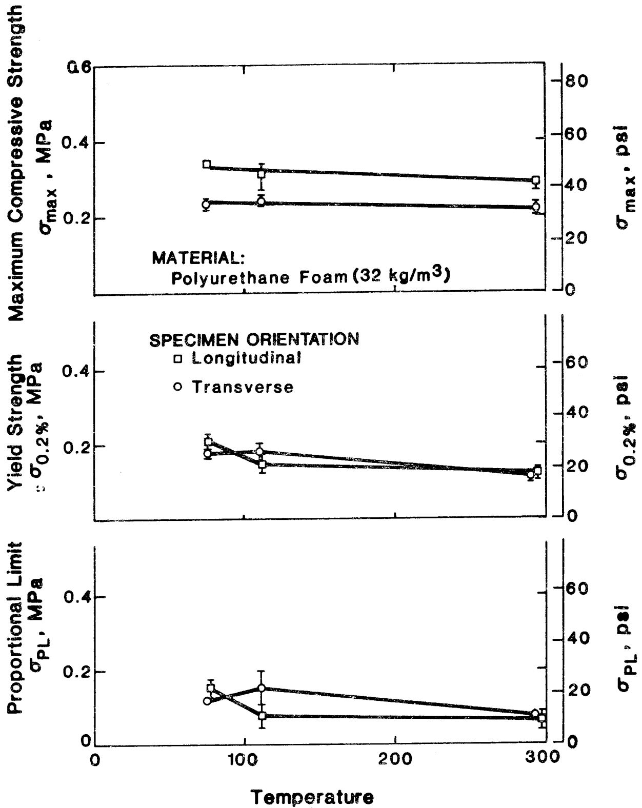
Figure 20. Compression test results: proportional limit, yield strength, and maximum compressive strength versus temperature for a 32-kg/m 3 polyurethane foam.
