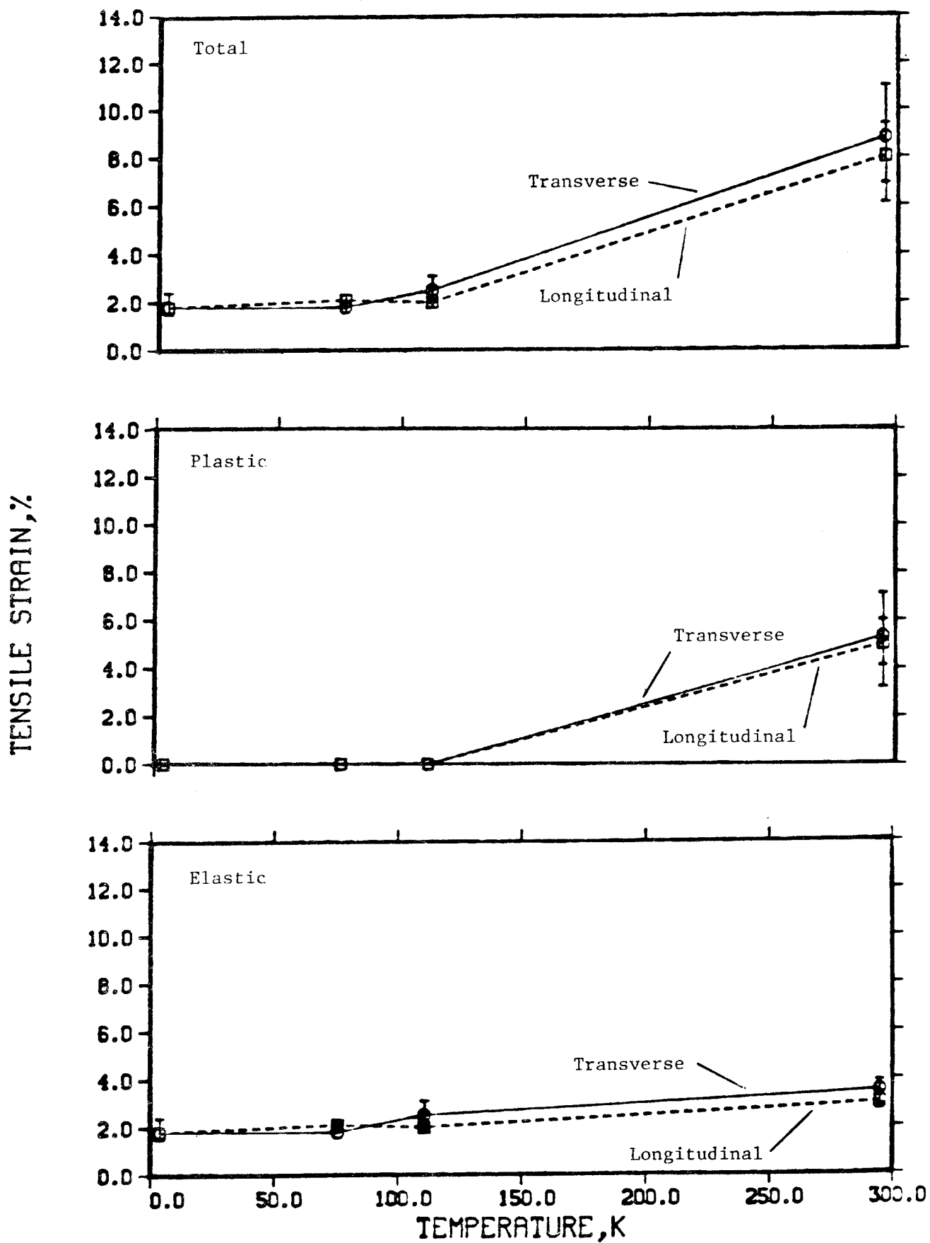
Figure 32. Tensile strain versus temperature for a 96-kg/m 3 polyurethane foam.
