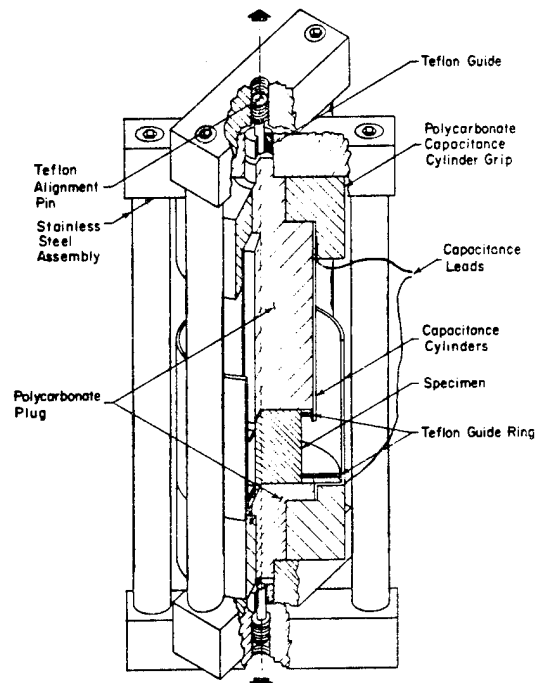
Compressive
