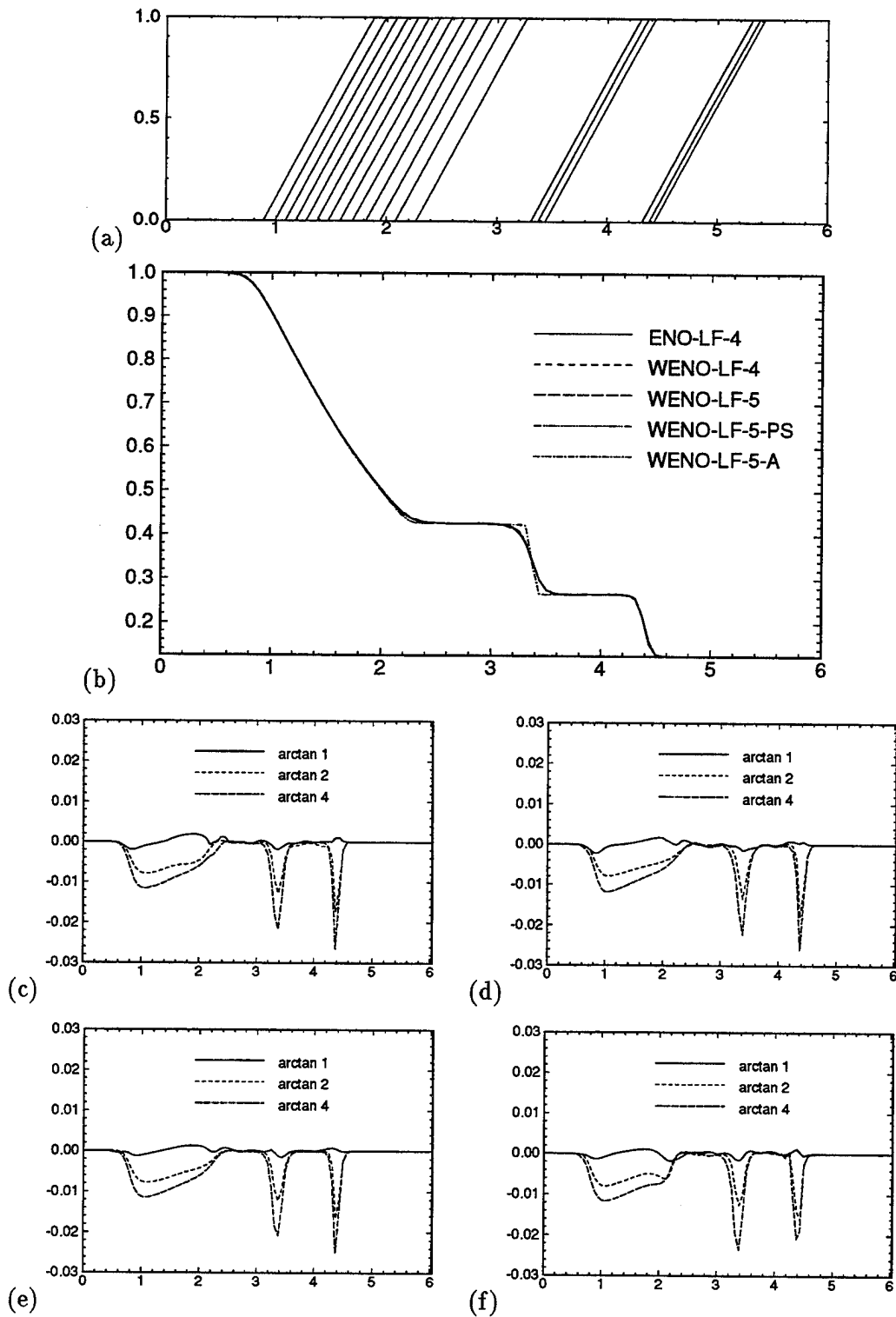
Figure 9: Oblique Sod's problem. (a) Density contours. WENO-LF-5-PS, \theta = \arctan 1 . (b) Density, y = 0 , \theta = \arctan 1 . (c)-(f) \rho_\theta - \rho_{1D} , y = 0 . (c) ENO-LF-4. (d) WENO-LF-4. (e) WENO-LF-5. (f) WENO-LF-5-PS.
