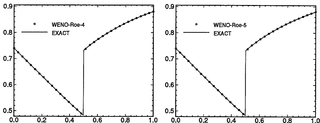
Figure 8: Density. Steady quasi-1D nozzle flow. 34 points. RK-3 in time.
