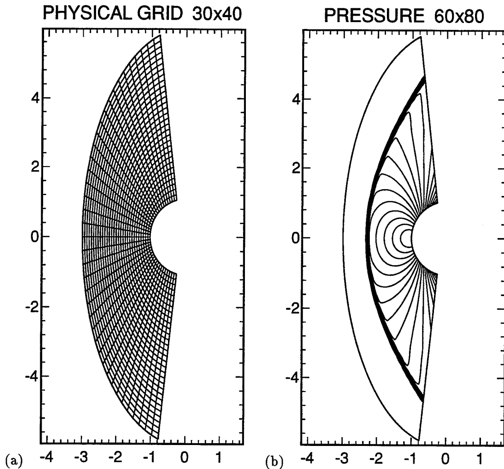
Figure 16: Flow past a cylinder. (a) Physical grid. (b) Pressure. WENO-LF-5 with RK-4. 20 contours
