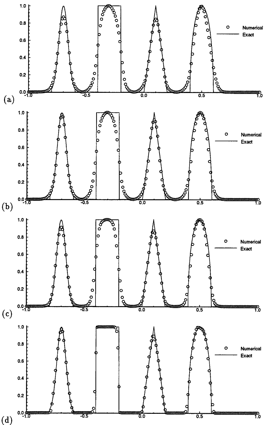
Figure 2: Linear Equation. 3rd order Runge-Kutta in time. 200 points, CFL=0.4 (0.2 for (d) only), T=8 . (a) ENO-Roe-4. (b) WENO-Roe-4. (c) WENO-Roe-5. (d) WENO-Roe-5-A.
