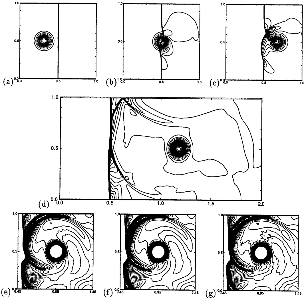
Figure 15: 2D shock vortex interaction. Pressure. (a)-(d) WENO-LF-5-PS. 30 contours. (a) t=0.05 . (b) t=0.20 . (c) t=0.35 . (d) t=0.80 . (e)-(g) t=0.60 . 90 contours from 1.19 to 1.37. (e) WENO-LF-5-PS. (f) WENO-LF-5. (g) ENO-LF-4.
