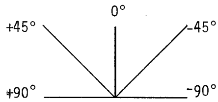
Figure 4. Top View of the Four Strips of Tape in a 45^\circ Lamina in the Group B Panels
