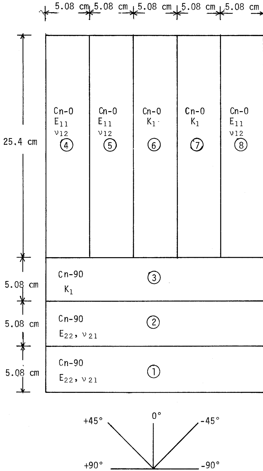
Figure 2. Coupon Designation for Panels in Groups C and D
