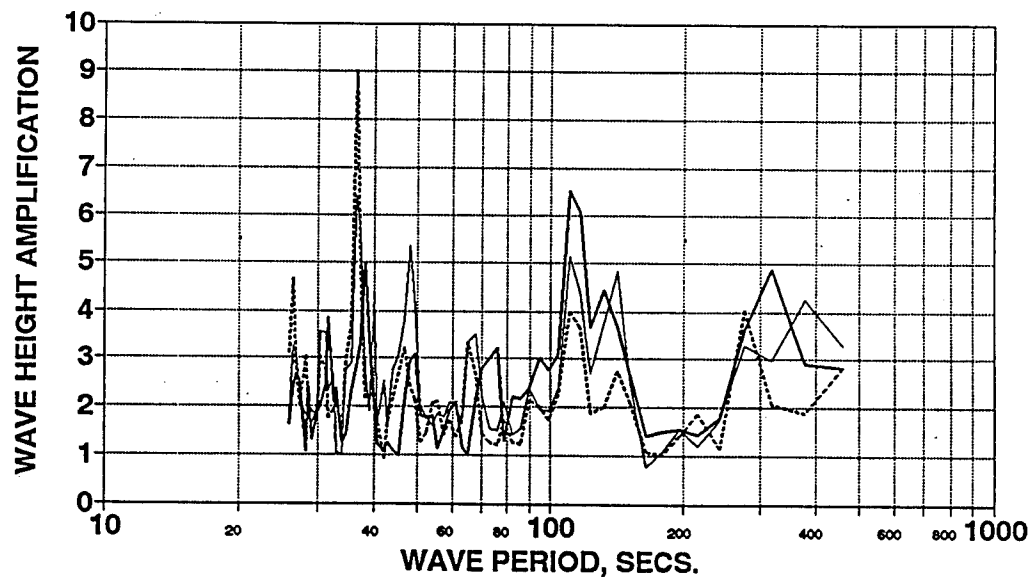
JANUARY AMPLIFICATION SPECTRUM GAGE 55
