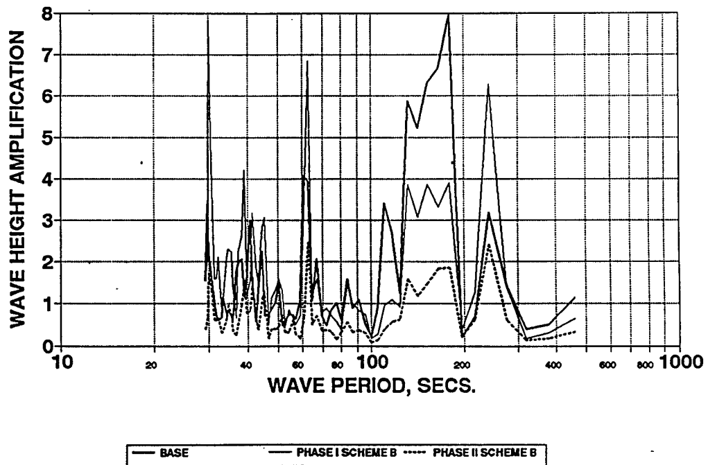
JANUARY AMPLIFICATION SPECTRUM GAGE 32 - CABRILLO BASIN
