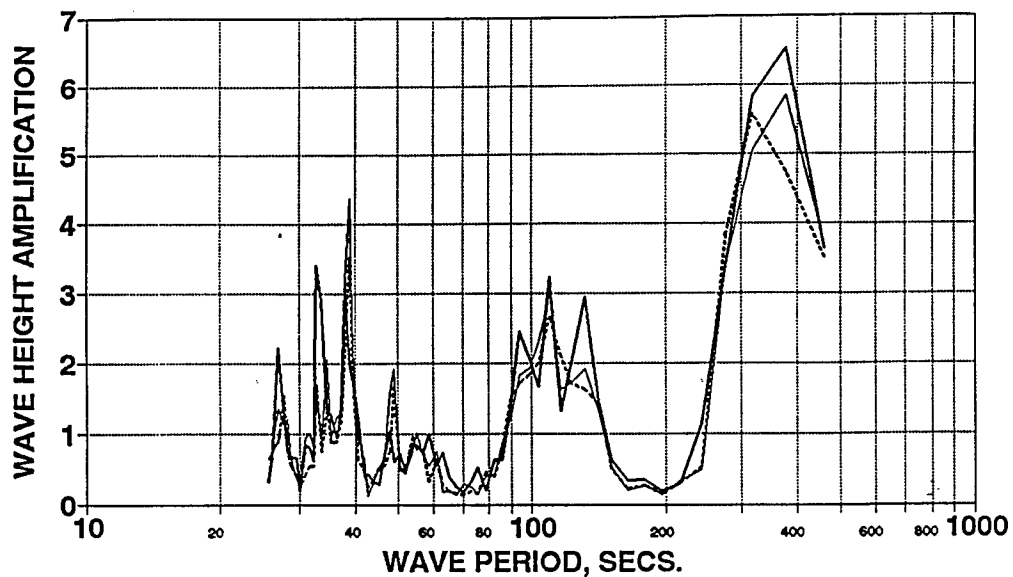
JANUARY AMPLIFICATION SPECTRUM GAGE 54
