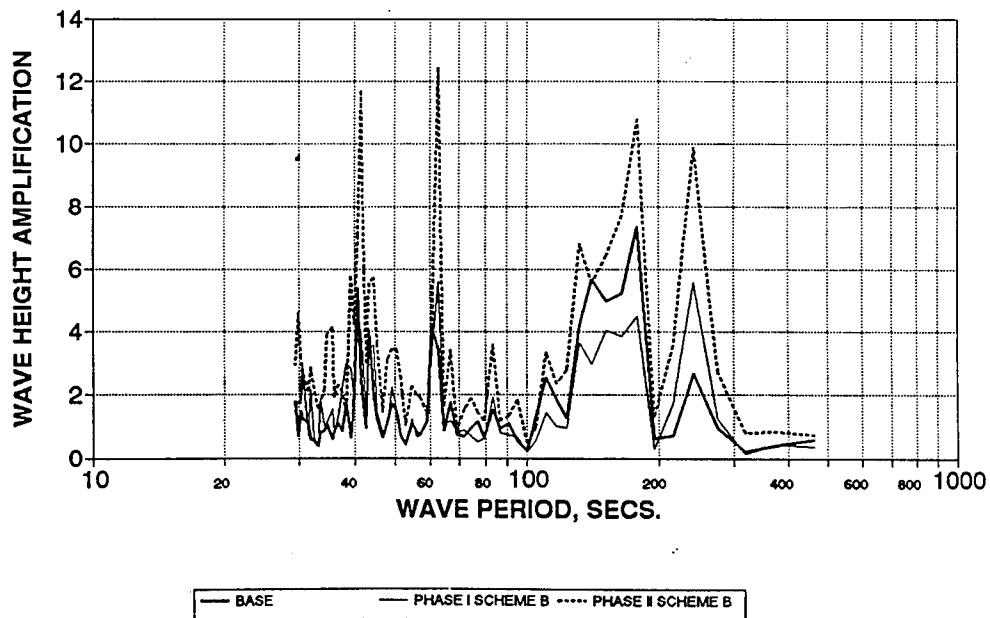
FEBRUARY AMPLIFICATION SPECTRUM GAGE 32 - CABRILLO BASIN
