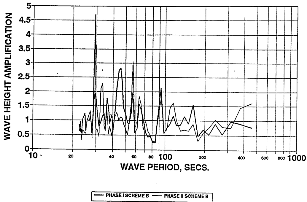
JANUARY AMPLIFICATION SPECTRUM GAGE 62
