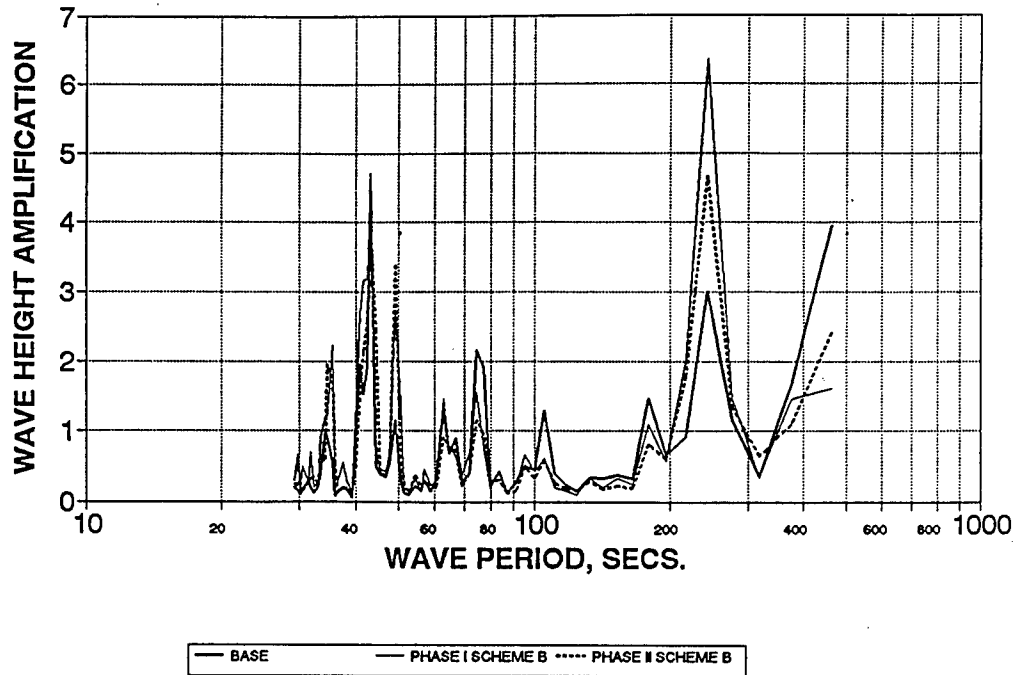
FEBRUARY AMPLIFICATION SPECTRUM GAGE 31-LA WEST CH NORTH SML BOAT BASIN
